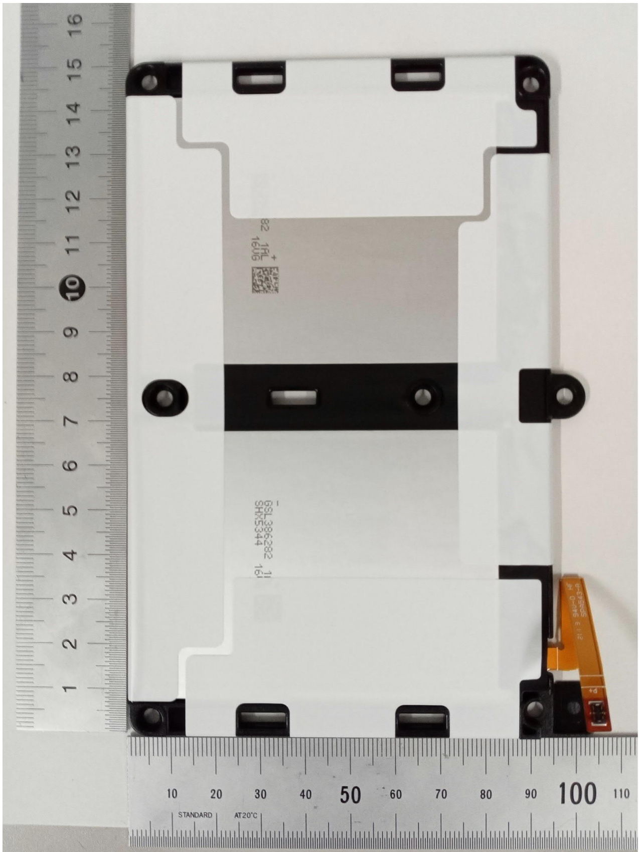
Battery Rear
