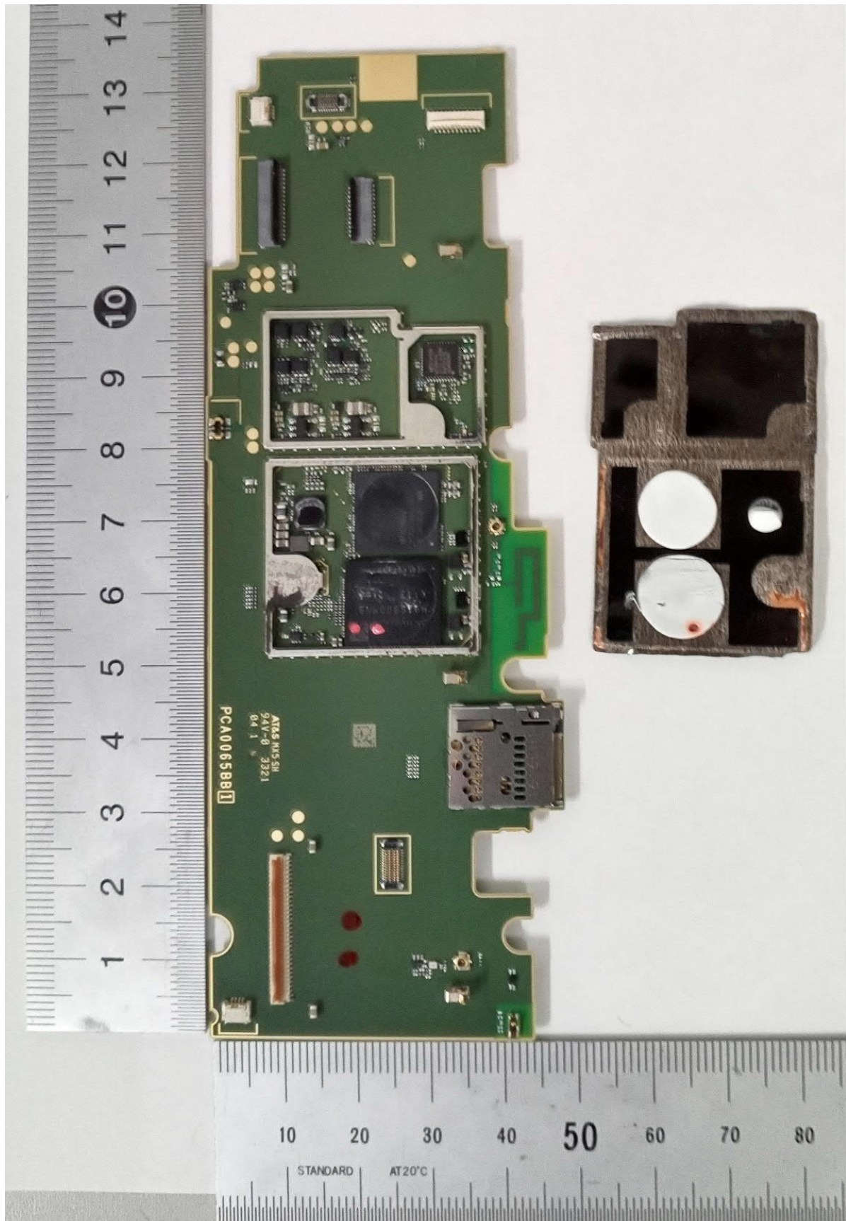
Main PCB Front Open
