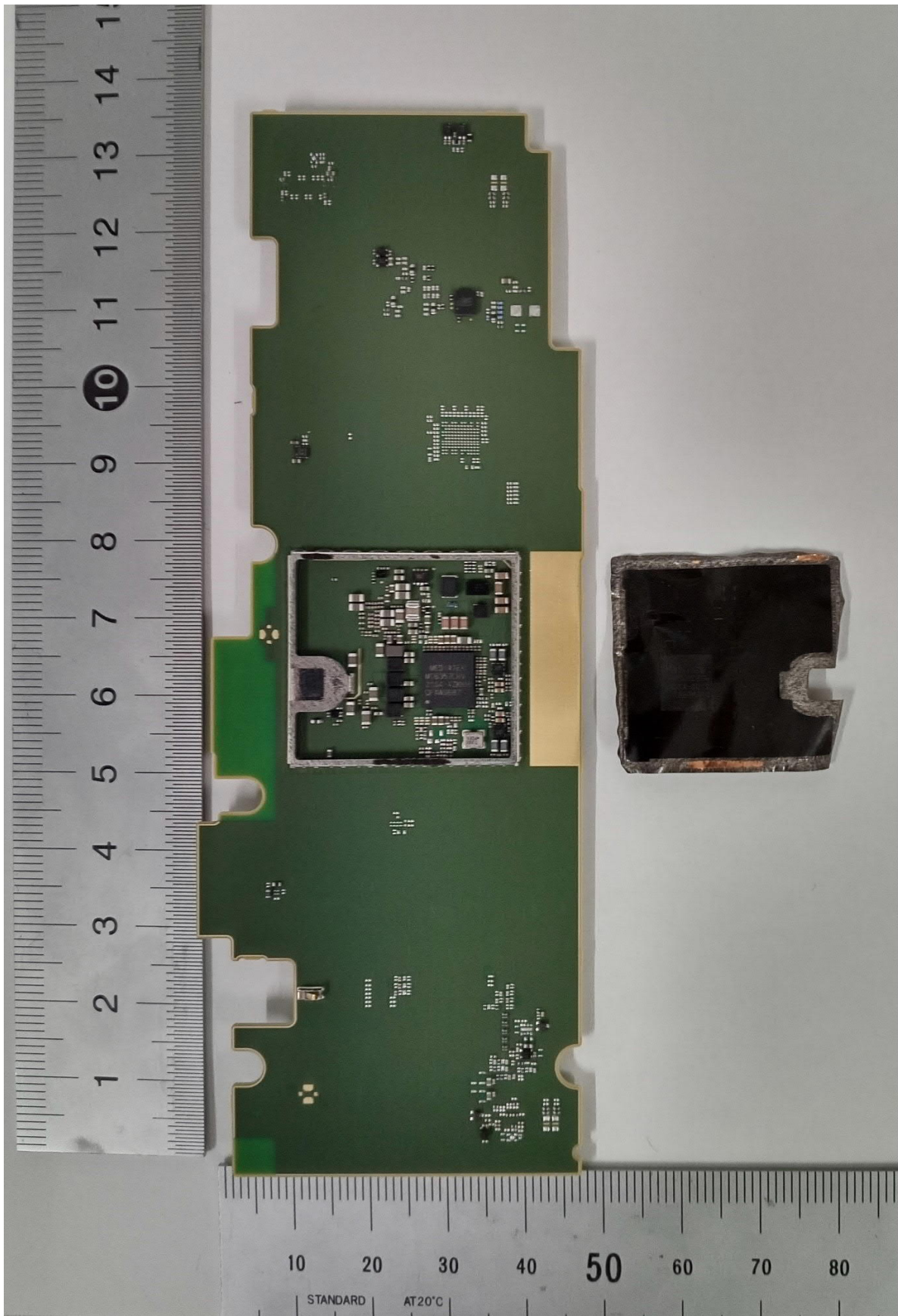
Main PCB Rear Open
