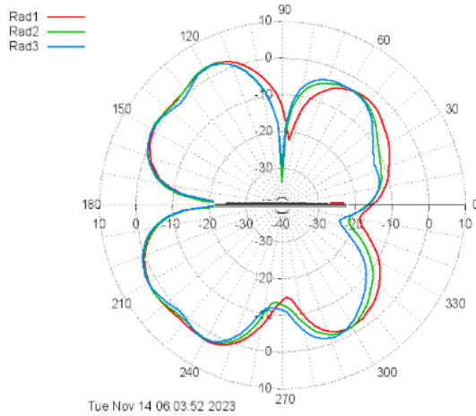
Rad #1: Tairua CR_RadPatt_murata_4_CH05-XZ plane-TX-AnH_3_CORR Rad #2: Tairua CR_RadPatt_murata_4_CH44-XZ plane-TX-AnH_0_CORR Rad #3: Tairua CR_RadPatt_murata_4_CH74-XZ plane-TX-AnH_0_CORR
