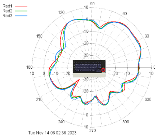
Rad #1: Tairua CR_RadPatt_murata_4_CH05-XY plane-TX-AnH_0_CORR Rad #2: Tairua CR_RadPatt_murata_4_CH44-XY plane-TX-AnH_0_CORR Rad #3: Tairua CR_RadPatt_murata_4_CH74-XY plane-TX-AnH_0_CORR
