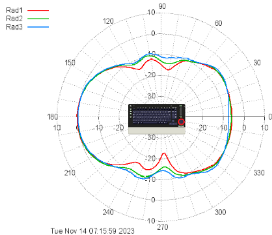
Rad #1: Tairua CR_RadPatt_murata_4_CH05-XZ plane-TX-AnV_0_CORR Rad #2: Tairua CR_RadPatt_murata_4_CH44-XZ plane-TX-AnV_0_CORR Rad #3: Tairua CR_RadPatt_murata_4_CH74-XZ plane-TX-AnV_0_CORR
