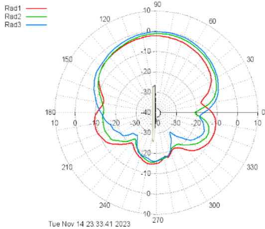
Rad #1: Tairua CR_RadPatt_murata_4_CH05-YZ plane-TX-AnV_0_CORR Rad #2: Tairua CR_RadPatt_murata_4_CH44-YZ plane-TX-AnV_0_CORR Rad #3: Tairua CR_RadPatt_murata_4_CH74-YZ plane-TX-AnV_1_CORR
