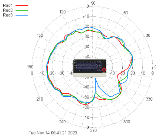
Rad #1: Tairua CR_RadPatt_murata_4_CH05-XY plane-TX-AnV_0_CORR Rad #2: Tairua CR_RadPatt_murata_4_CH44-XY plane-TX-AnV_0_CORR Rad #3: Tairua CR_RadPatt_murata_4_CH74-XY plane-TX-AnV_0_CORR
