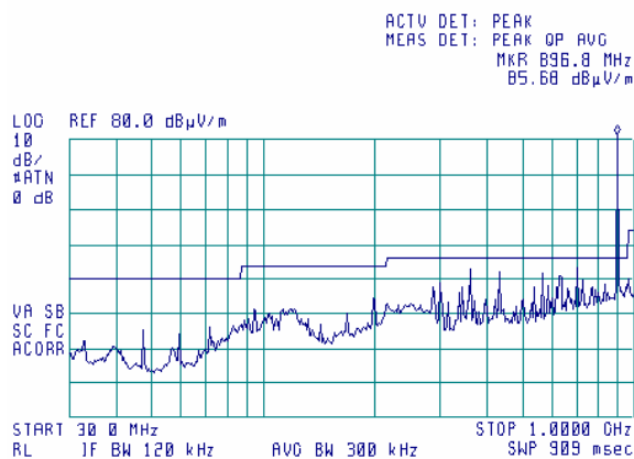
Plot 7.1.10 Radiated emission measurements from 30 to 1000 MHz
