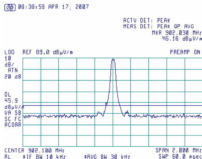
Plot 7.2.1 Lower band edge emission test result
