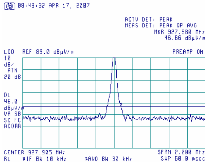
Plot 7.2.2 High b and edge emission test result
