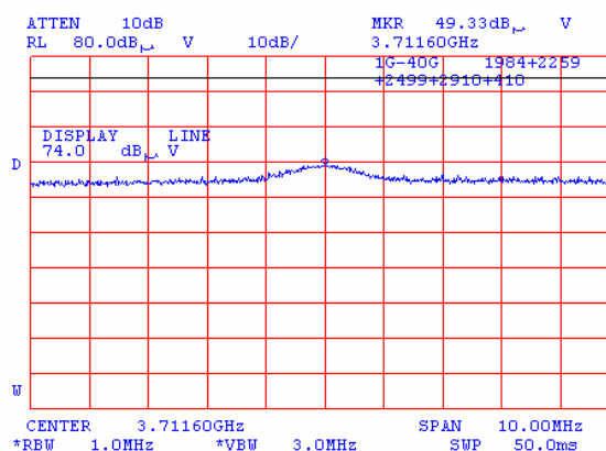
Plot 7.1.27 Radiated emission measurements at the fifth harmonic frequency
