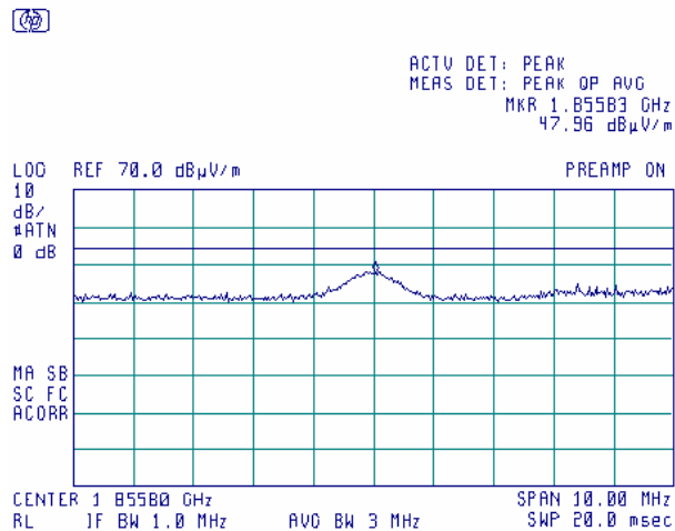
Plot 7.1.21 Radiated emission measurements at the third harmonic frequency
