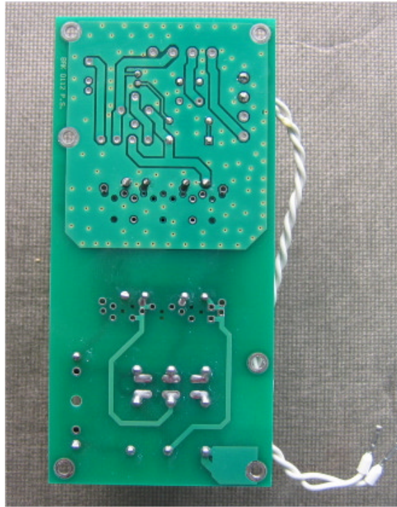
Photograph No.6 Second PCB bottom view
