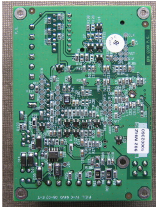
Photograph No4 Site controller main PCB front view
