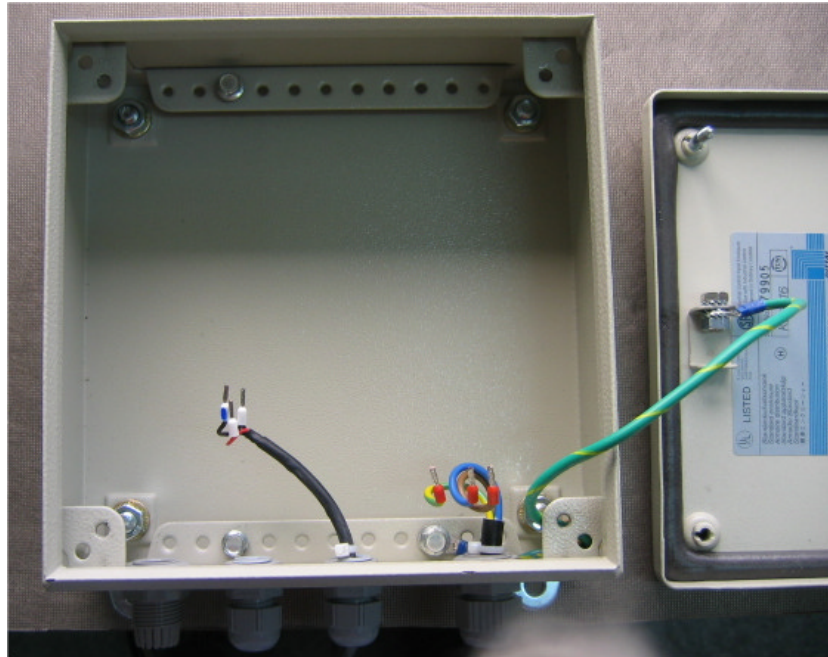
Photograph No.8 Site controller case internal view
