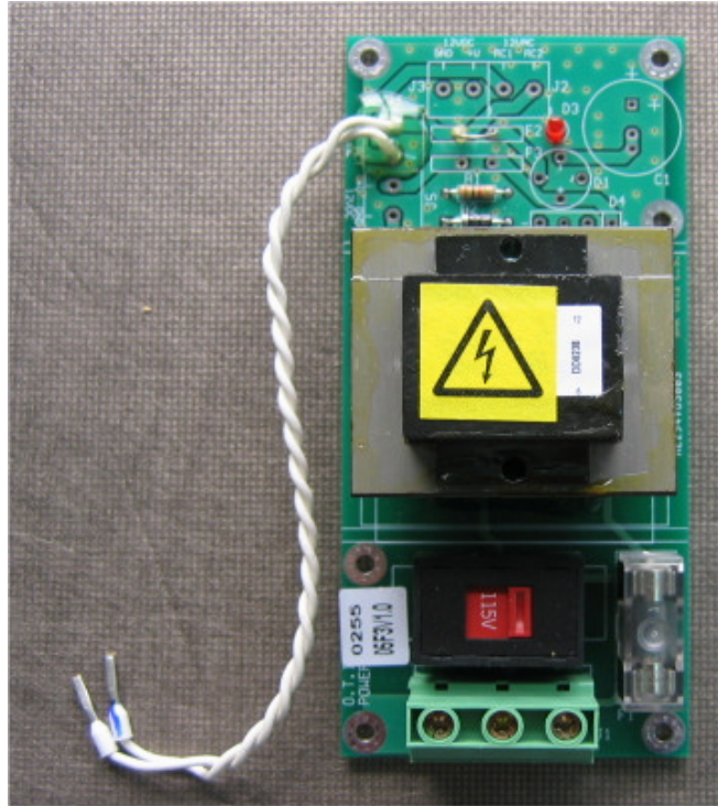
Photograph No.5 Second PCB front view
