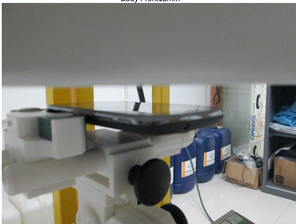
Body Front15mm
