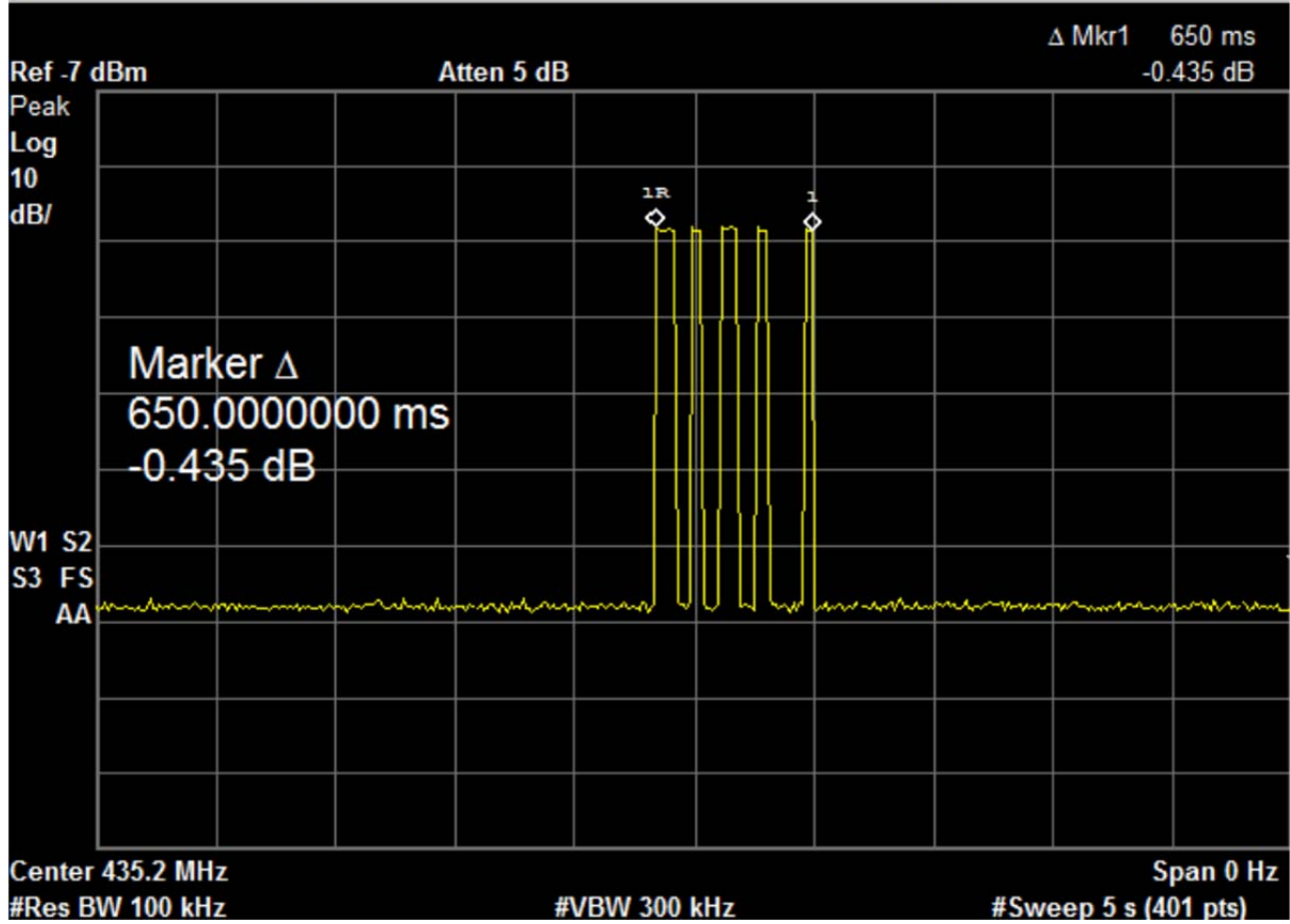
Plot 2 – Deactivation Time – Continuous Transmit Mode
