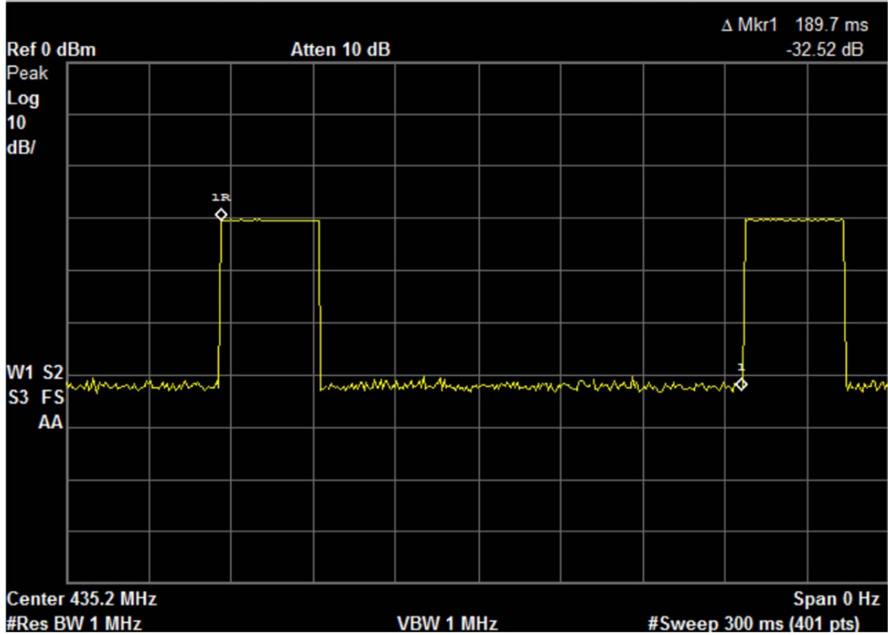
Plot 4 – Duty Cycle – Period
