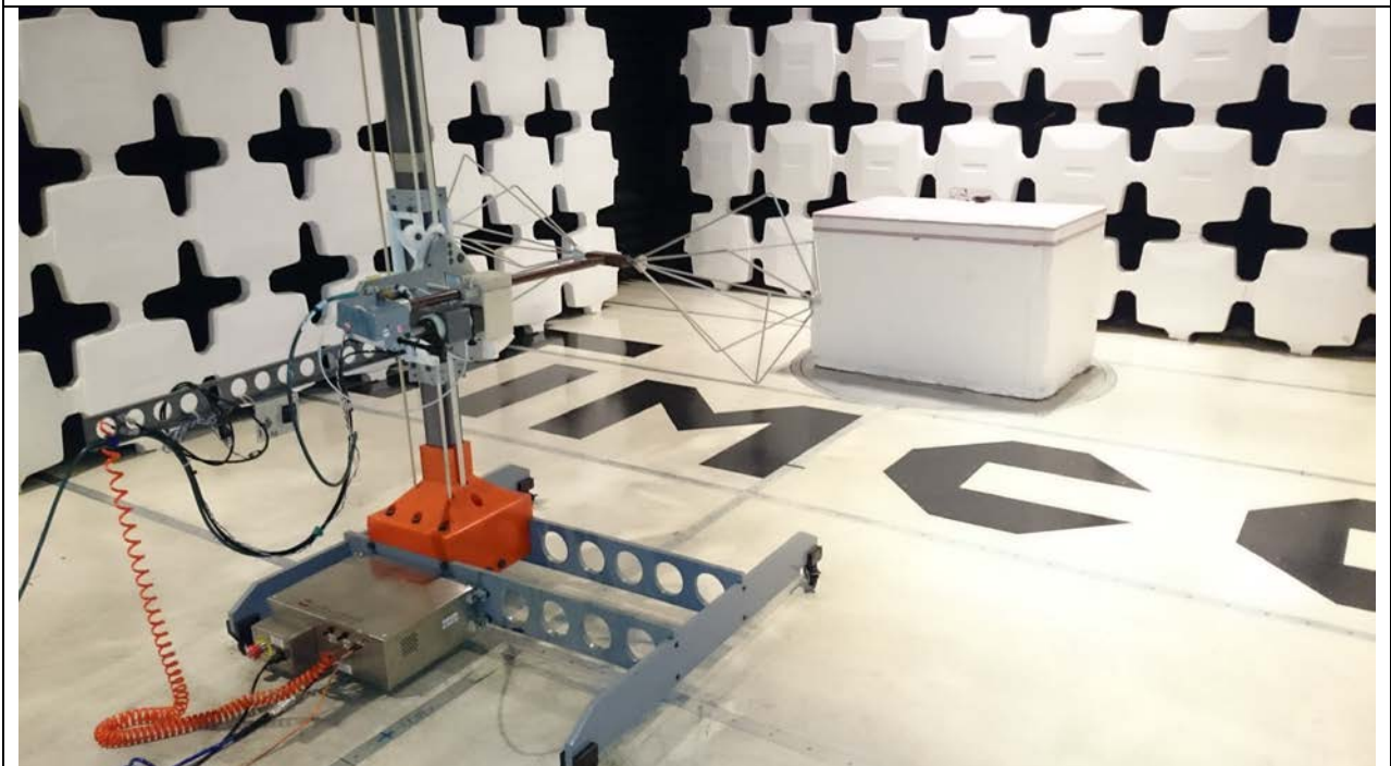
FIELD STRENGTH SPURIOUS EMISSIONS 30 – 200 MHz
