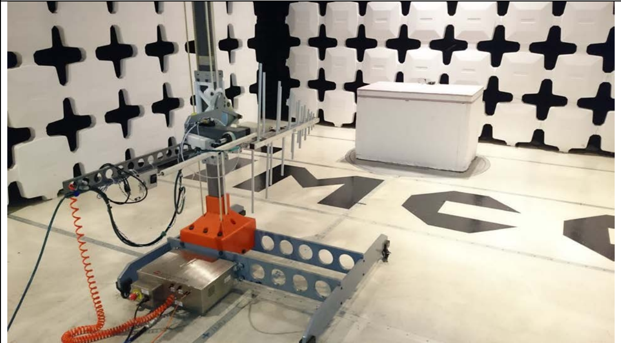
FIELD STRENGTH SPURIOUS EMISSIONS 200 MHz – 1 GHz
