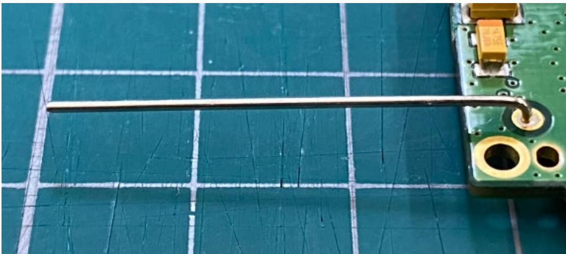
Antenna 2 (Wire Antenna)
