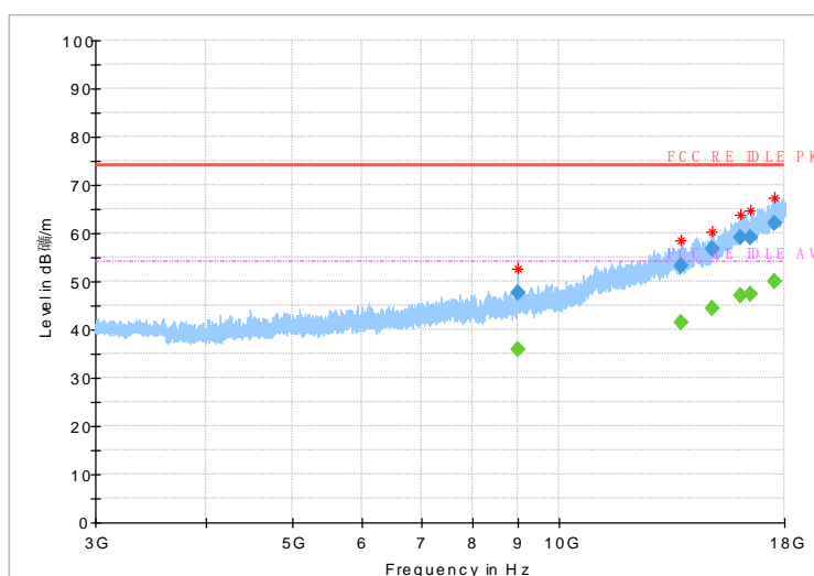
Fig.54 Radiated emission: 8DPSK, Ch0, 3GHz~18GHz
