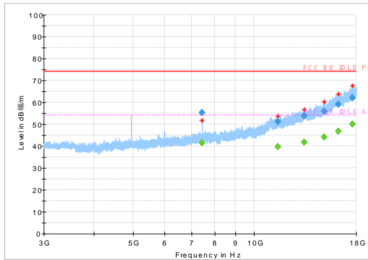
Fig.42 Radiated emission: GFSK, Ch78, 3GHz~18GHz
