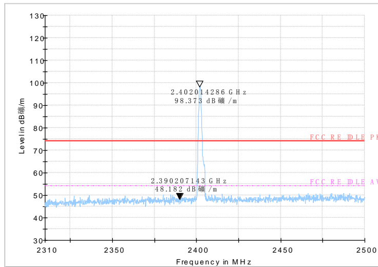
Fig.43 Radiated emission (Power): GFSK, low channel
