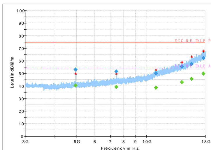
Fig.48 Radiated emission: \pi/4 DQPSK, Ch78, 3GHz~18GHz
