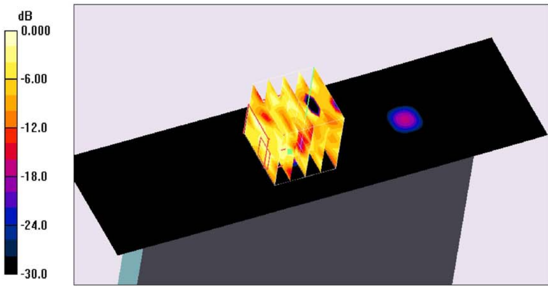
0 dB = 0.015mW/g
