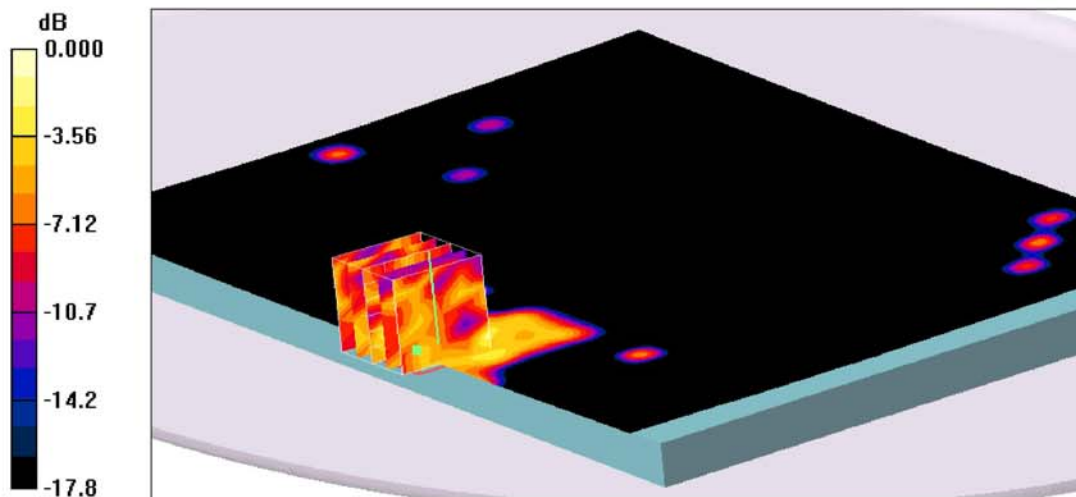
0 dB = 0.024mW/g
