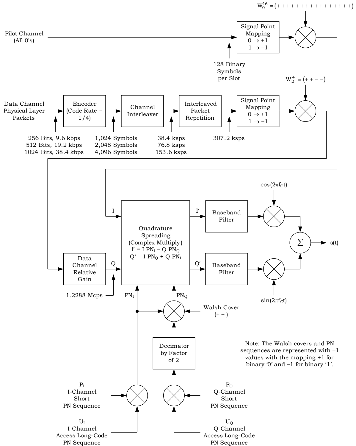
Figure 4-5 Subtype 1 Physical Layer Protocol Reverse Channel Structure for the Access Channel
