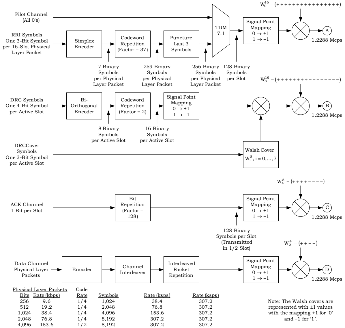
Figure 4-6 Reverse Channel Structure for the Reverse Traffic Channel (Part 1 of 2)
