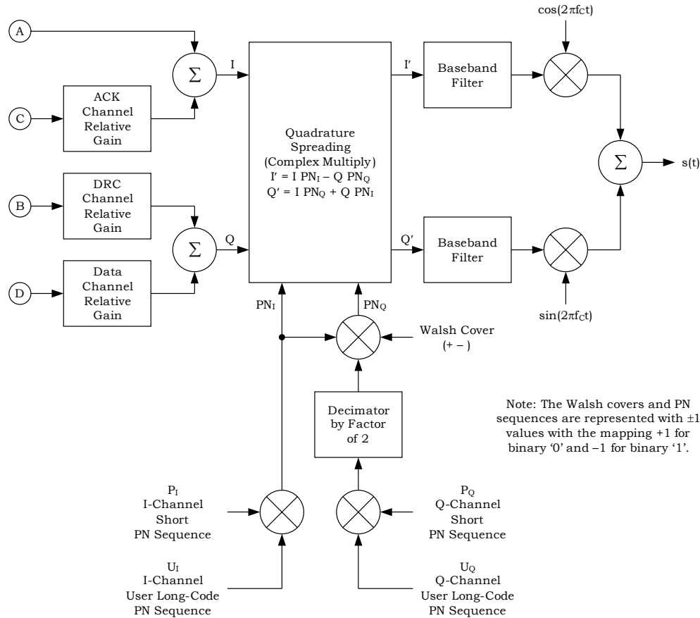
Figure 4-7 Reverse Channel Structure for the Reverse Traffic Channel (Part 2 of 2)
