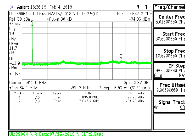
LTE B5 3MHz 16QAM Mid Channel RB1-0
