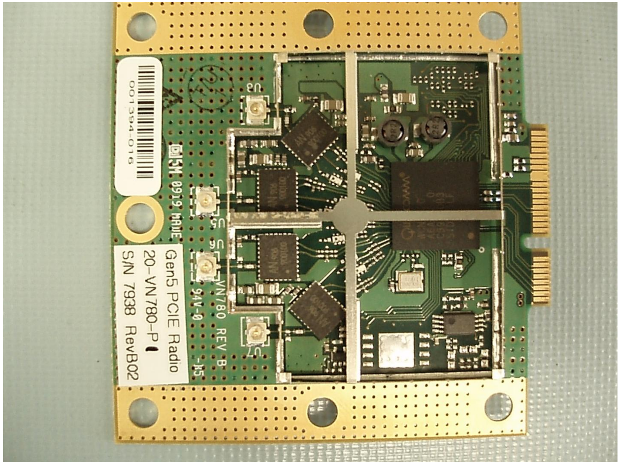
Figure 1 EA544D_1 Ethernet Adapter Card without shield
