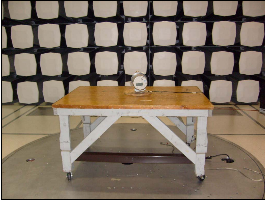
Photograph 5. Radiated Emissions, Test Setup
