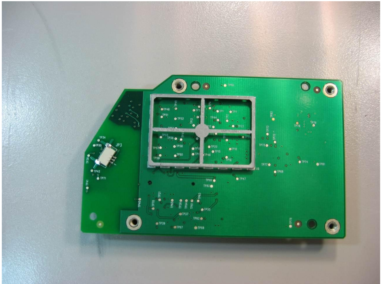
Photograph 39. 375-1371_Metering_piggyback_I0352
