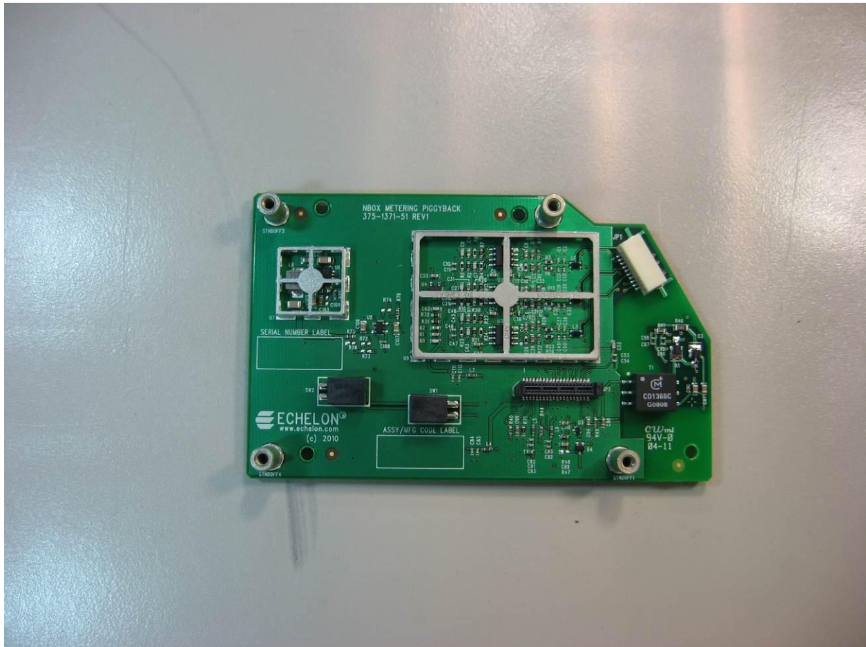
Photograph 38. 375-1371_Metering_piggyback_I0351
