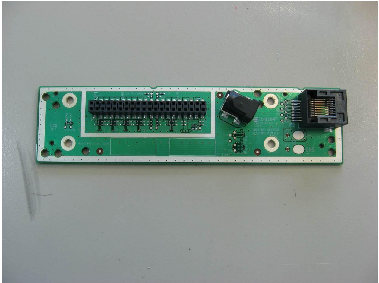
Photograph 41. 375-1371_WIFI_IFB_I0399
