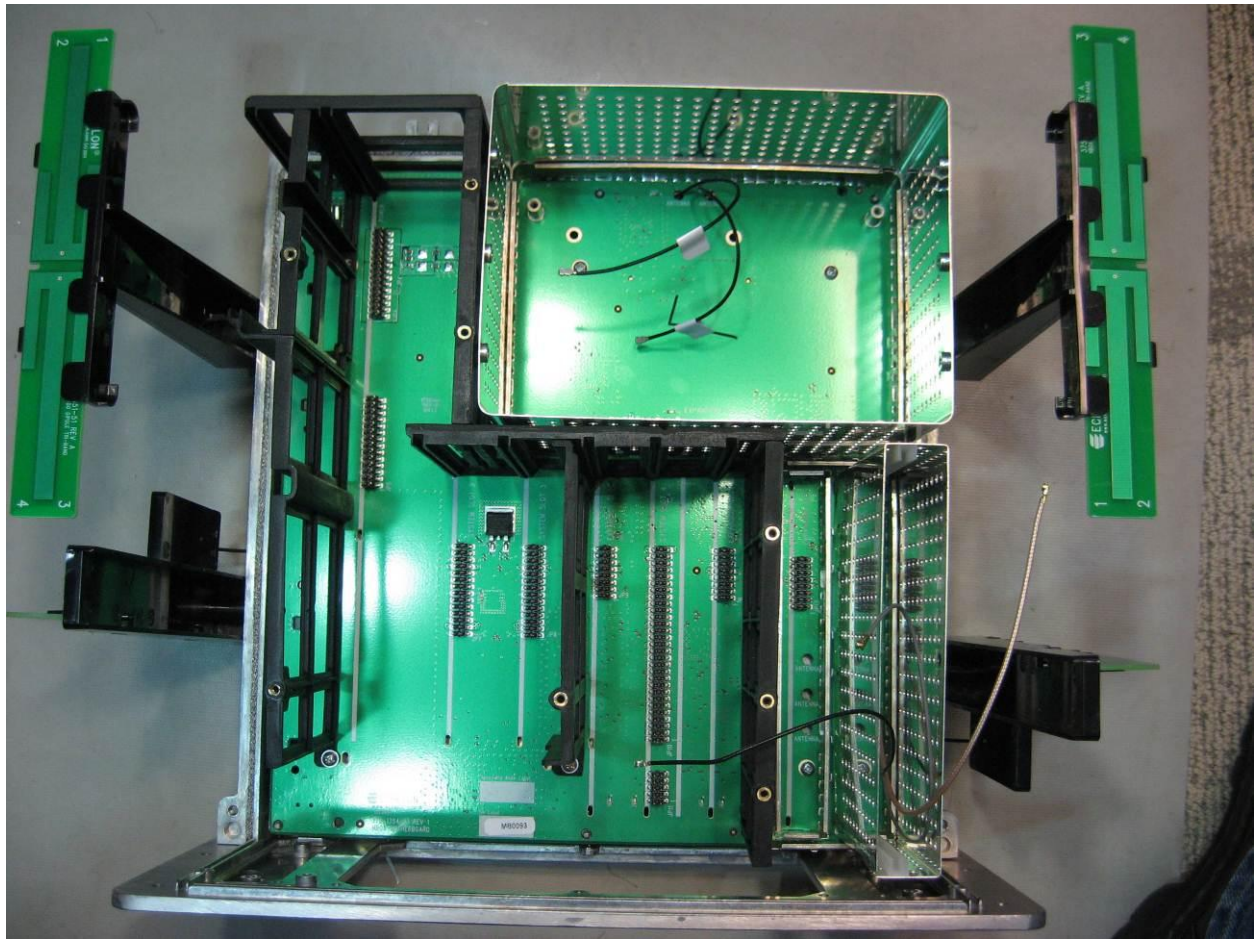
Photograph 46. ECN-70101_Chassy_Empty_0374
