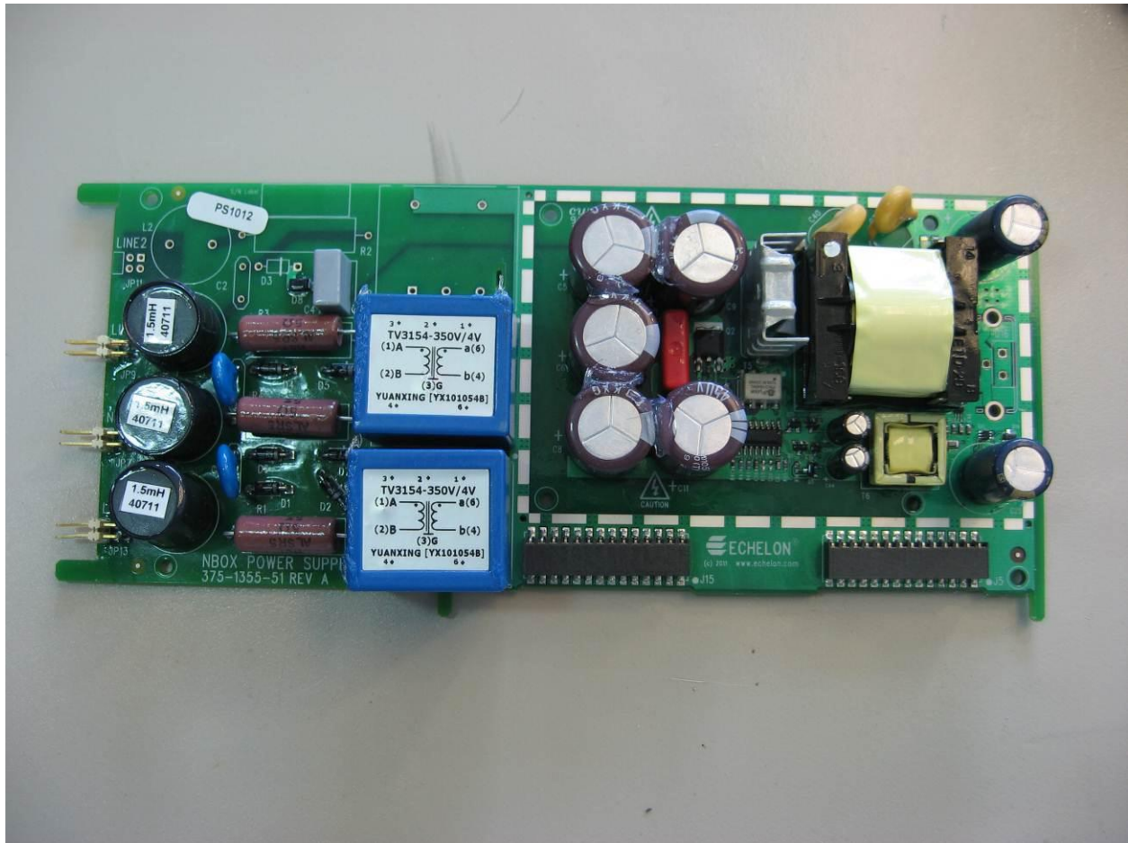
Photograph 27. 375-1355_Power_Supply_I0387
