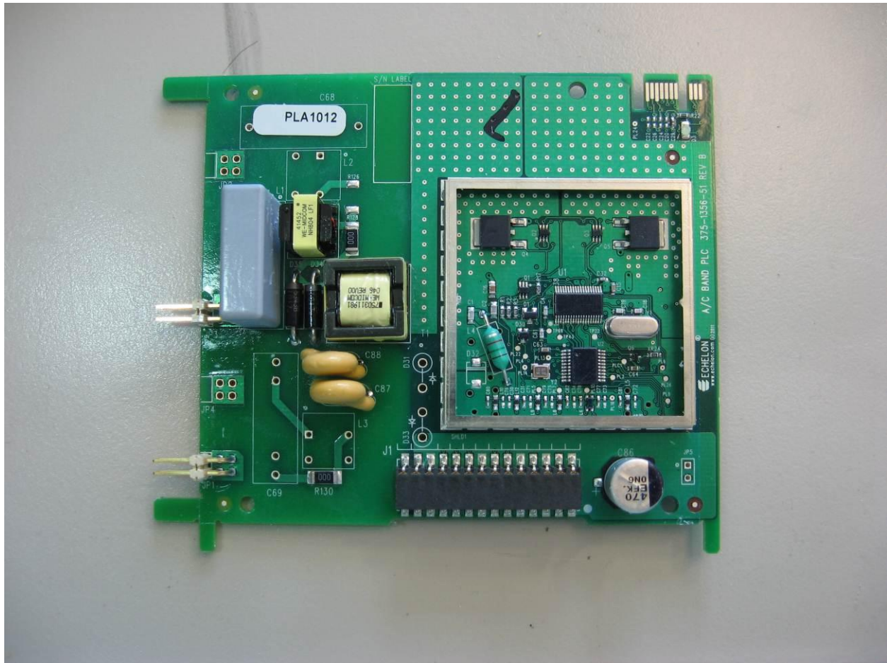
Photograph 28. 375-1356_PLC-A_I0393
