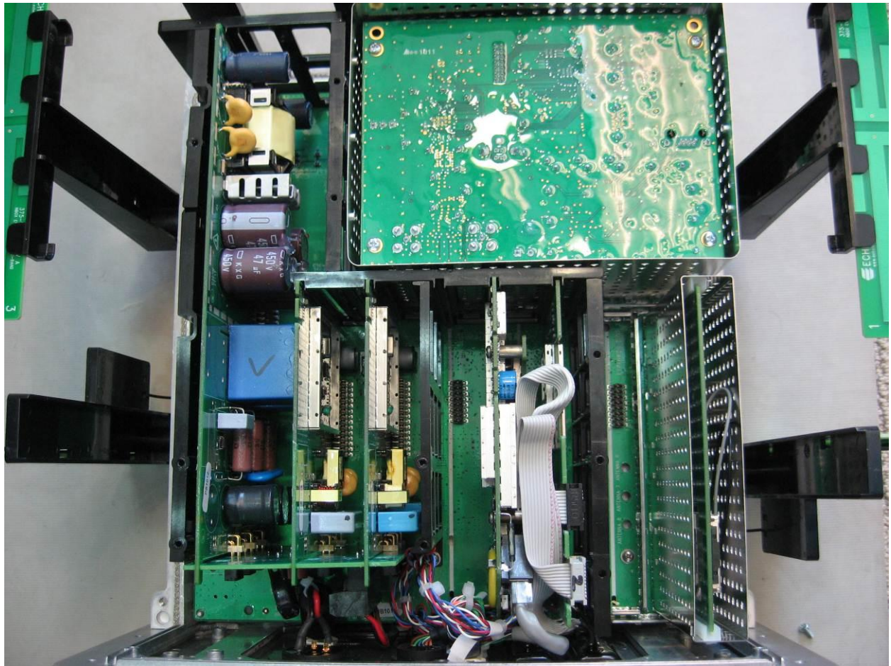
Photograph 47. 70101-R003-Top-Shield removed-I0406
