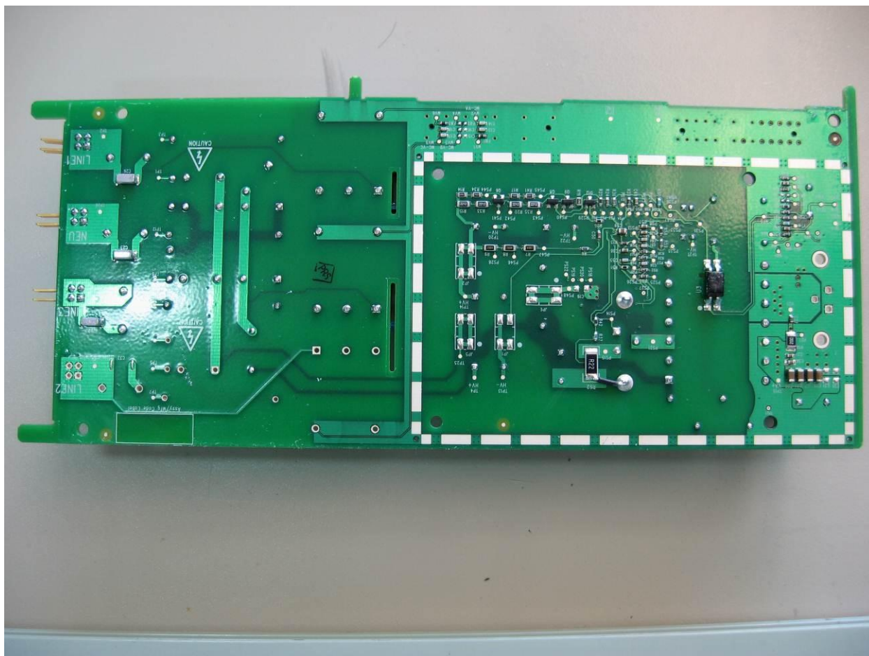
Photograph 25. 375-1355_Power_Supply_bottom_I0388
