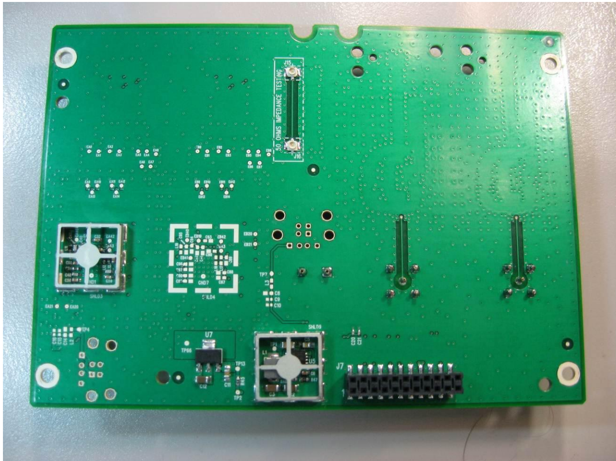
Photograph 42. 375-1394_Badger_IFB_Back_I0356
