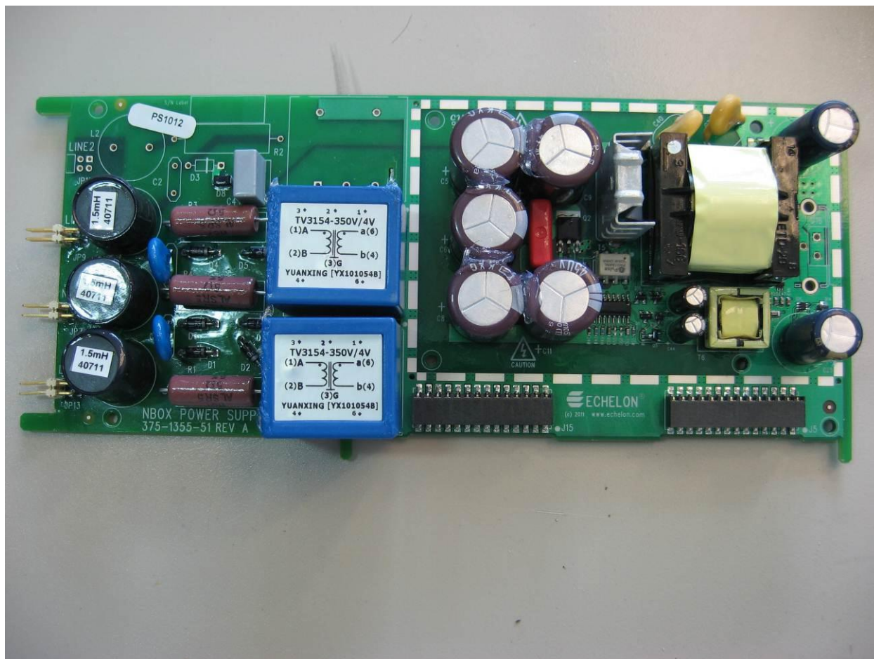
Photograph 26. 375-1355_Power_Supply_I0386
