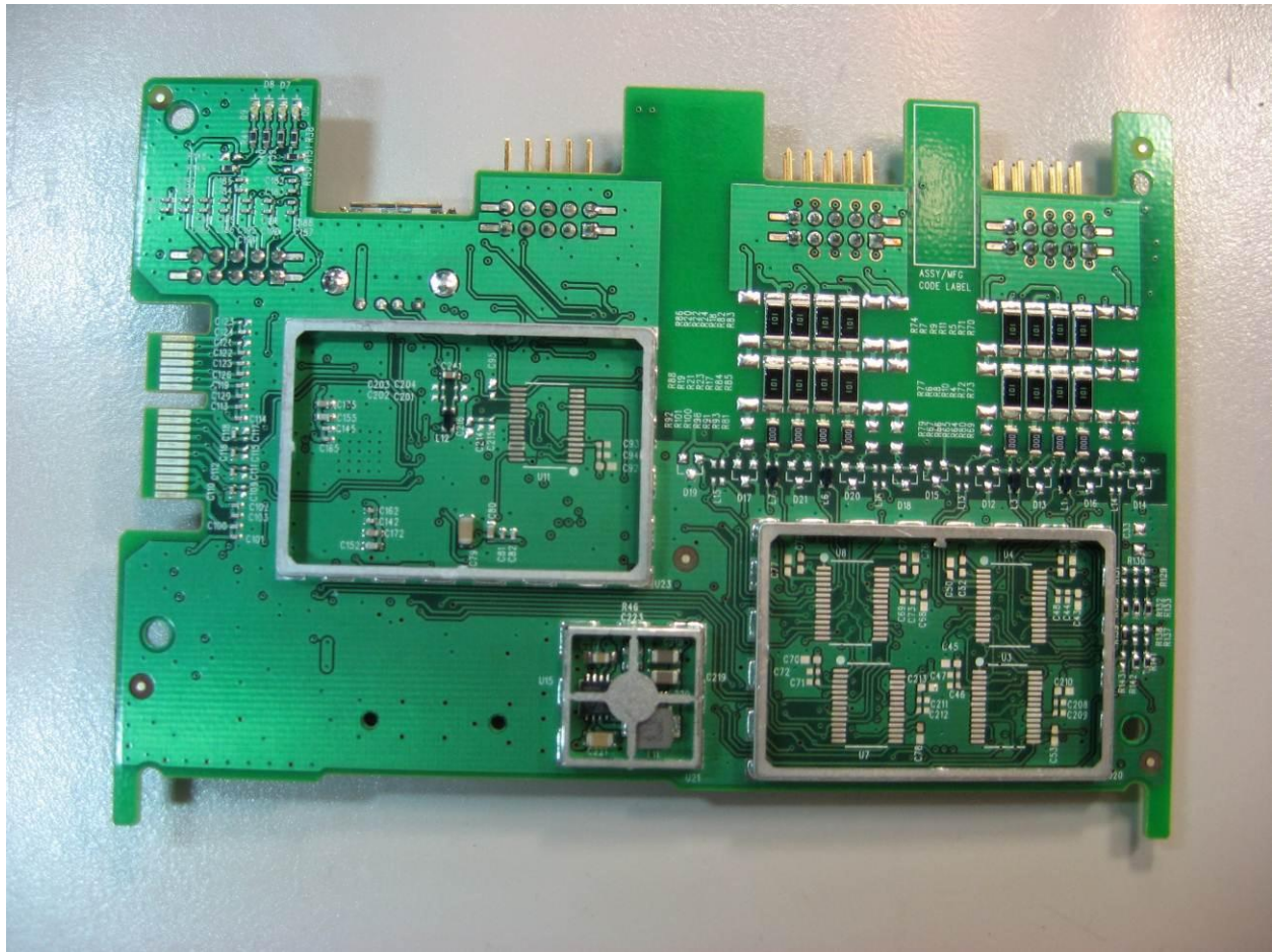
Photograph 32. 375-1358_Serial_Board_Bottom_I0342
