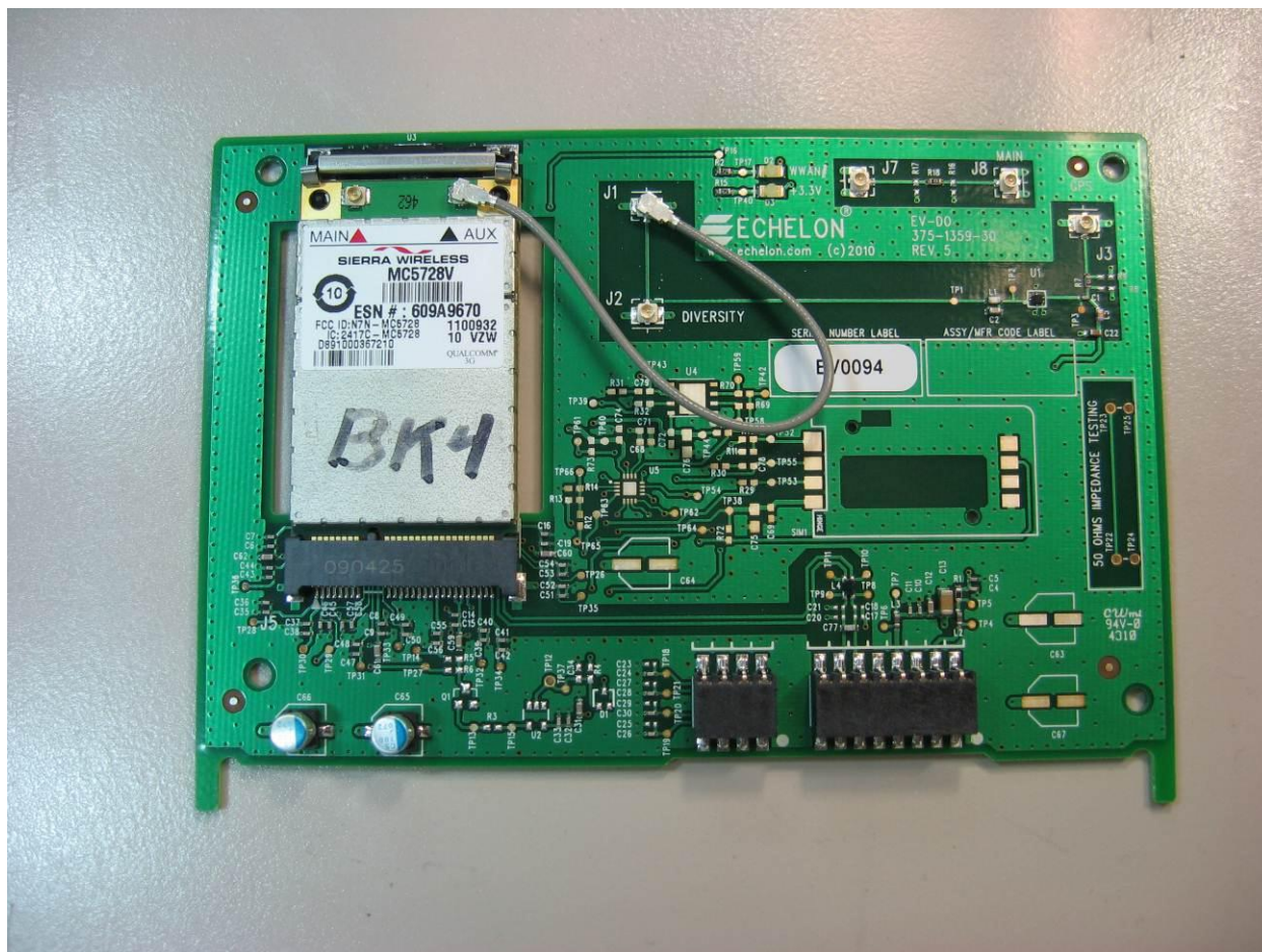
Photograph 35. 375-1359-30_EVDO_IFB_I0335
