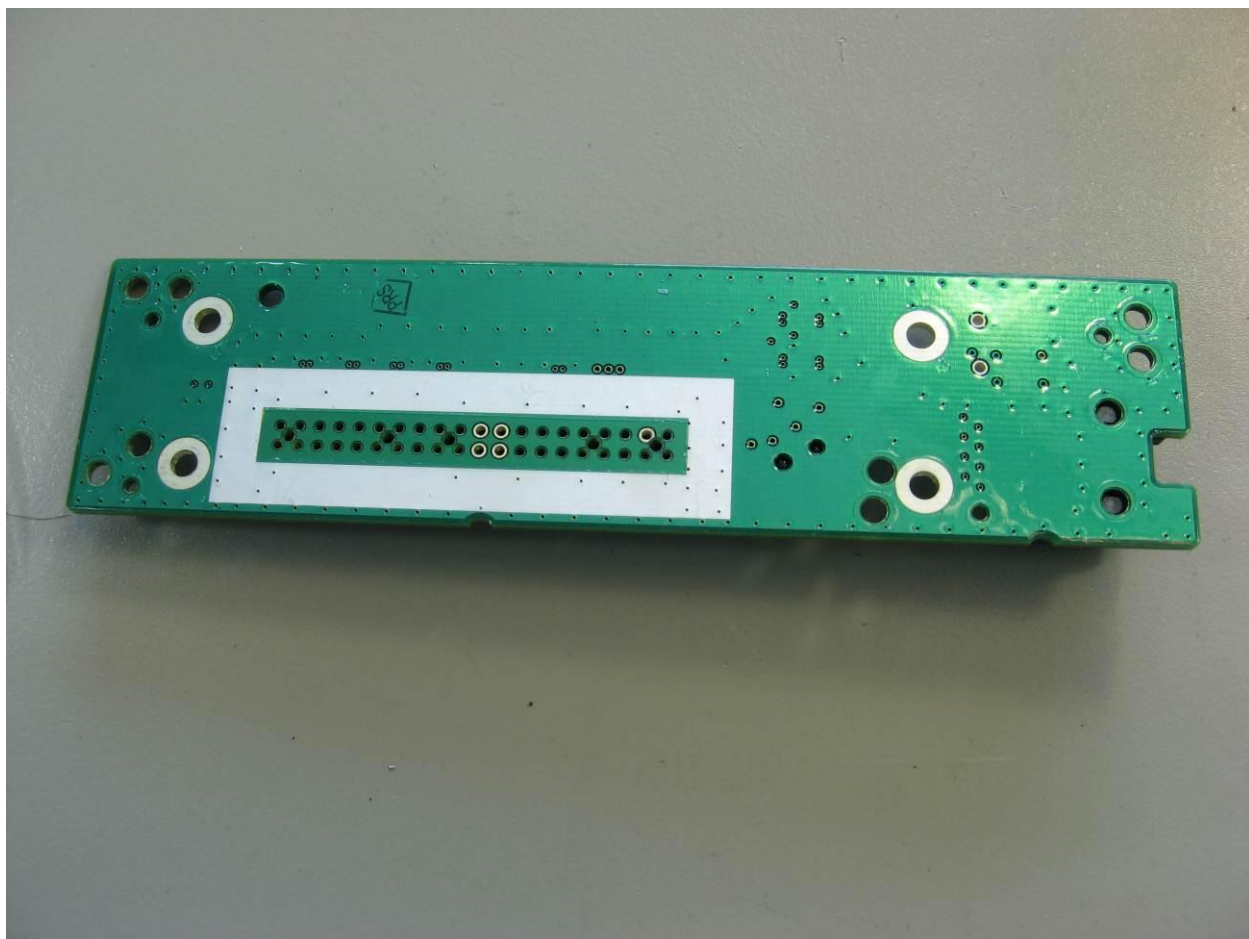
Photograph 40. 375-1371_WIFI_IFB_bottom_I0400
