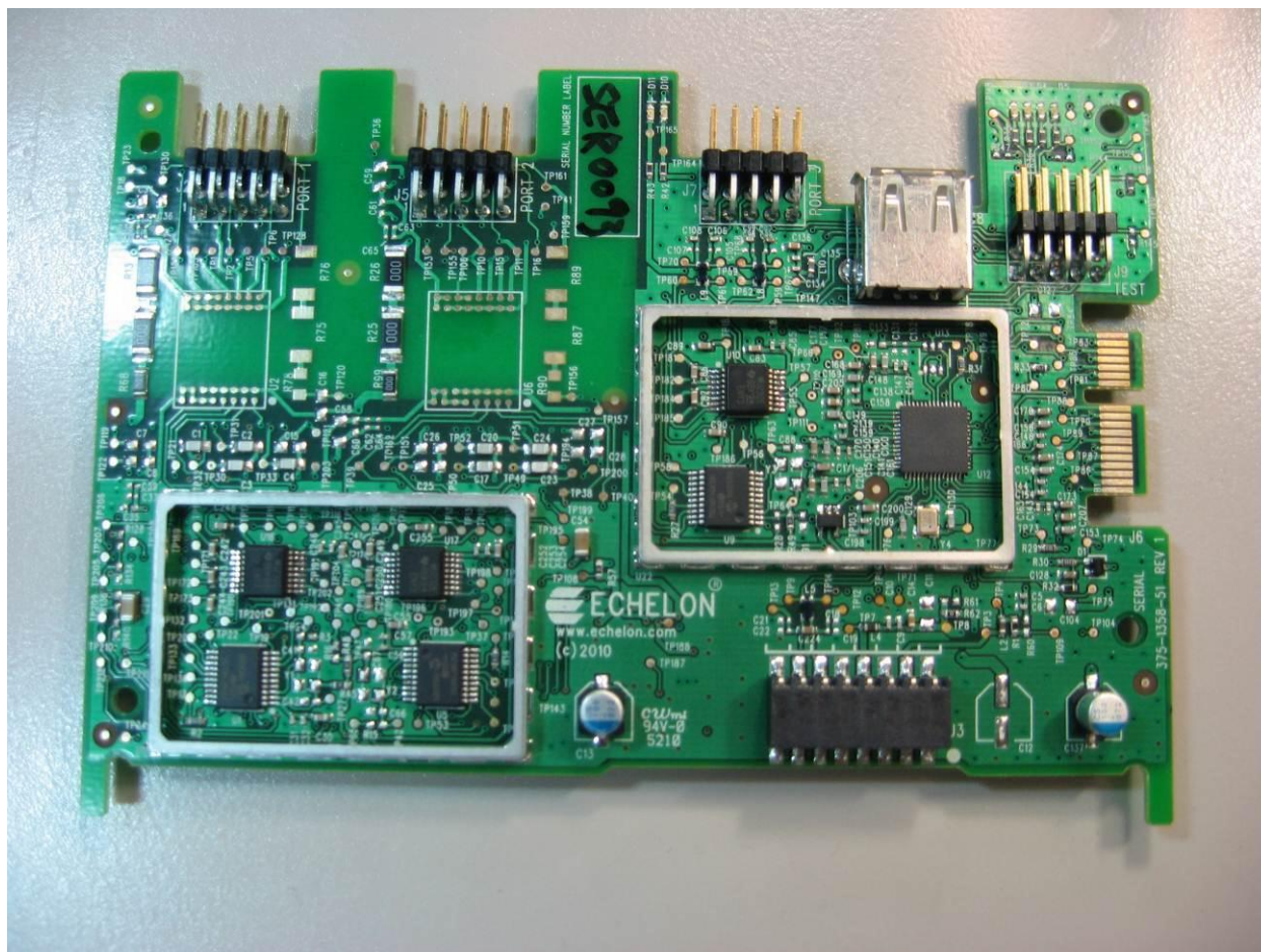
Photograph 33. 375-1358_Serial_Board_I0344
