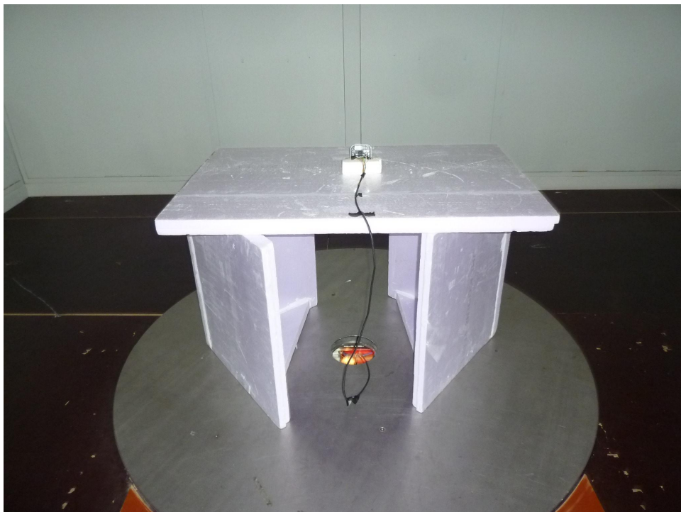
181073emi4.JPG: Final radiated emissions OATS
