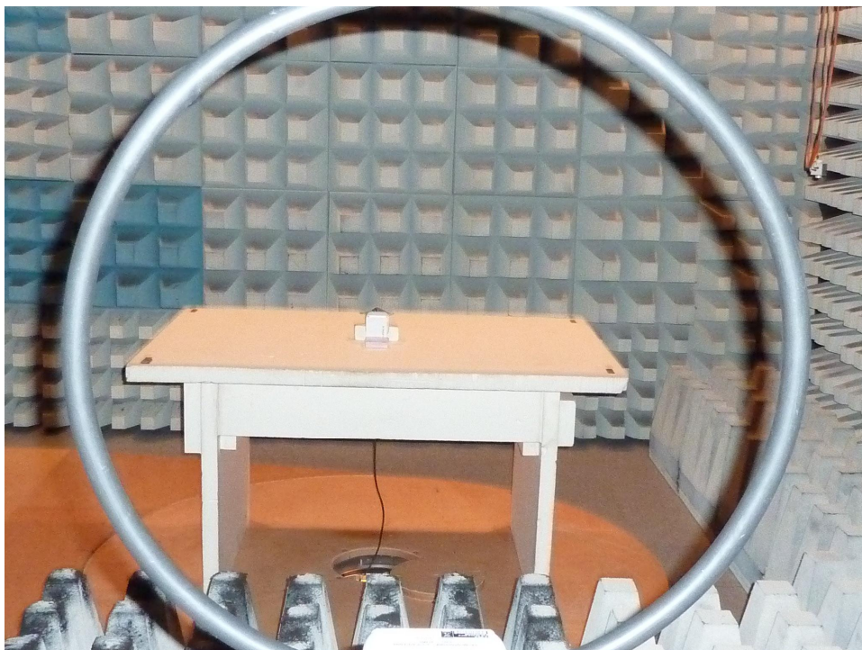
181073emi2.JPG: Radiated emissions FAR < 30 MHz
