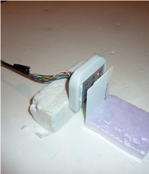
181073emi1.JPG: Radiated emissions FAR
