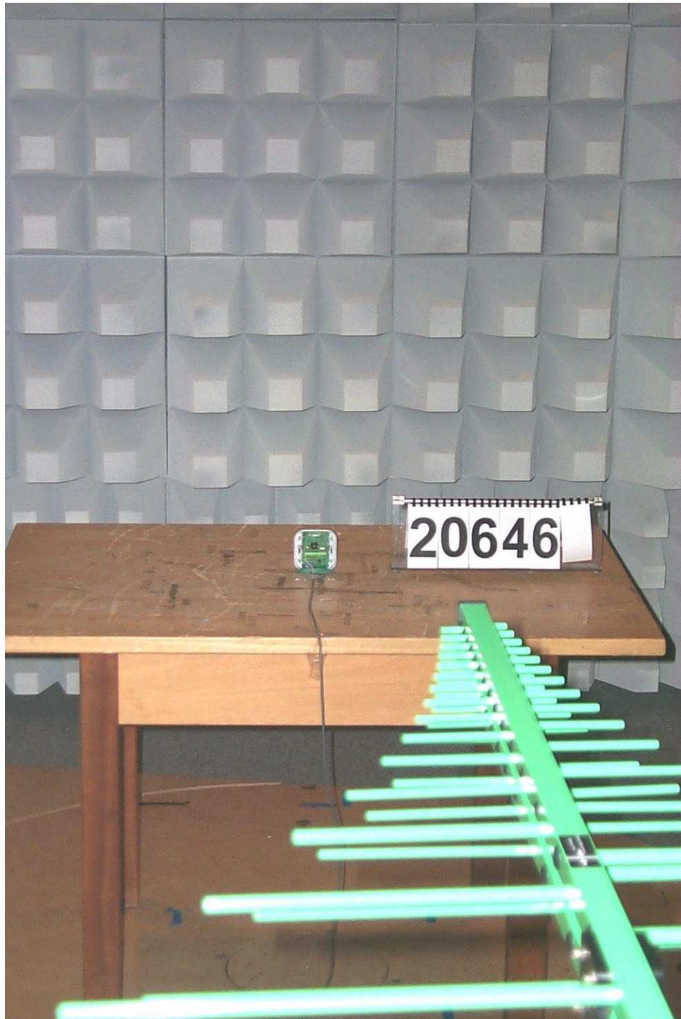
20646_c.jpg test set-up preliminary emission measurement (30 MHz to 1 GHz)
