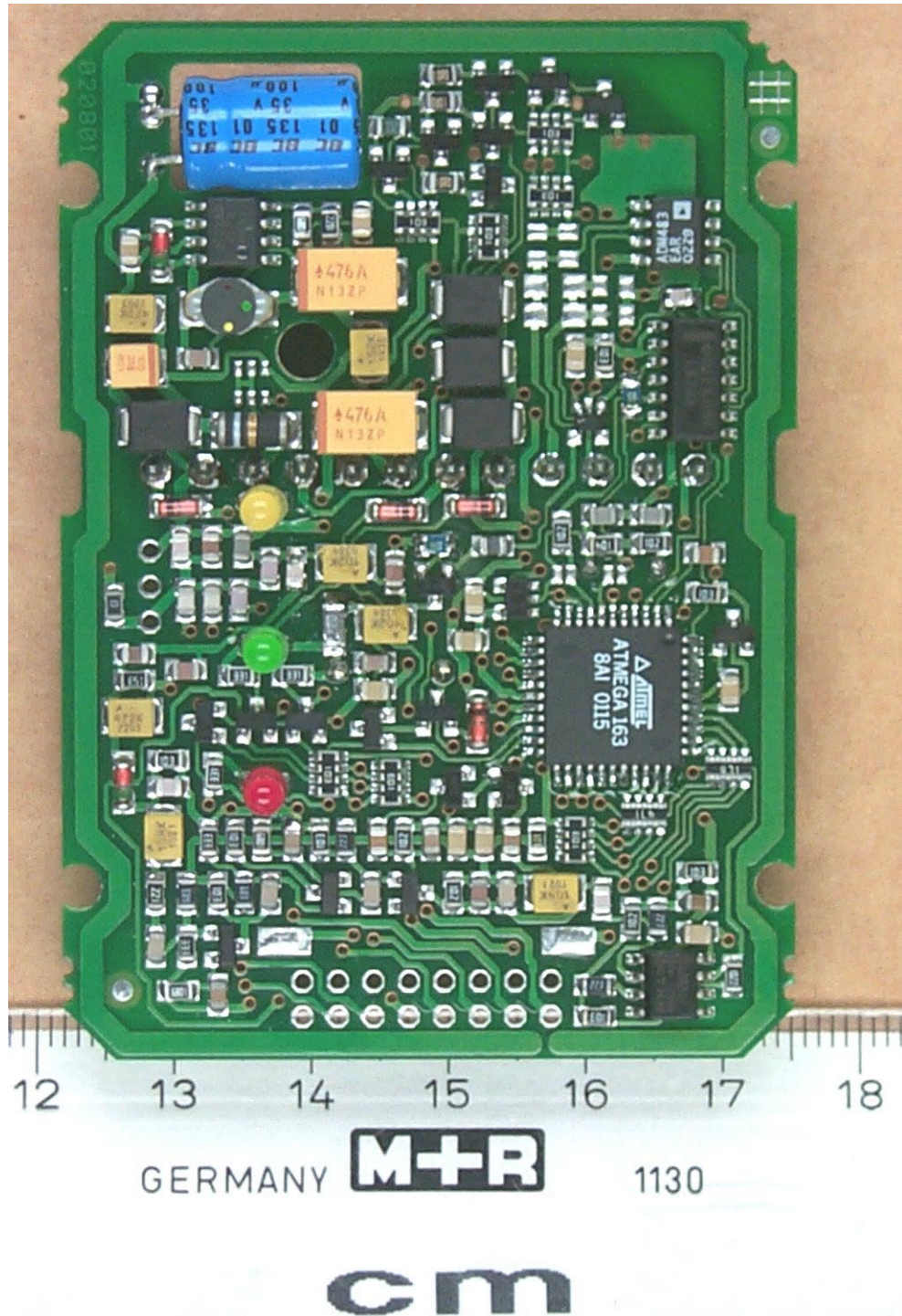
20646_4.jpg Model 240 (PRA5) PVB, bottom view
