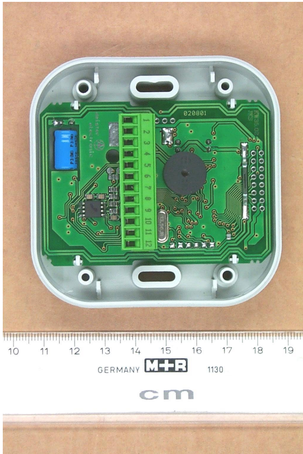
20646_2.jpg Model 240 (PRA5) internal view
