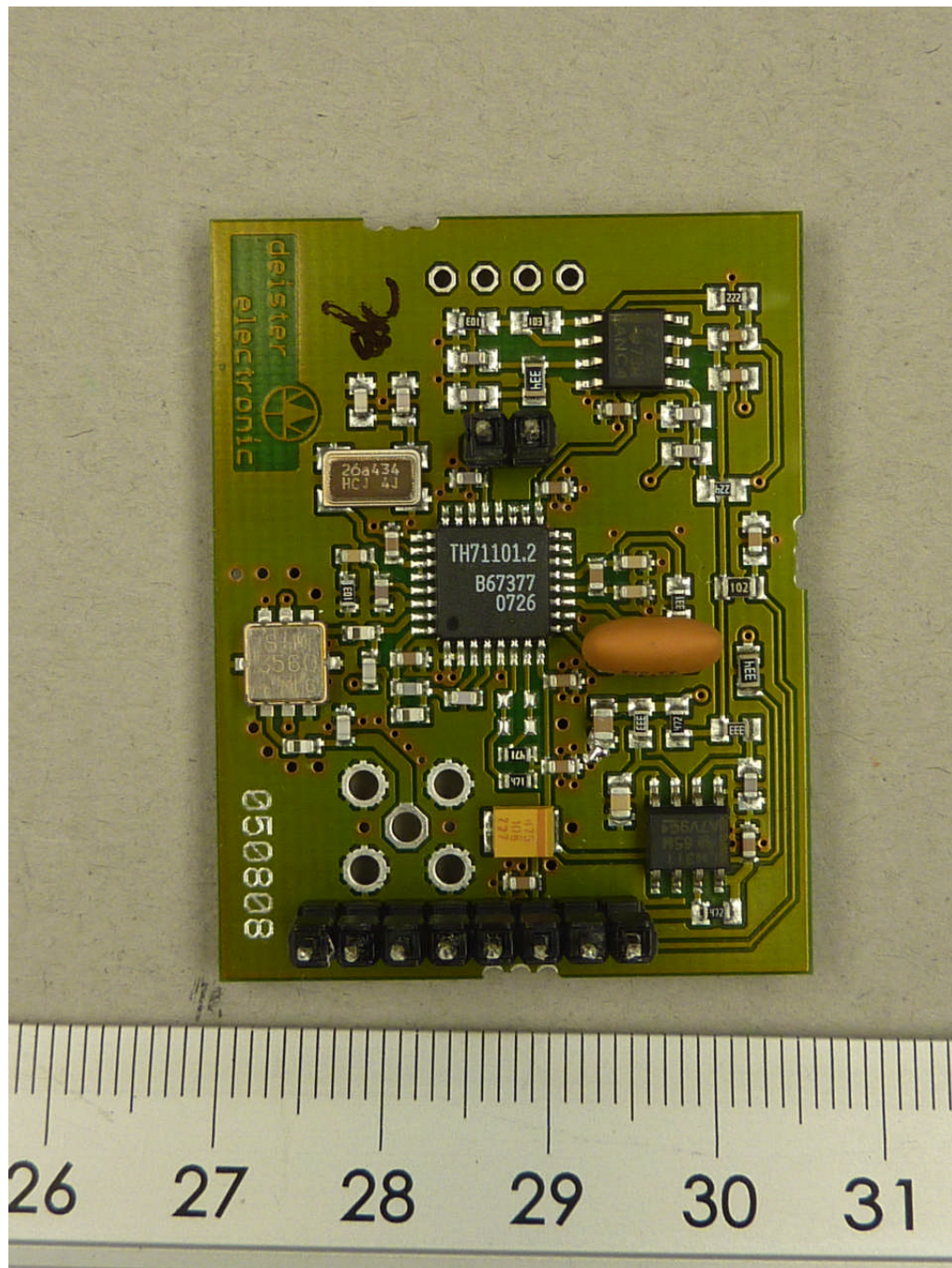
111945_f.JPG: Amantag Compact, subPCB 1, top view
