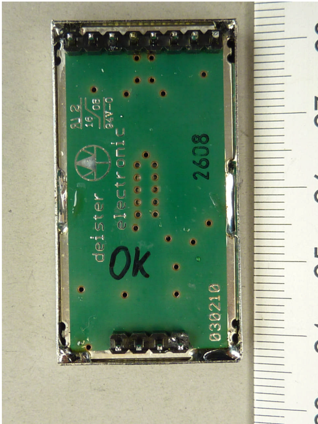
111945_h.JPG: Amantag Compact, subPCB 2, bottom view
