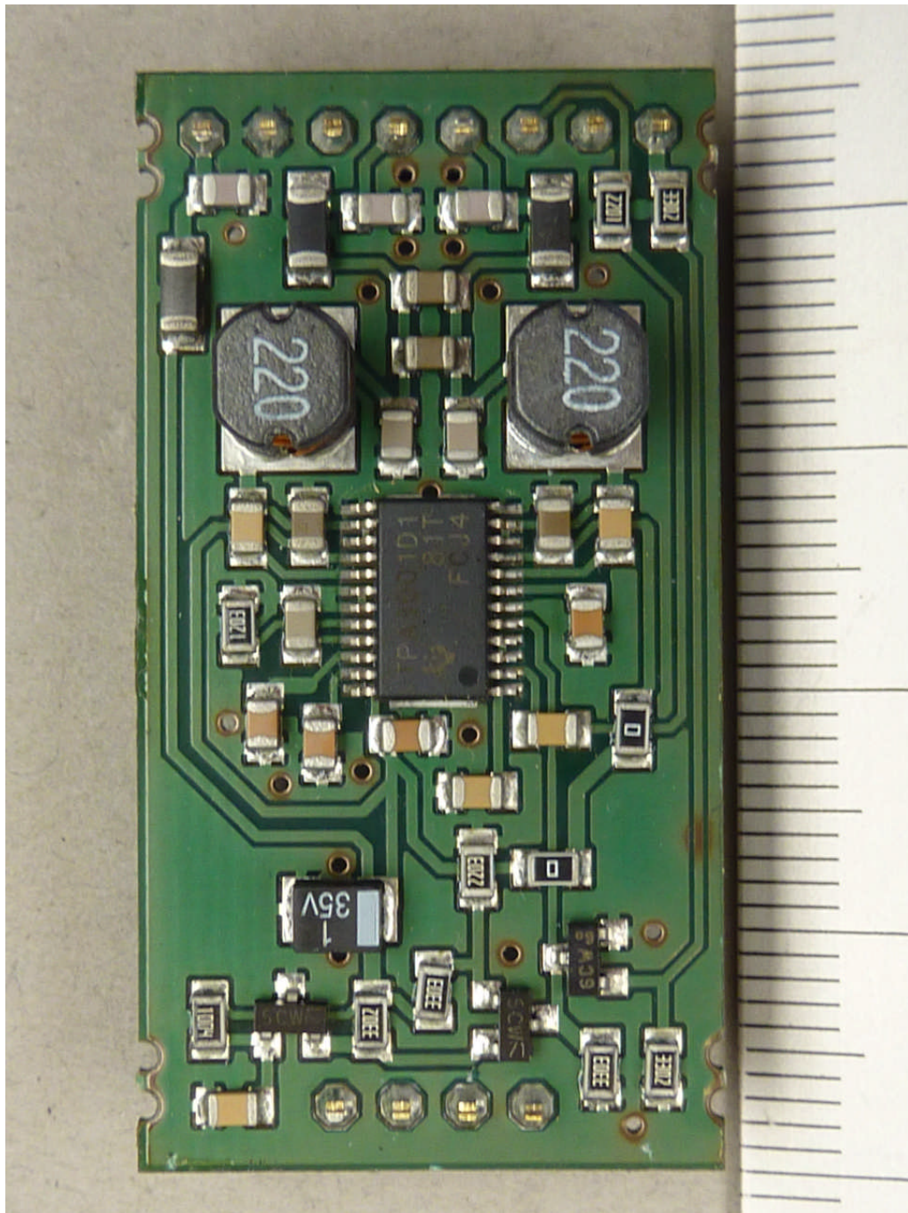
111945_i.JPG: Amantag Compact, subPCB 2, top view, shielding removed
