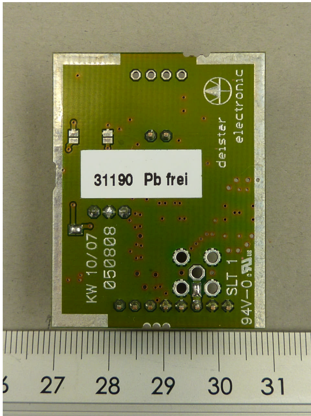
111945_g.JPG: Amantag Compact, subPCB 1, bottom view
