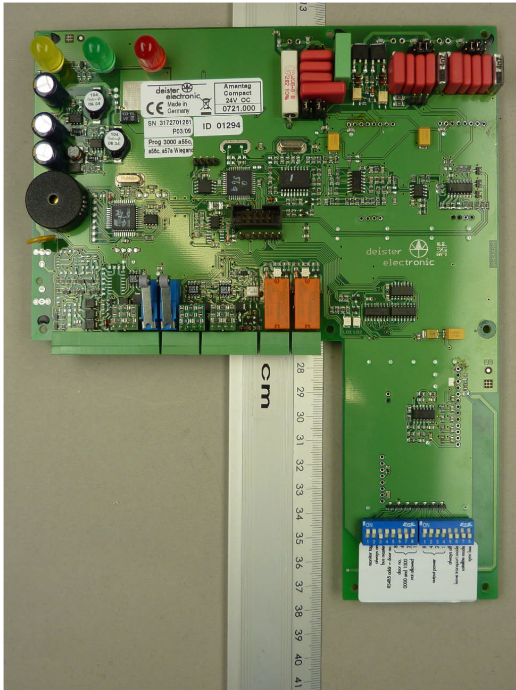
111945_j.JPG: Amantag Compact, main PCB, top view, sub PCBs removed
