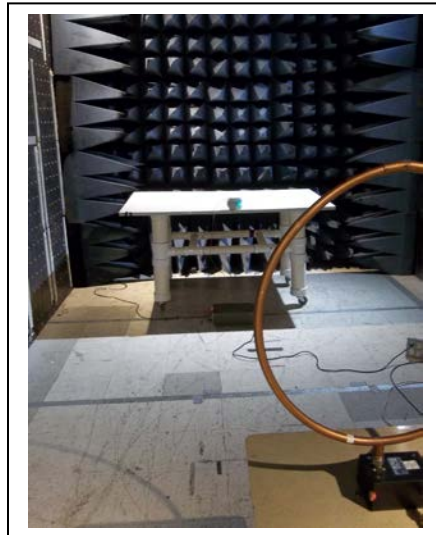
Loop Antenna
