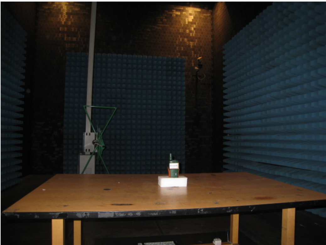
Photo 2 Rear of Radiated Disturbance Test, Measuring Mode
