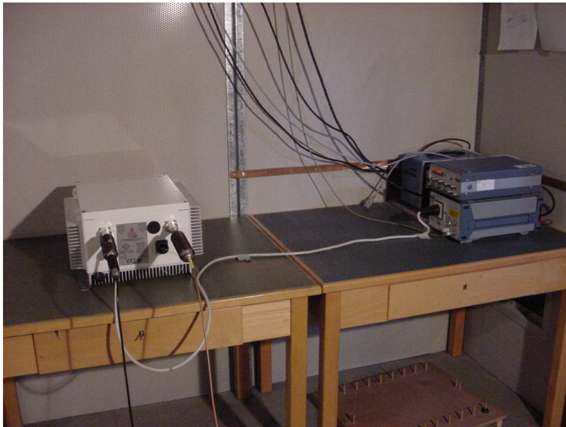
Photo 3: Conducted Emissions
