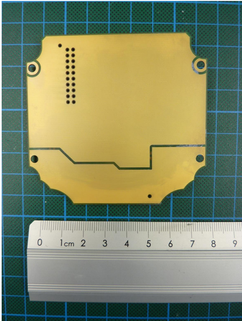
171663_19.JPG: IUHF190V1B, PCB 3, bottom view
