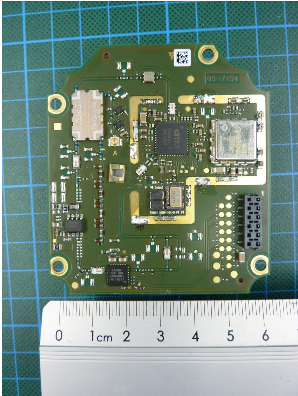
171663_16.JPG: IUHF190V1B, PCB 2, top view, shielding removed
