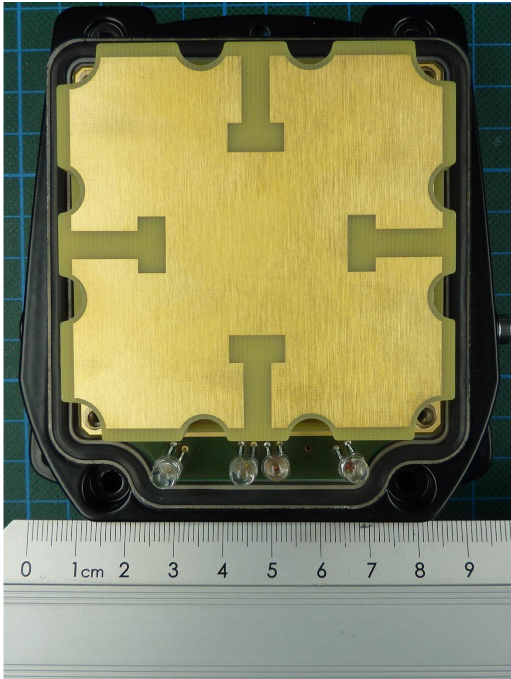
171663_22.JPG: IUHF190V1B, internal view 1 (top housing removed)
