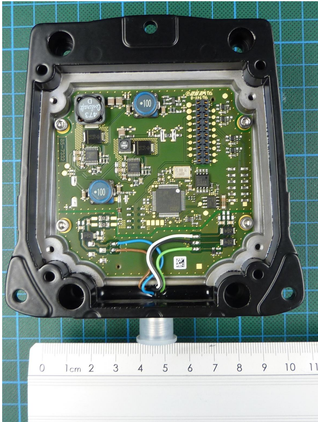
171663_9.JPG: IUHF190V1B, internal view 4 (without rear cover)
