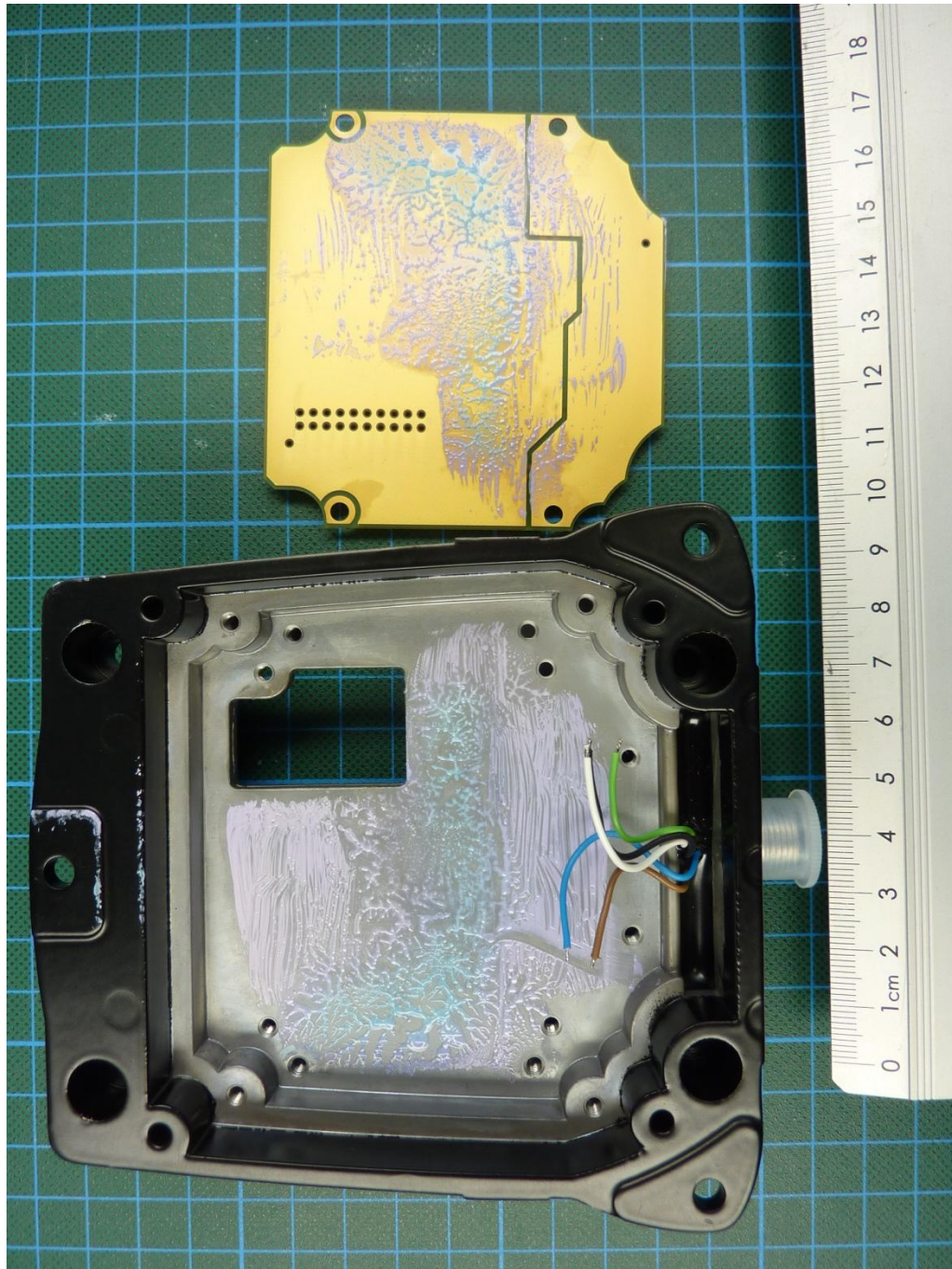
171663_17.JPG: IUHF190V1B, internal view 5 (PCB 3 removed)
