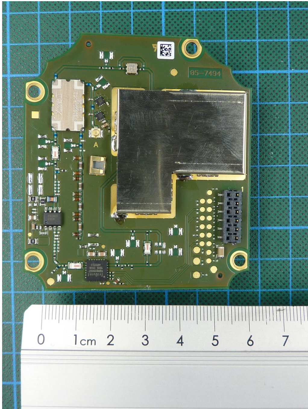
171663_13.JPG: IUHF190V1B, PCB 2, top view
