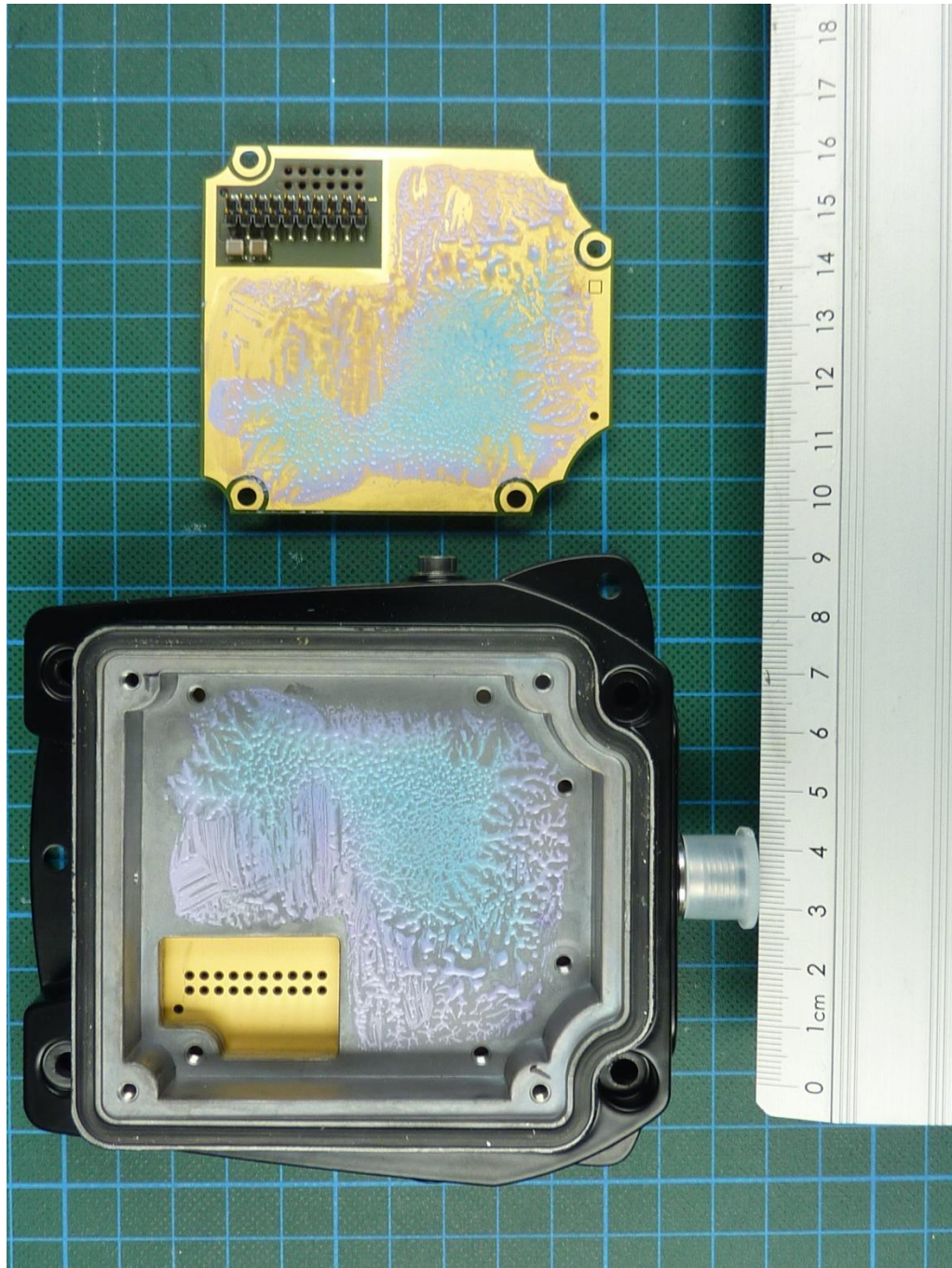
171663_11.JPG: IUHF190V1B, internal view 3 (PCB 2 removed)
