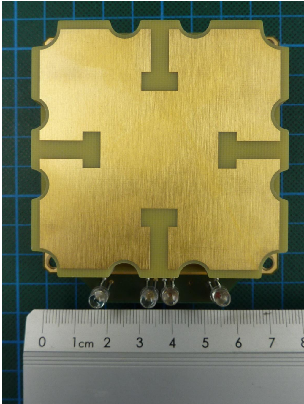
171663_7.JPG: IUHF190V1B, antenna, top view
