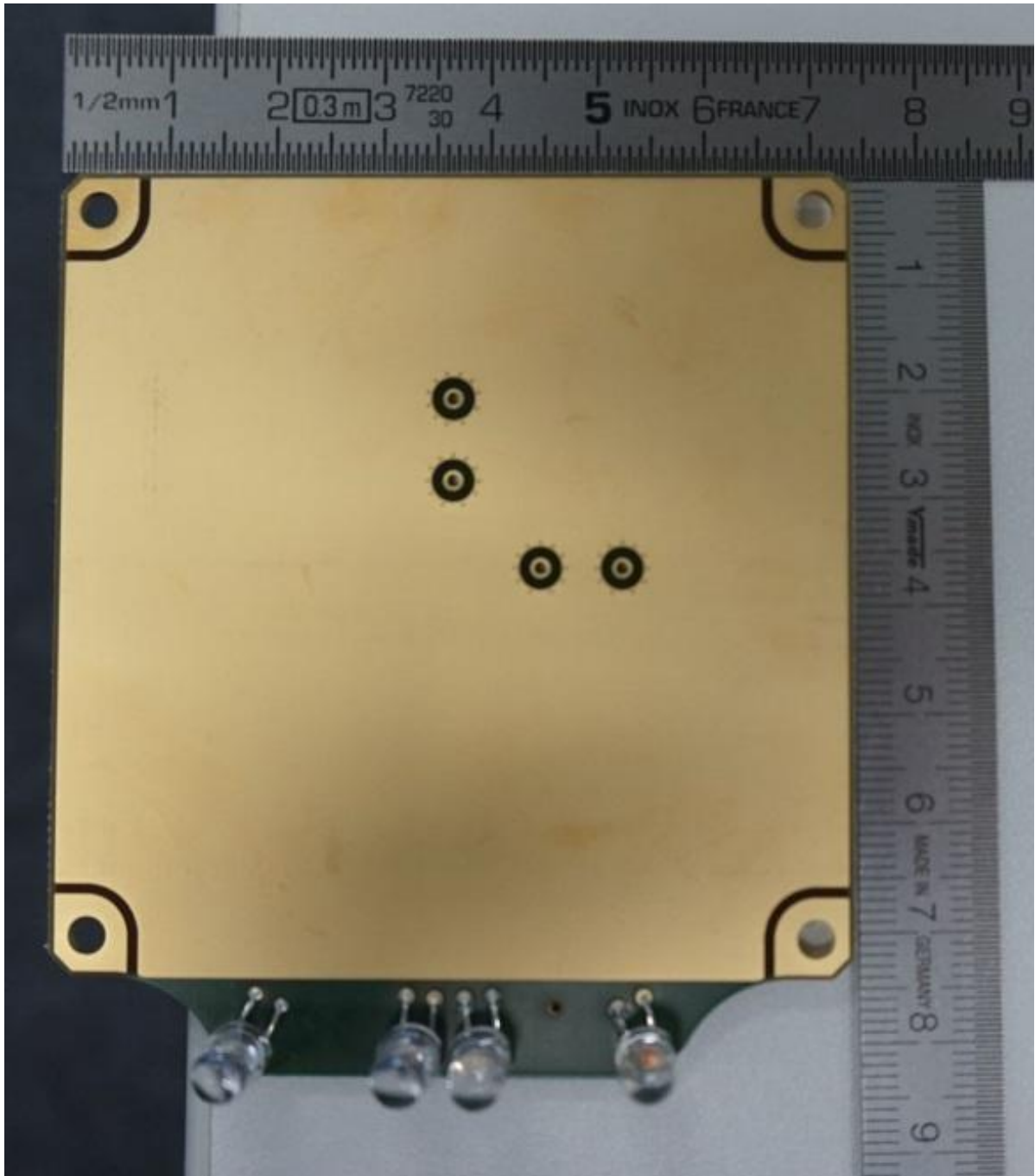
171663_20.JPG: IUHF190V1B, PCB 1, bottom view (antenna removed)
