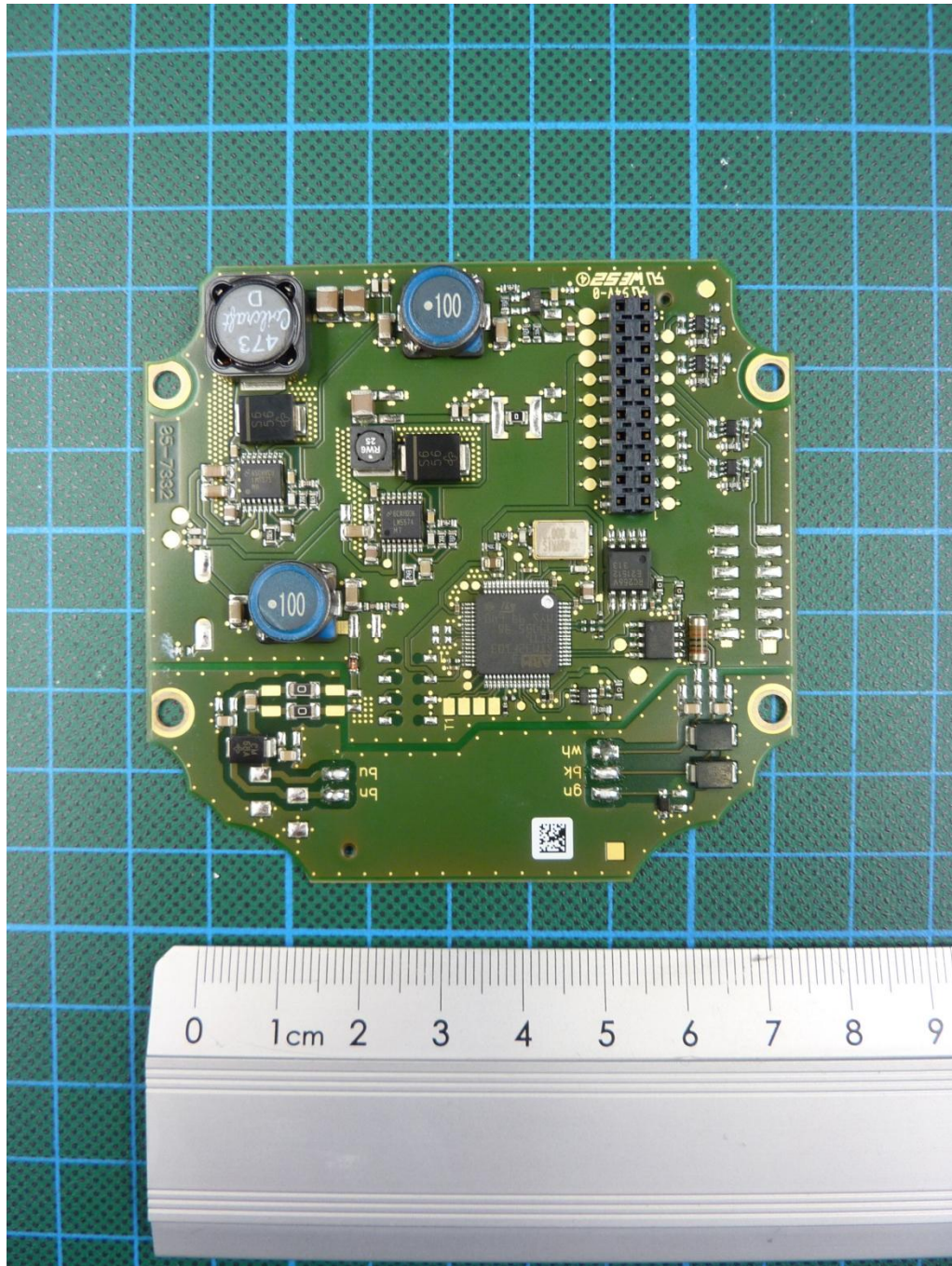
171663_18.JPG: IUHF190V1B, PCB 3, top view
