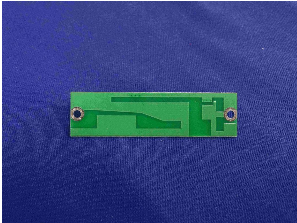
(23) EUT Photo –Aux Antenna
