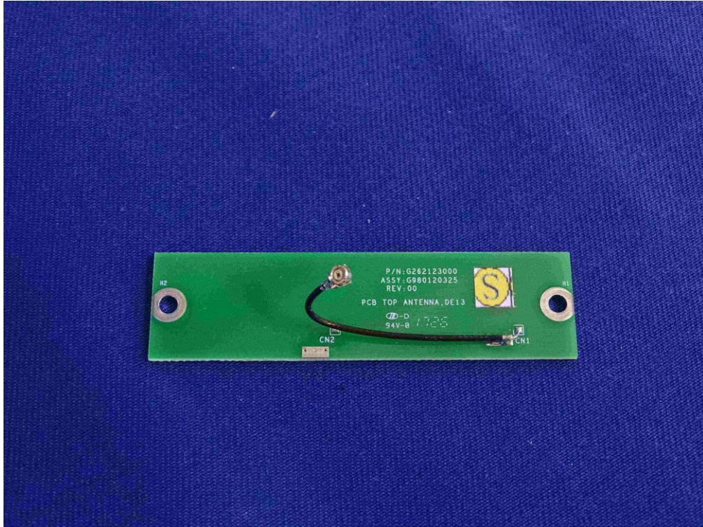
(20) EUT Photo –Main Antenna
