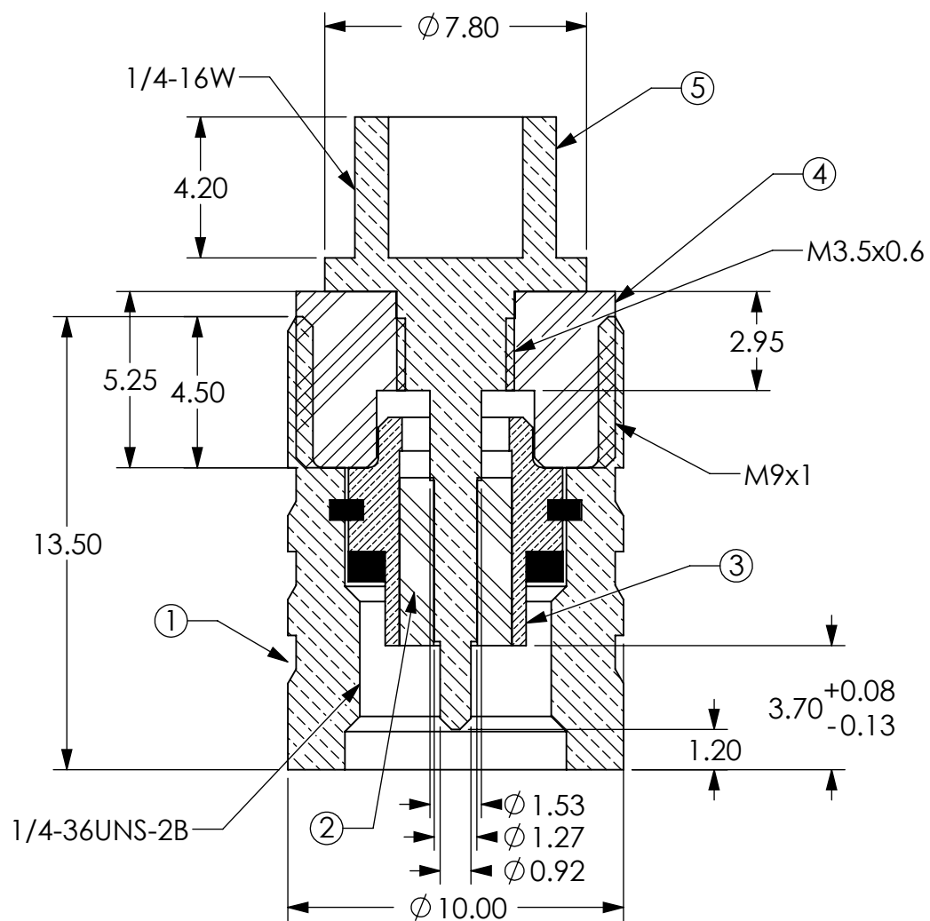
SECTION B-B
