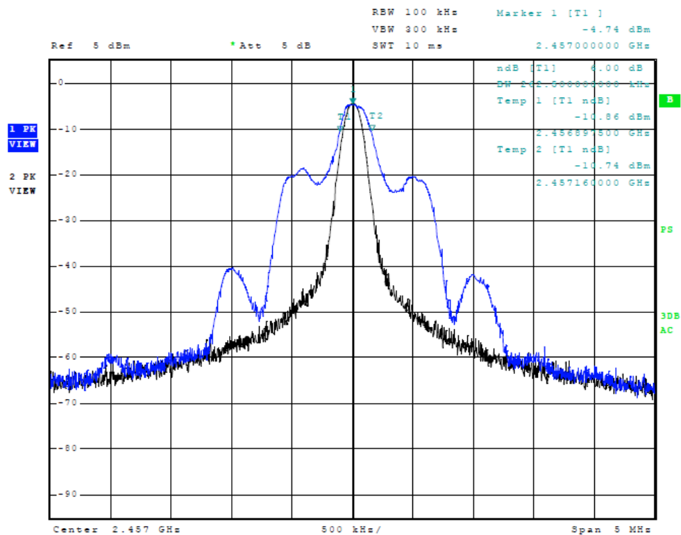
Figure 2 Plot of Transmitter Emissions (Occupied Bandwidth)
