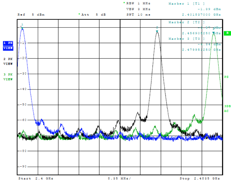
Figure 1 Plot of Transmitter Emissions (Output in Operational Band)
