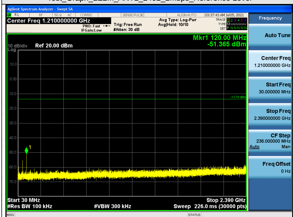
Test Graph LE2M ANT1 2402 2Mbps Lower Band Emissions
