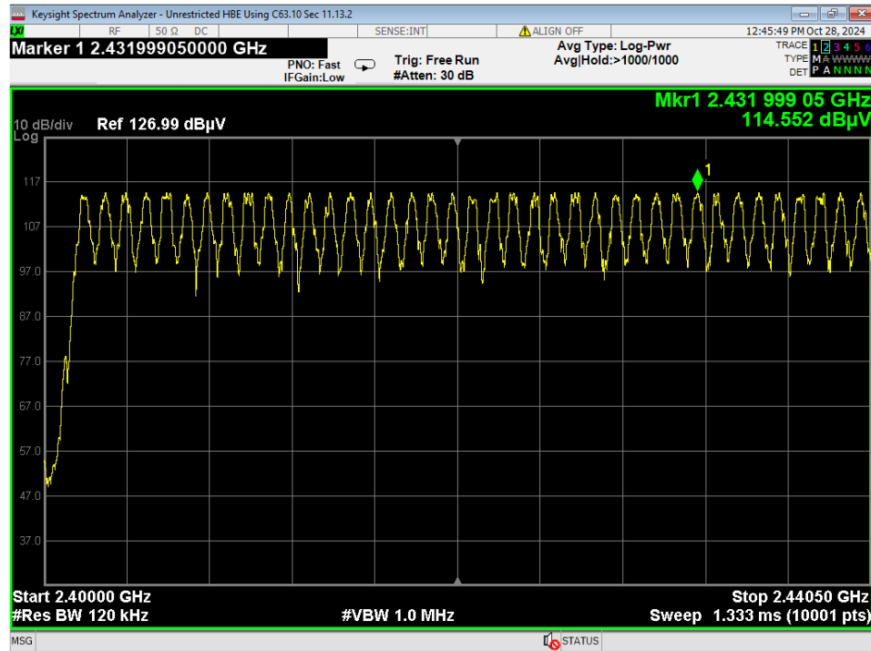
13 Channel Count, 2400-2440.5M
