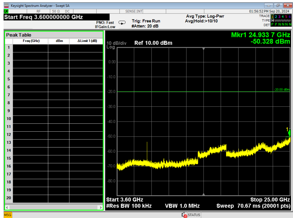
Figure 9 - Conducted Emissions Plot, BTBR, 3.6G – 25G
