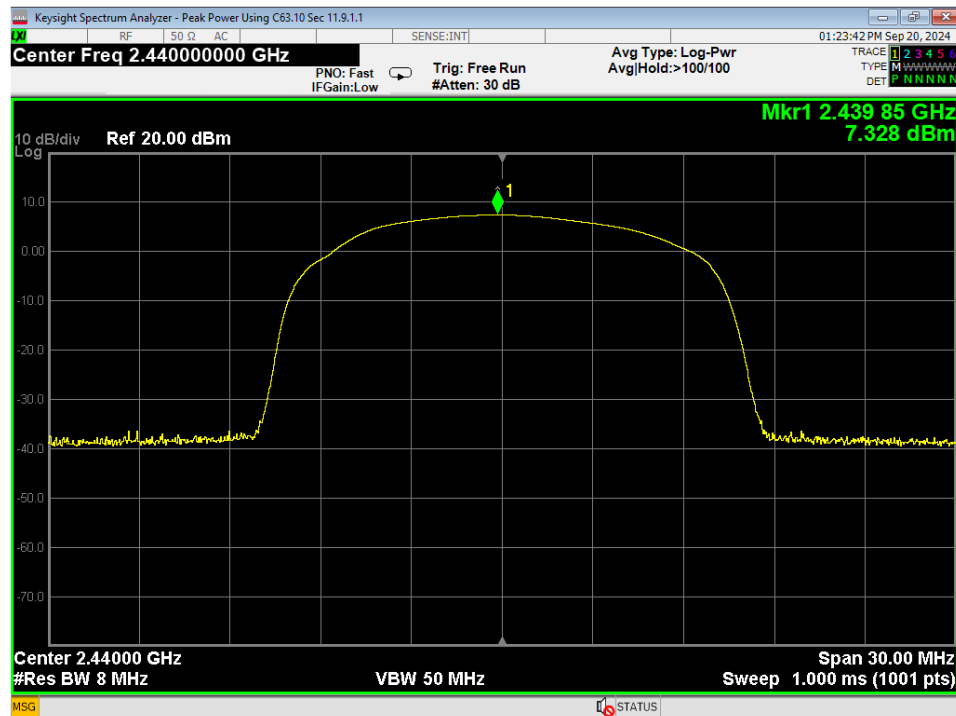
02 Peak Power, Mid Channel, BTBR
