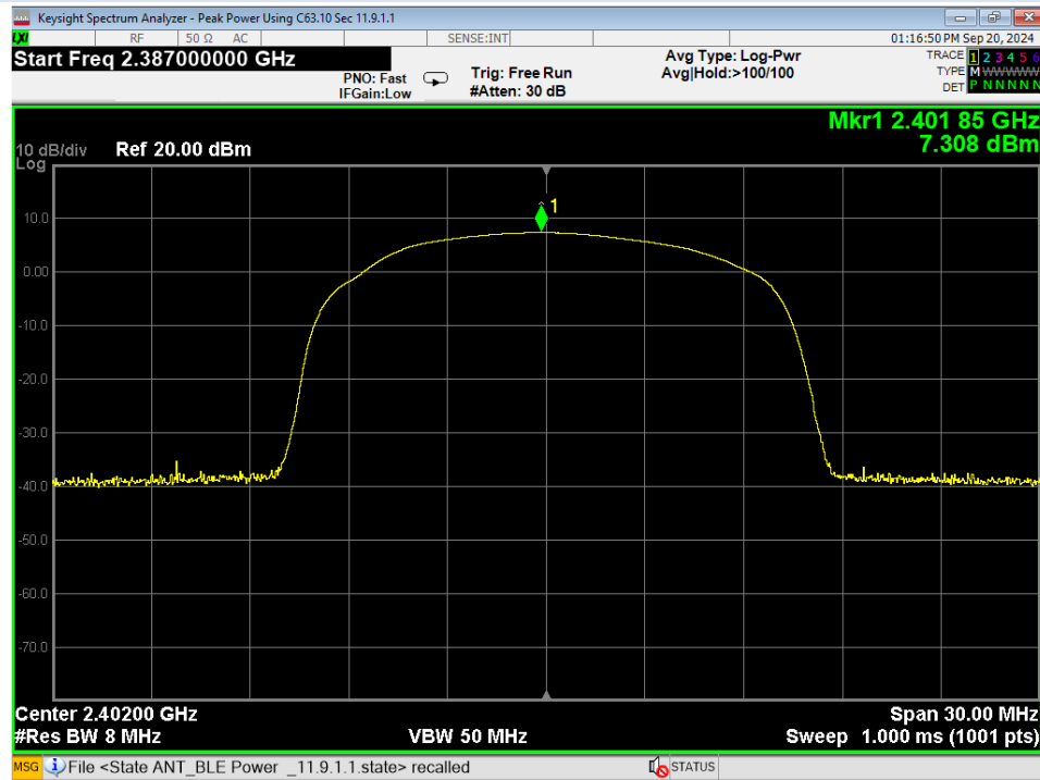
01 Peak Power, Low Channel, BTBR
