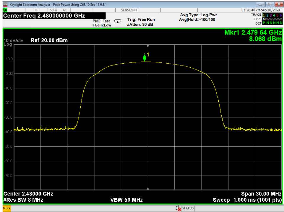
03 Peak Power, High Channel, BTBR
