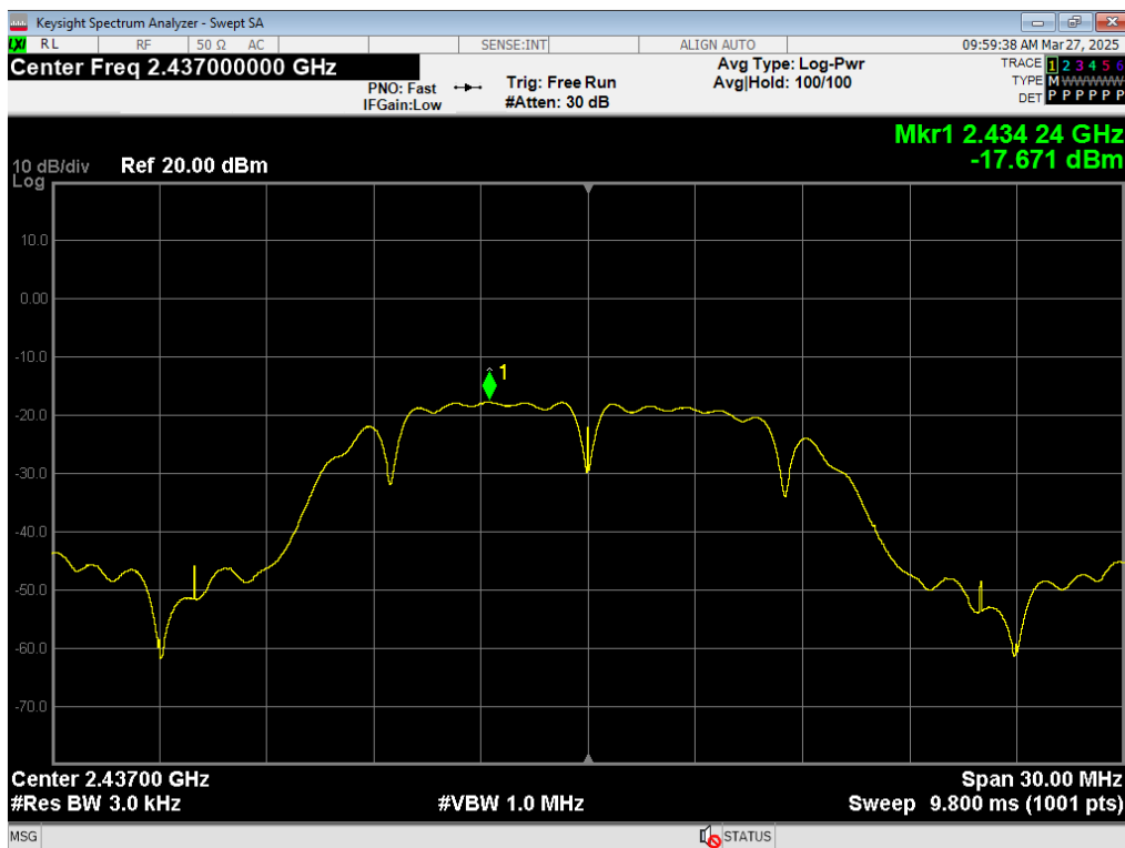
74 PSD, WiFi B 1MB, 2437MHz
