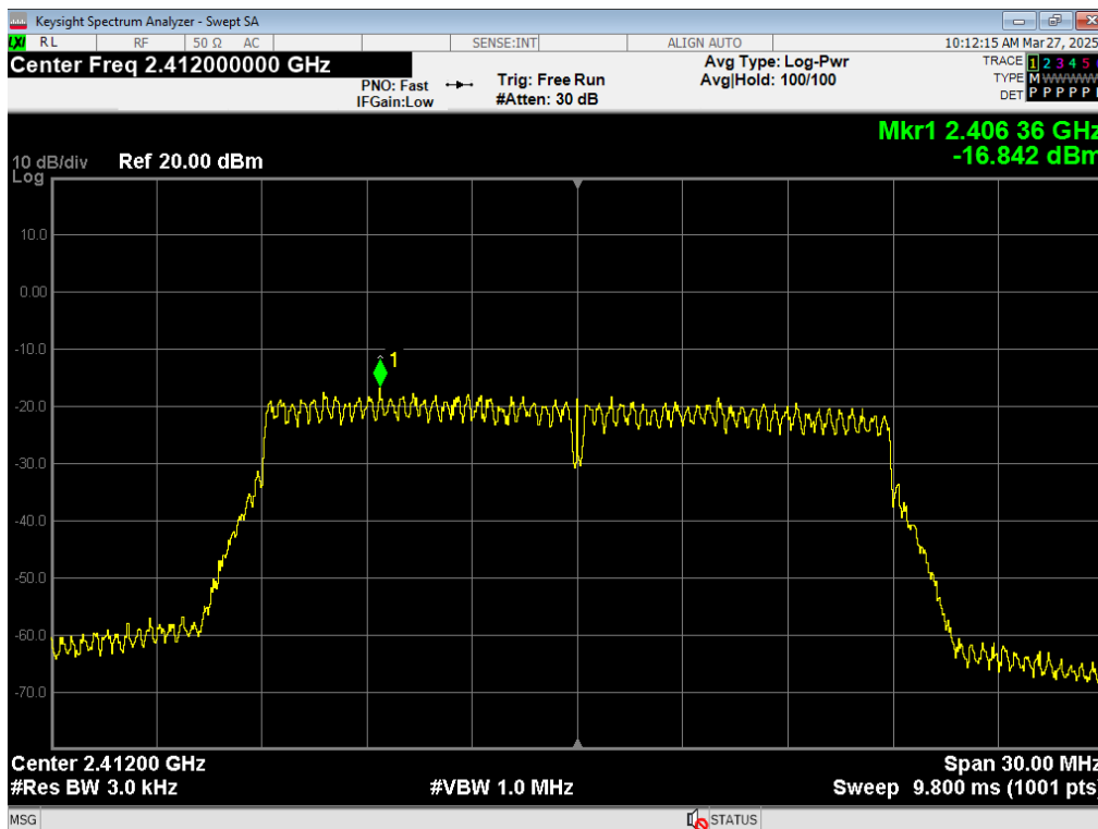
85 PSD, WiFi N MCS0, 2412MHz
