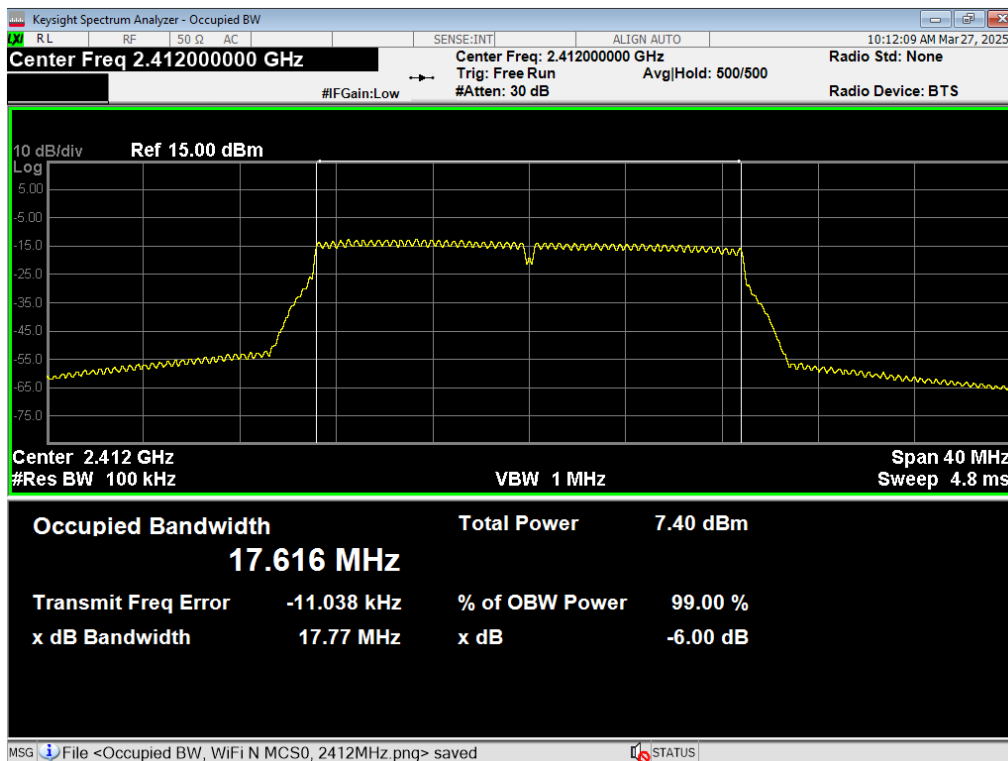
13 6dB BW, WiFi N MCS0, 2412MHz
