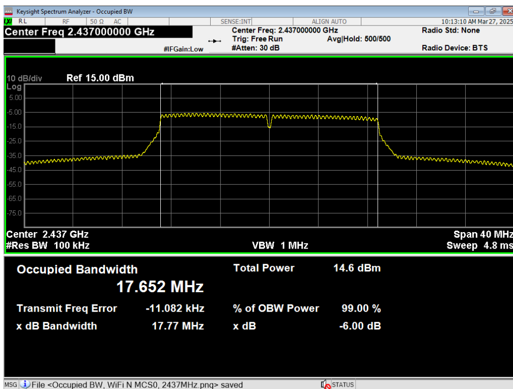
14 6dB BW, WiFi N MCS0, 2437MHz
