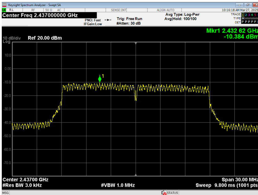
89 PSD, WiFi N MCS7, 2437MHz
