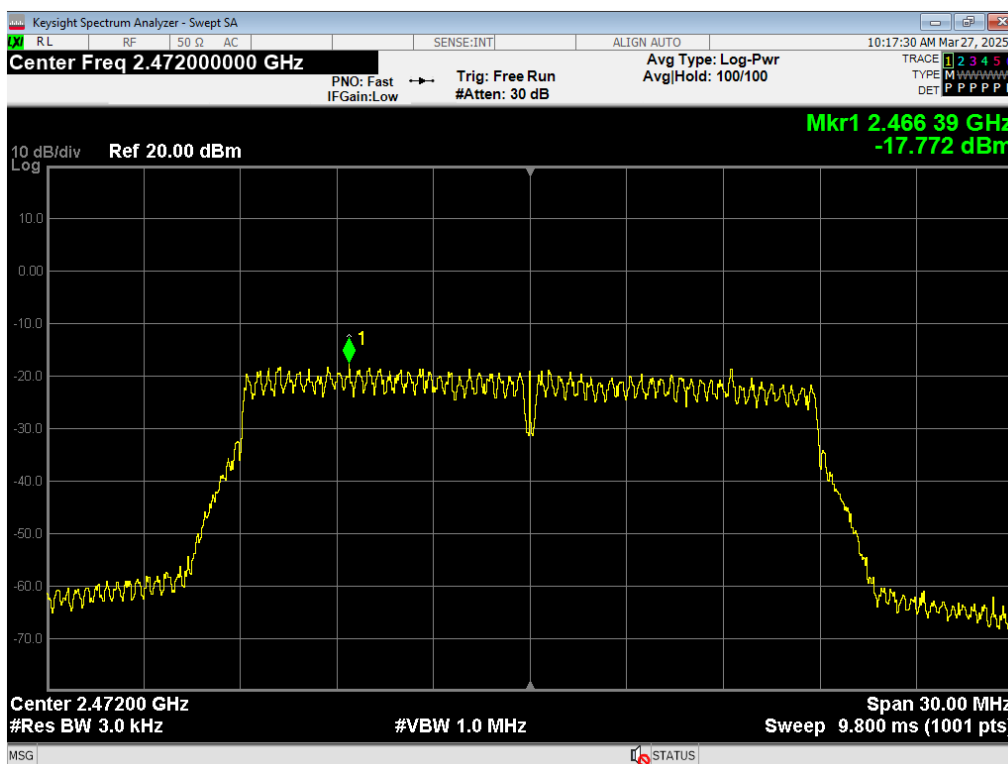
90 PSD, WiFi N MCS7, 2472MHz
