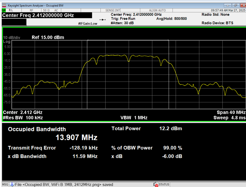
01 6dB BW, WiFi B 1MB, 2412MHz
