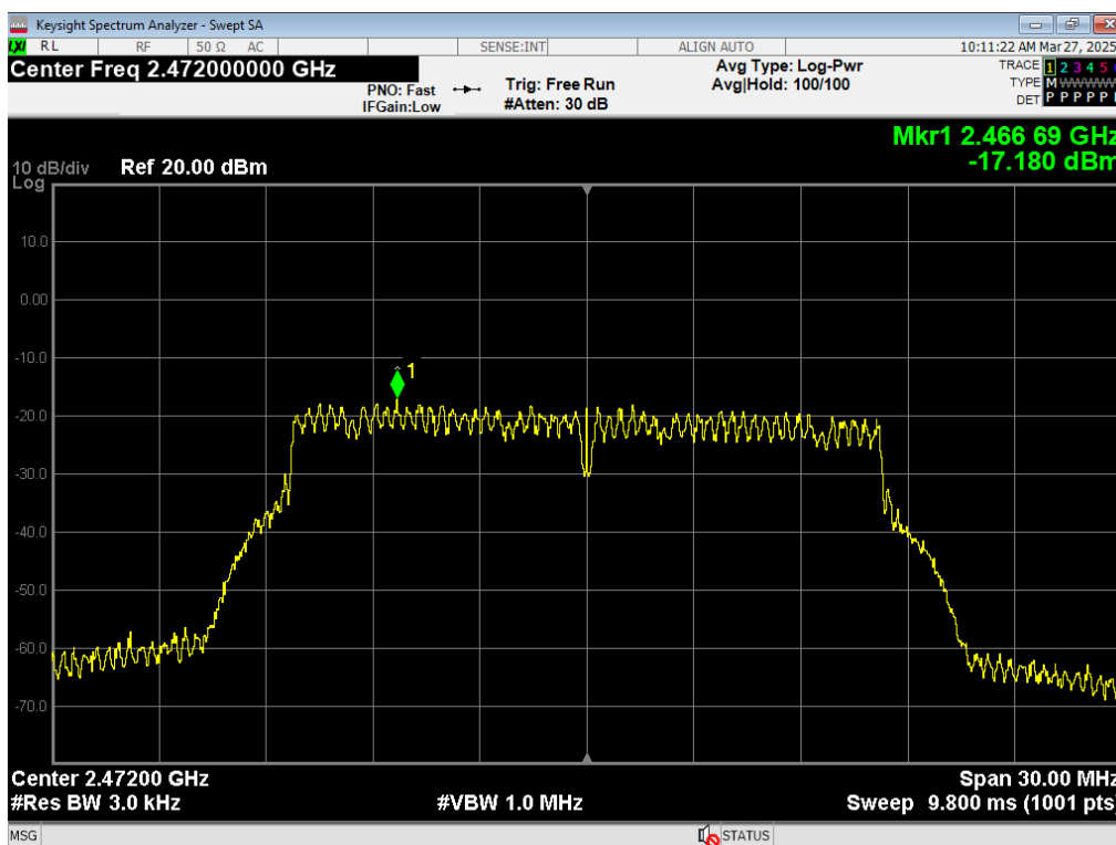
84 PSD, WiFi G 54MB, 2472MHz
