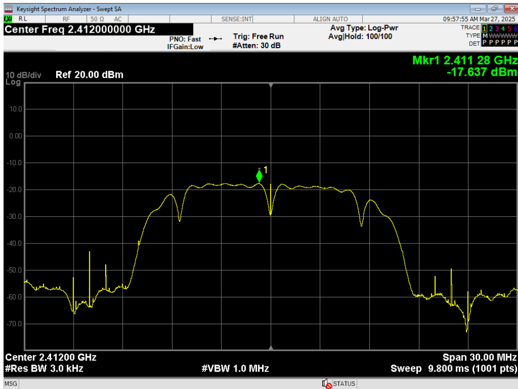
73 PSD, WiFi B 1MB, 2412MHz
