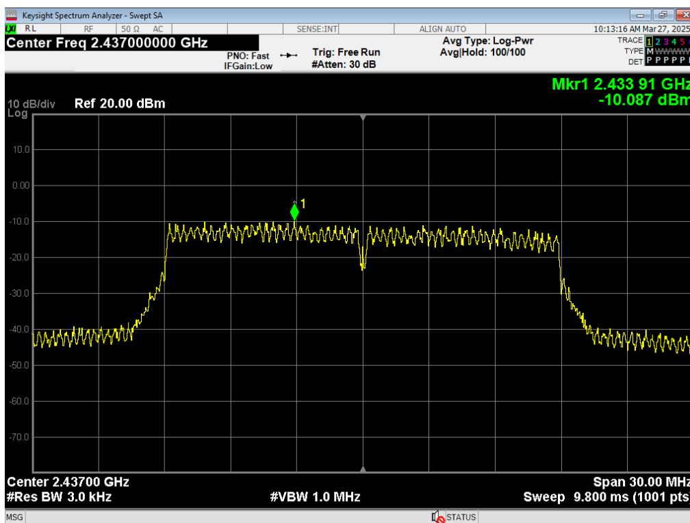
86 PSD, WiFi N MCS0, 2437MHz
