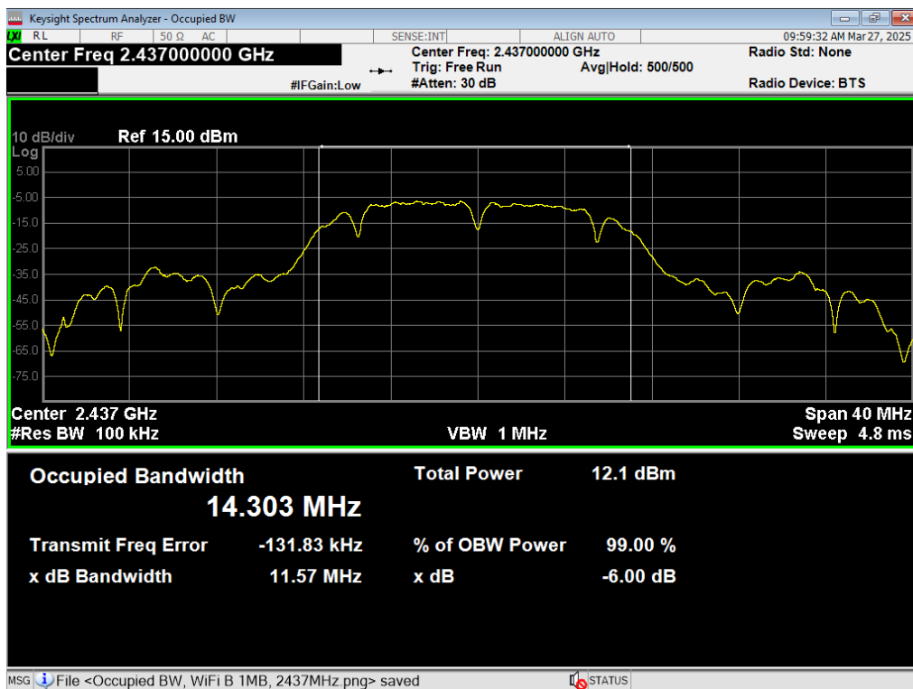
02 6dB BW, WiFi B 1MB, 2437MHz
