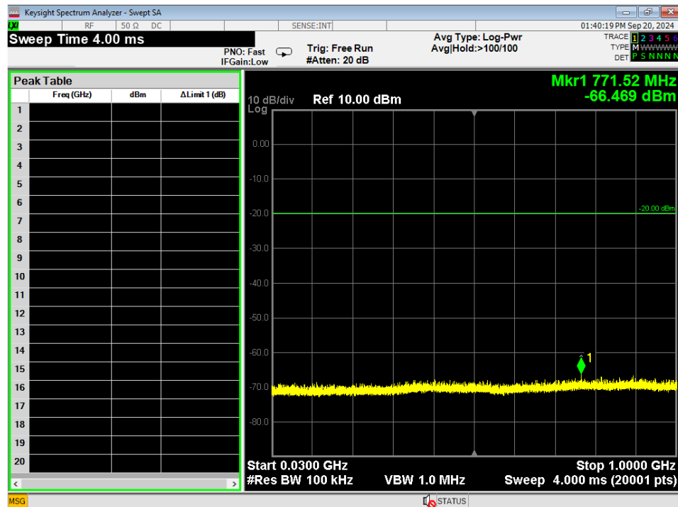
Figure 13 - Conducted Emissions Plot, GMSK 1MB, 30MHz – 1GHz, Mid
