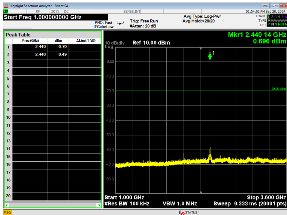
Figure 11 - Conducted Emissions Plot, GFSK, 1GHz – 3.6GHz, Mid
