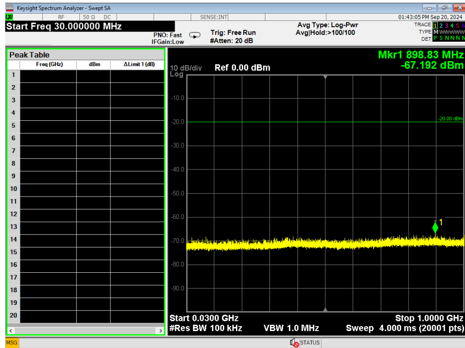
Figure 16 - Conducted Emissions Plot, GMSK 2MB, 30MHz – 1GHz, Mid
