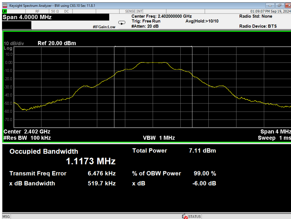
07, 6dB Bandwidth, ANT GFSK, Low
