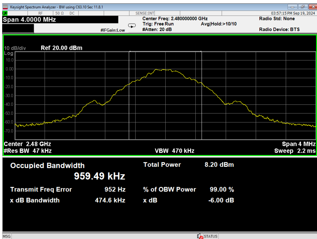
06, Occupied Bandwidth, ANT GFSK, High
