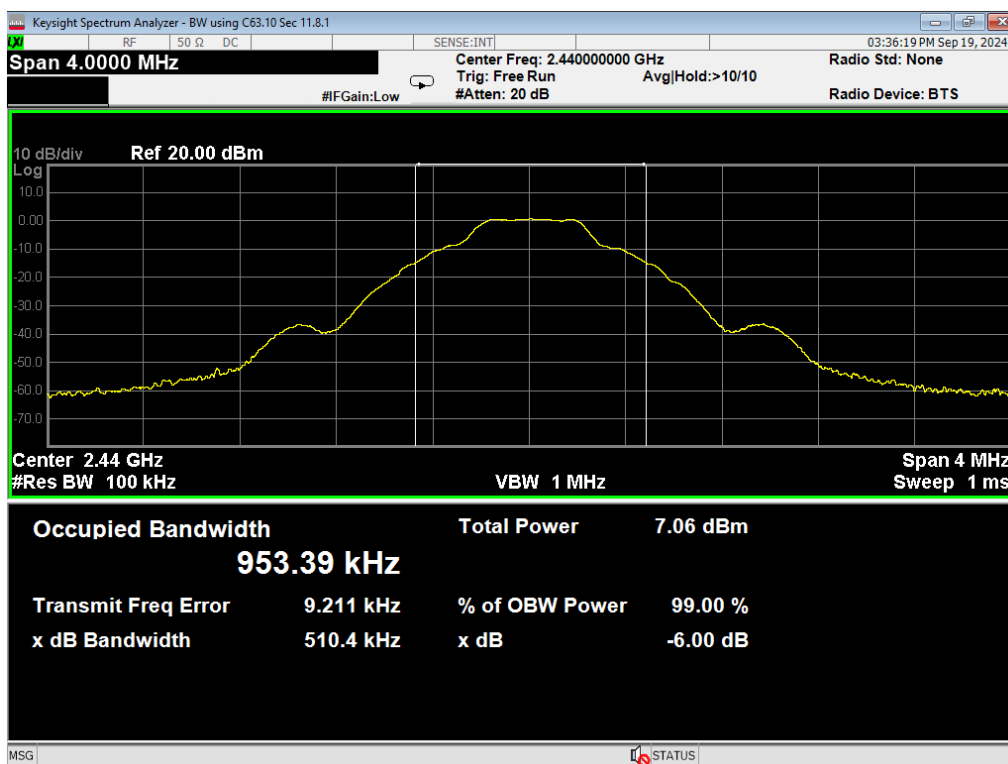
08, 6dB Bandwidth, ANT GFSK, Mid
