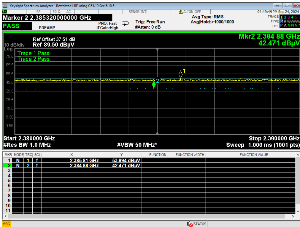
15, LBE Restricted, ANT GFSK
