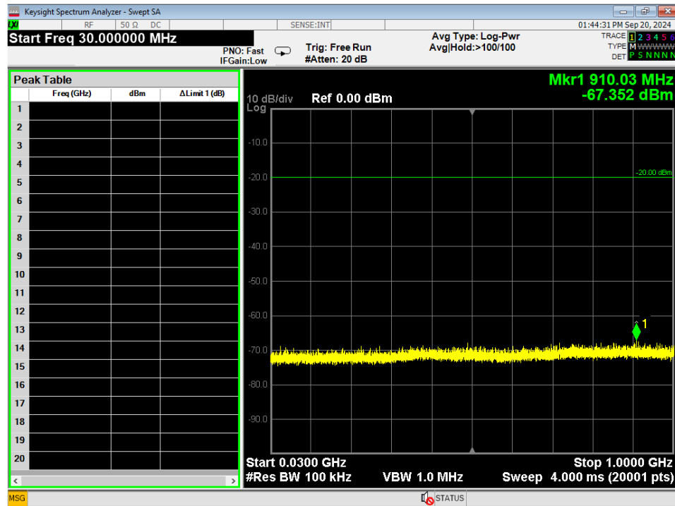
Figure 10 - Conducted Emissions Plot, GFSK, 30MHz – 1GHz, Mid
