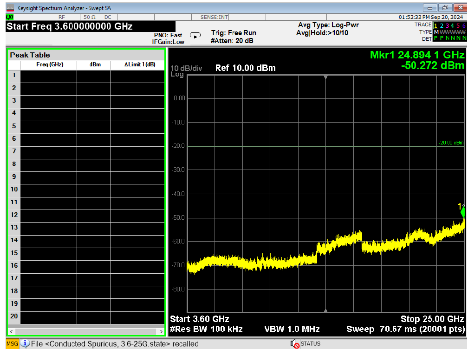
Figure 18 - Conducted Emissions Plot, GMSK 2MB, 3.6GHz – 25GHz, Mid
