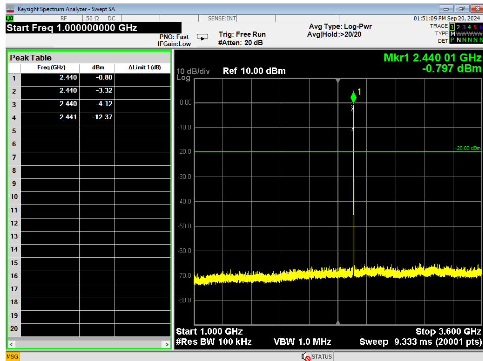
Figure 17 - Conducted Emissions Plot, GMSK 2MB, 1GHz – 3.6GHz, Mid
