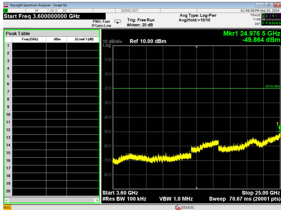
Figure 15 - Conducted Emissions Plot, GMSK 1MB, 3.6GHz – 25GHz, Mid
