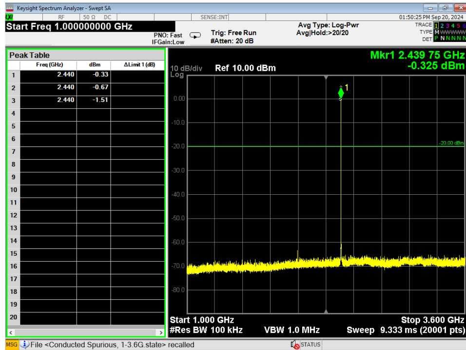
Figure 14 - Conducted Emissions Plot, GMSK 1MB, 1GHz – 3.6GHz, Mid
