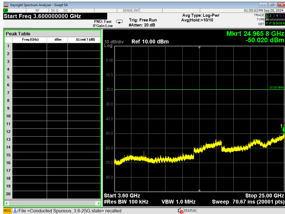
Figure 12 - Conducted Emissions Plot, GFSK, 3.6GHz – 25GHz, Mid
