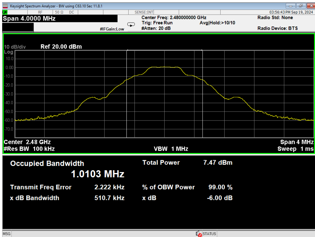
09, 6dB Bandwidth, ANT GFSK, High
