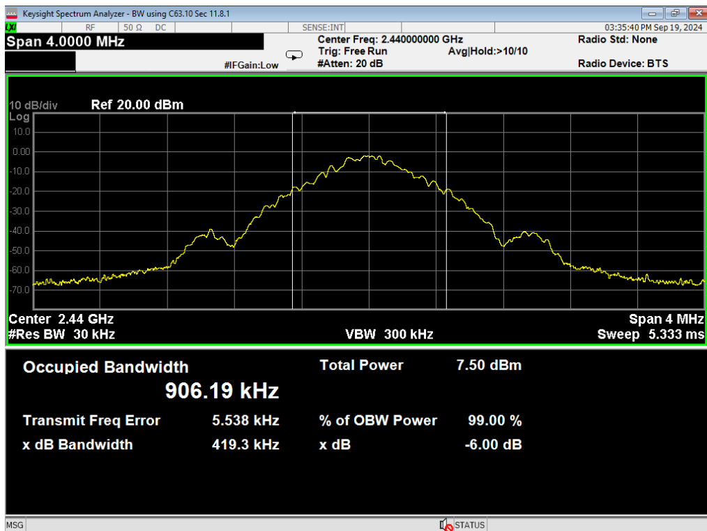
05, Occupied Bandwidth, ANT GFSK, Mid
