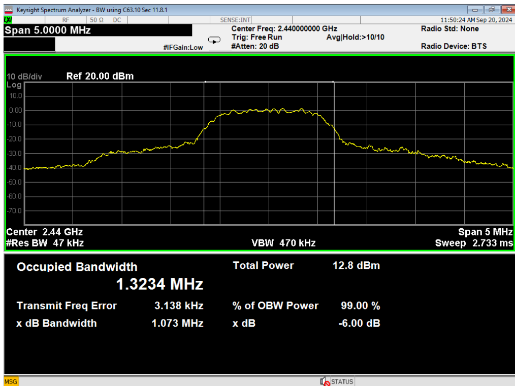
05, Occupied Bandwidth, 2EDR, Mid
