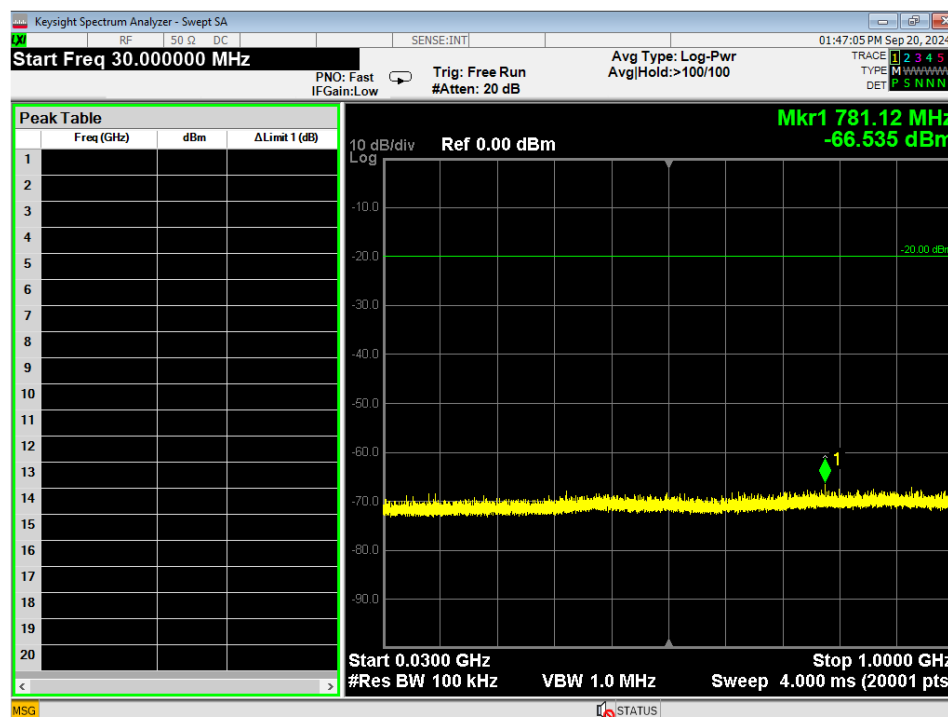
Figure 10 - Conducted Emissions Plot, 3EDR, 30MHz – 1GHz, Mid
