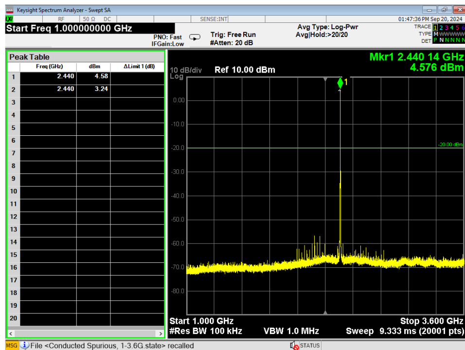
Figure 11 - Conducted Emissions Plot, 3EDR, 1GHz – 3.6GHz, Mid
