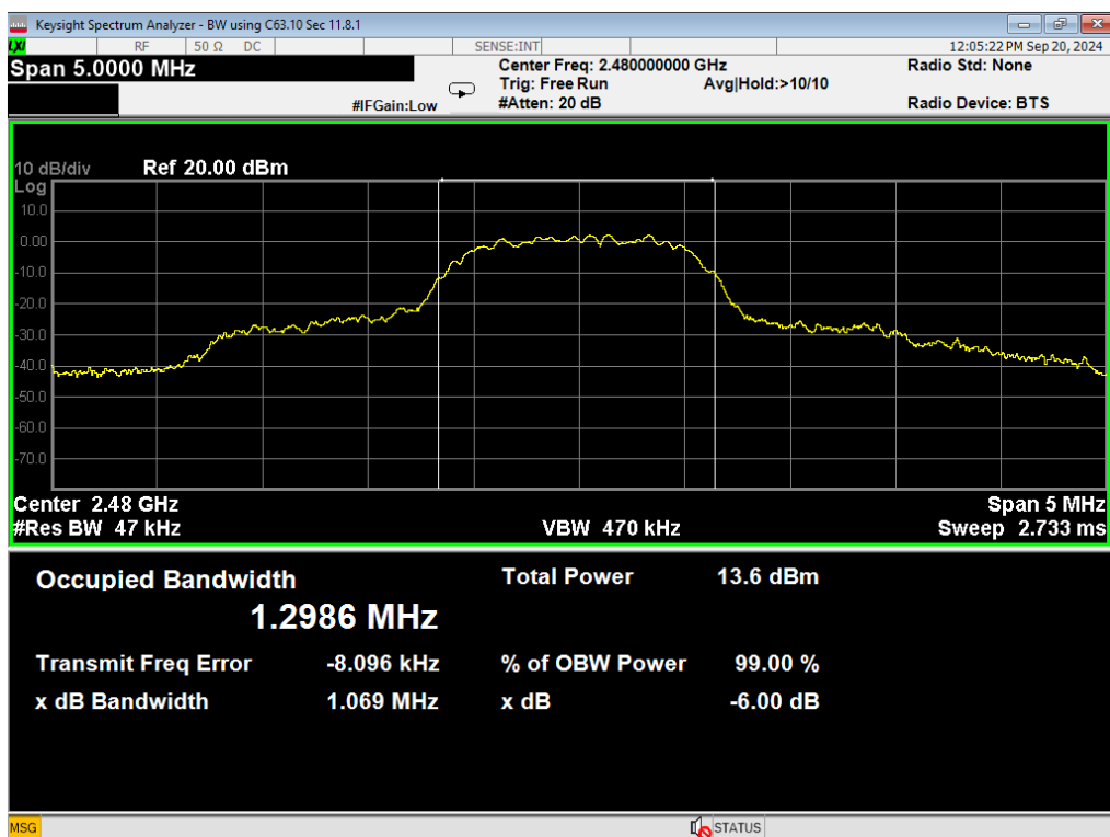
06, Occupied Bandwidth, 2EDR, High
