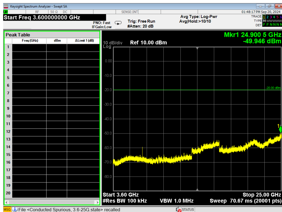
Figure 12 - Conducted Emissions Plot, 3EDR, 3.6GHz – 25GHz, Mid
