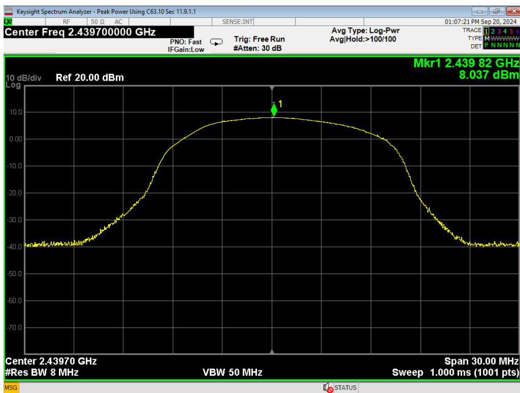
18, Peak Power, 3EDR, Mid
