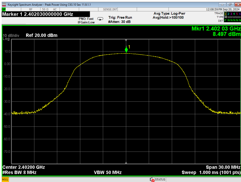
17, Peak Power, 3EDR, Low
