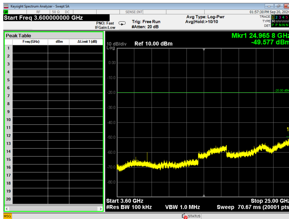
Figure 9 - Conducted Emissions Plot, 2EDR, 3.6GHz – 25GHz, Mid
