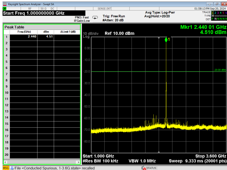
Figure 8 - Conducted Emissions Plot, 2EDR, 1GHz – 3.6GHz, Mid
