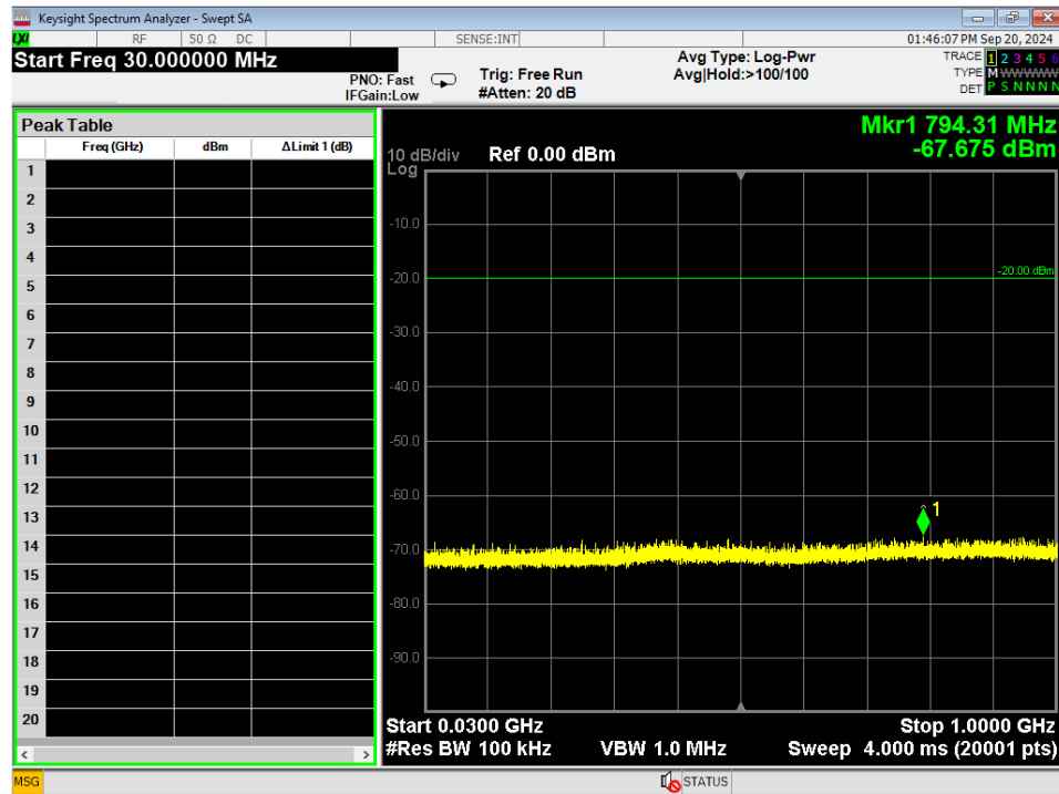
Figure 7 - Conducted Emissions Plot, 2EDR, 30MHz – 1GHz, Mid
