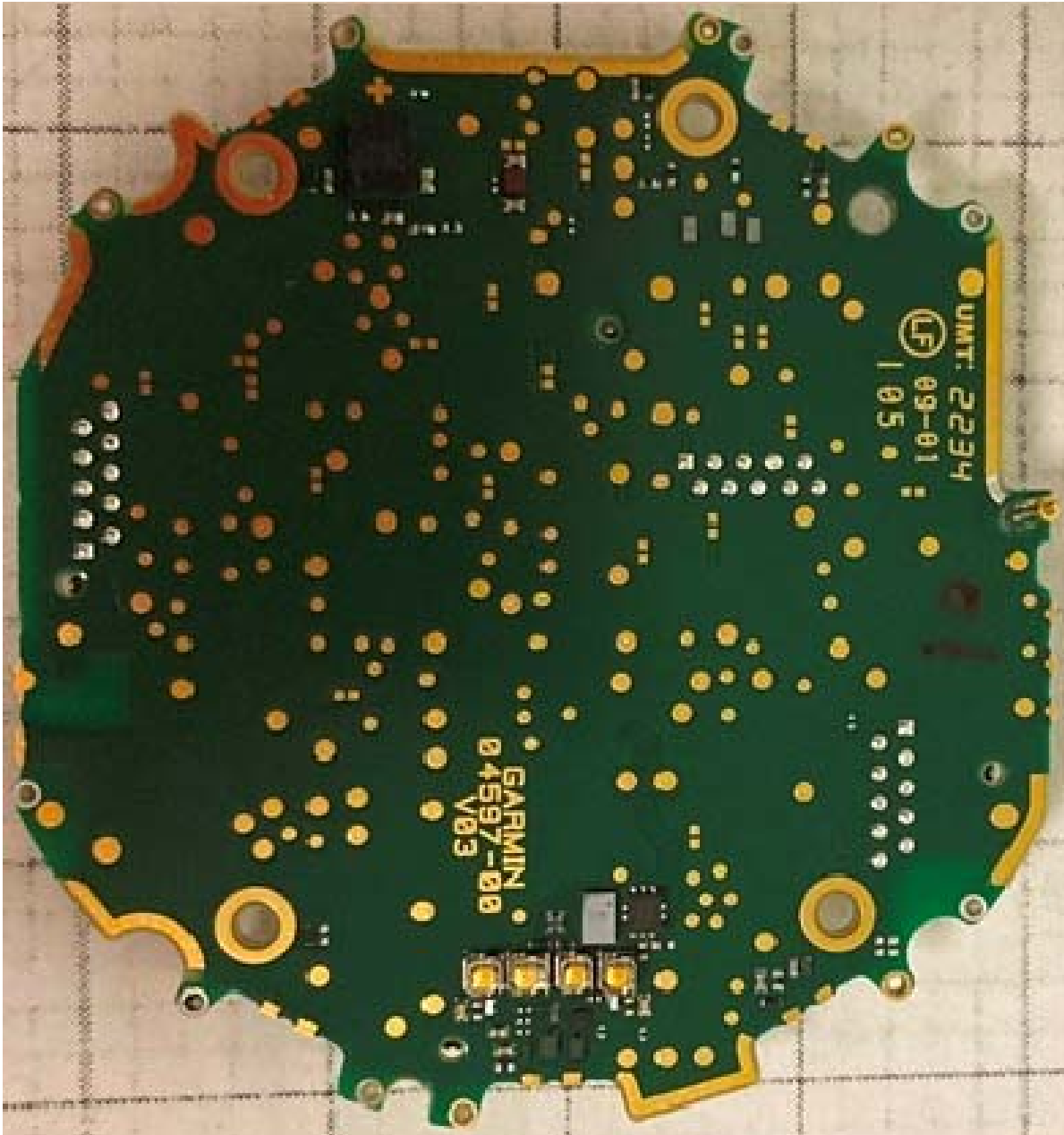
Figure E15.3 – Internal, PCB Bottom Side
