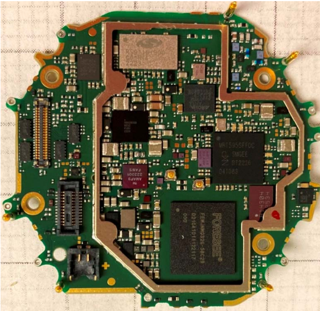
Figure E15.5 – Internal, PCB Top Side, Shield Removed
