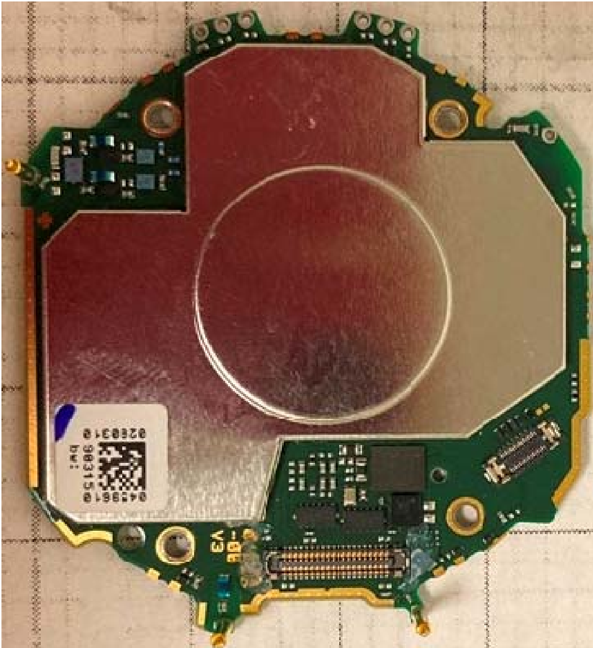
Figure E15.4 – Internal, PCB Top Side
