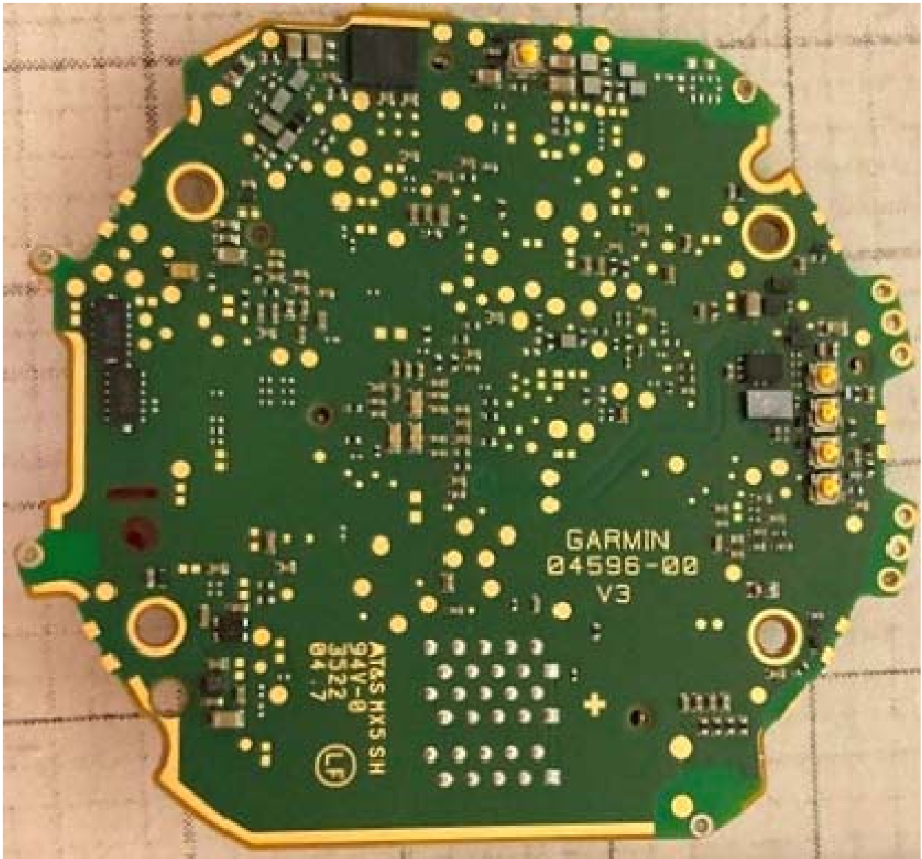
Figure E15.5 – Internal, PCB Bottom Side, Shield Removed
