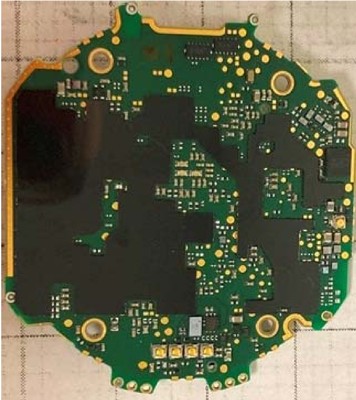
Figure E15.3 – Internal, PCB Bottom Side
