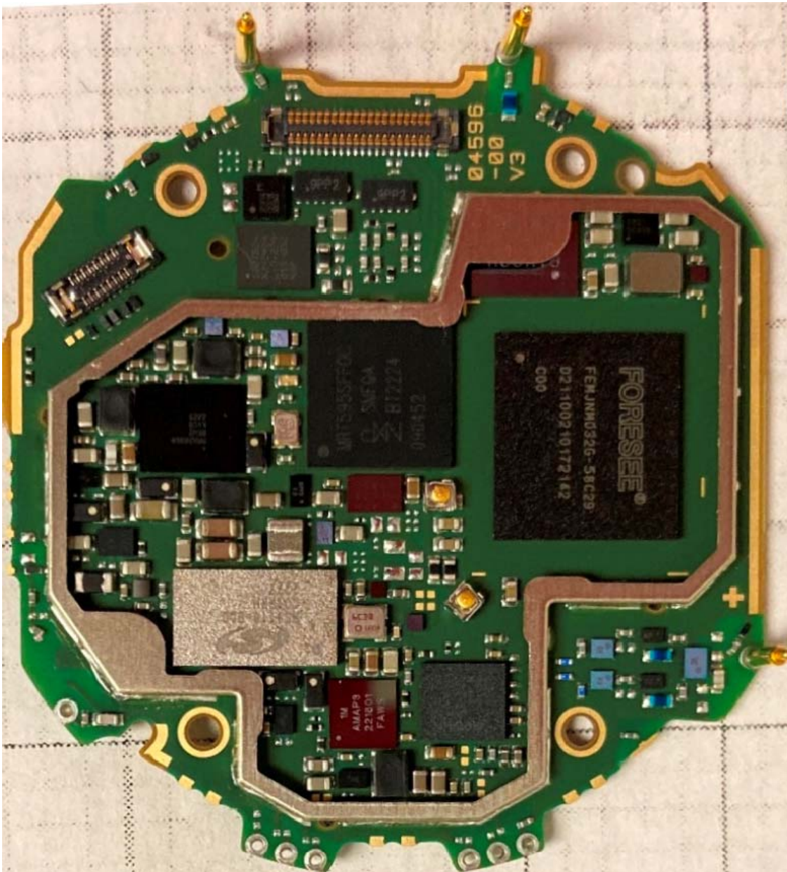
Figure E15.6 – Internal, PCB Top Side, Shield Removed
