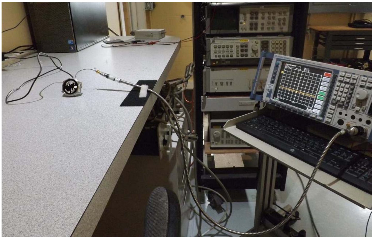
Figure E16.1 – Setup, Conducted Measurements
