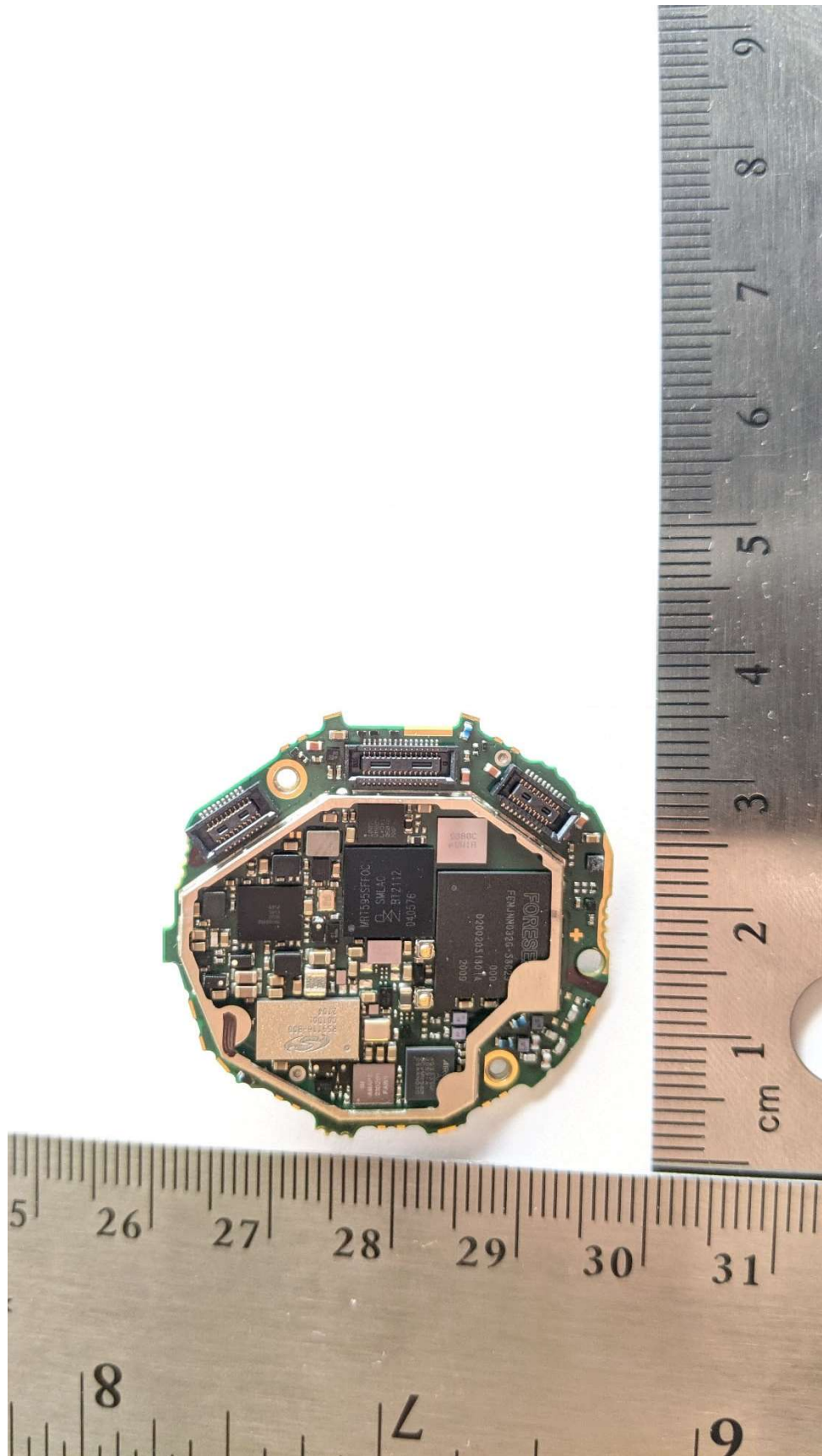
Front face of main PCB, shield removed
