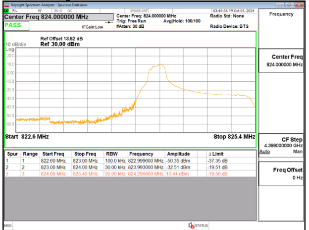
Band Edge_Band26_1.4MHz_PUSCH_824.7MHz_Chain0
