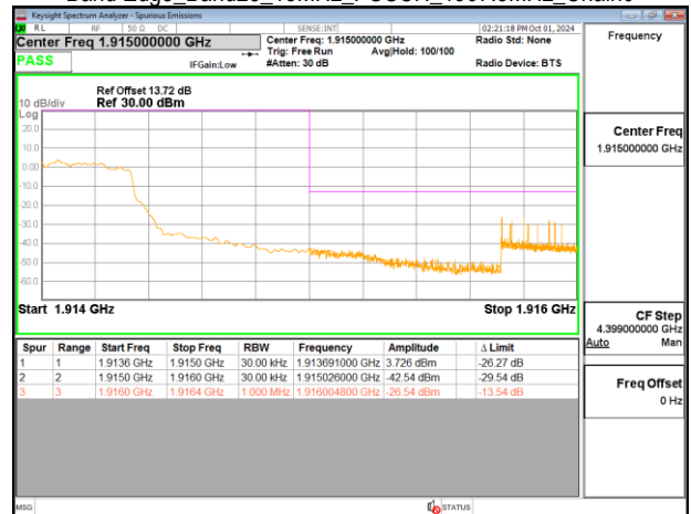
Band Edge_Band25_15MHz_PUSCH_1907.5MHz_Chain0
