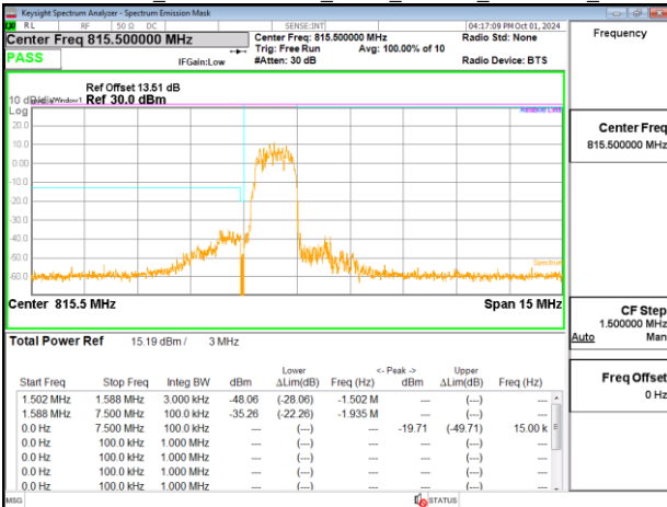
Emission Mask_Band26-Part90s_3MHz_PUSCH_815.5MHz_Chain0
