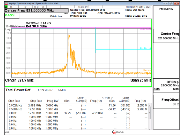
Emission Mask_Band26-Part90s_5MHz_PUSCH_821.5MHz_Chain0
