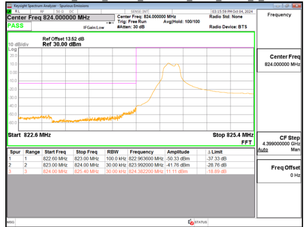
Band26_3MHz_Chain0_825.5MHz_NBI 0_QPSK_6_0
