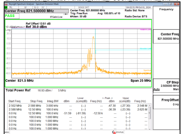
Emission Mask_Band26-Part90s_5MHz_PUSCH_821.5MHz_Chain0
