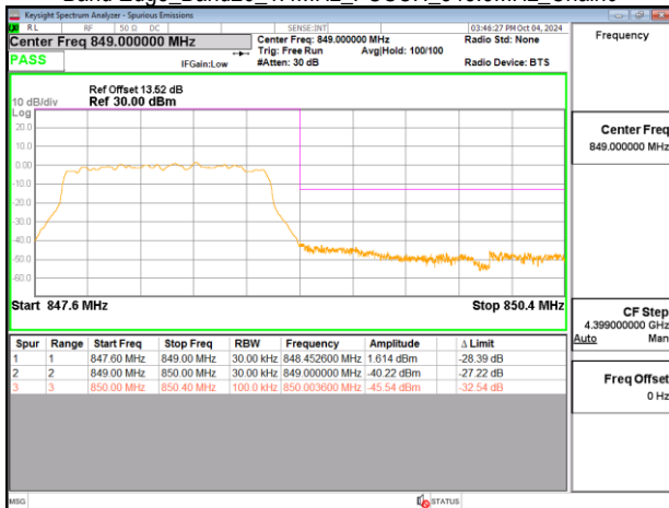
Band Edge_Band26_1.4MHz_PUSCH_848.3MHz_Chain0
