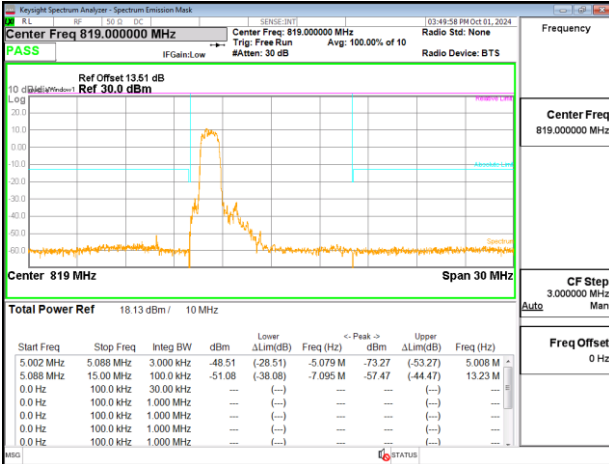
Emission Mask_Band26-Part90s_10MHz_PUSCH_819MHz_Chain0
