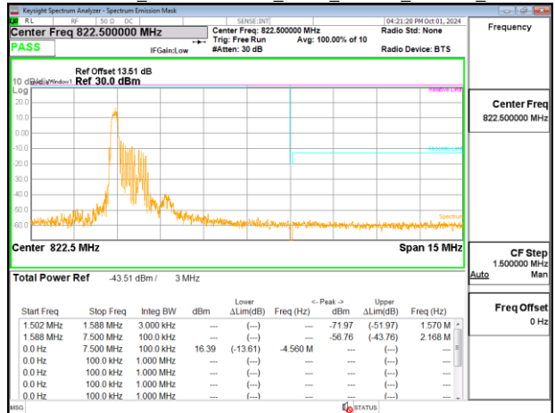
Emission Mask_Band26-Part90s_3MHz_PUSCH_819MHz_Chain0
