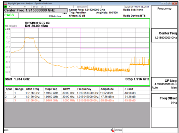
Band Edge_Band25_15MHz_PUSCH_1907.5MHz_Chain0
