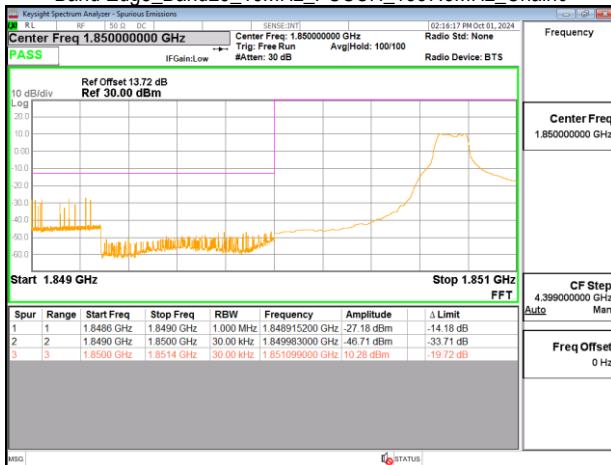
Band Edge_Band25_15MHz_PUSCH_1857.5MHz_Chain0
