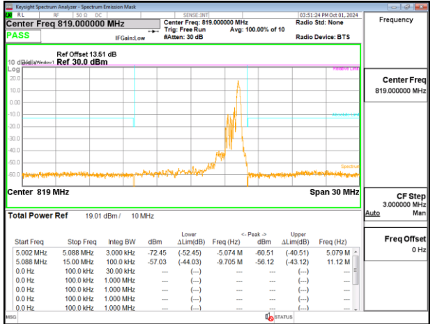
Emission Mask_Band26-Part90s_10MHz_PUSCH_819MHz_Chain0
