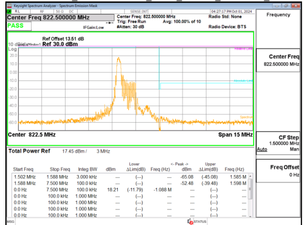
Emission Mask_Band26-Part90s_3MHz_PUSCH_822.5MHz_Chain0
