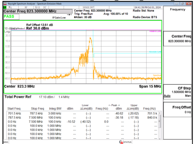
Emission Mask_Band26-Part90s_1.4MHz_PUSCH_823.3MHz_Chain0
