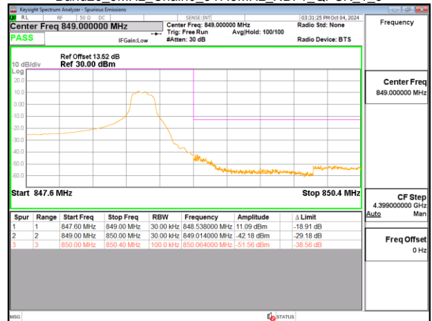
Band26_3MHz_Chain0_847.5MHz_NBI 1_QPSK_1_5
