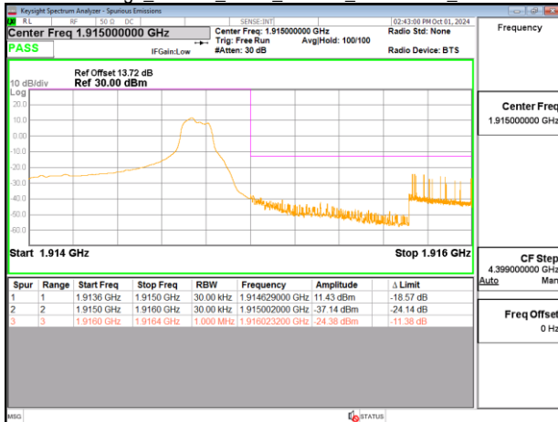
Band Edge_Band25_5MHz_PUSCH_1912.5MHz_Chain0
