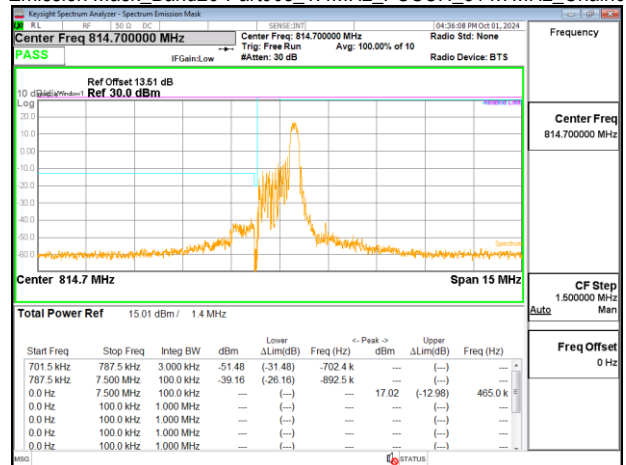
Emission Mask_Band26-Part90s_1.4MHz_PUSCH_814.7MHz_Chain0
