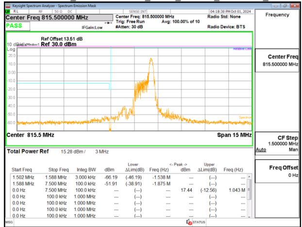
Emission Mask_Band26-Part90s_3MHz_PUSCH_815.5MHz_Chain0
