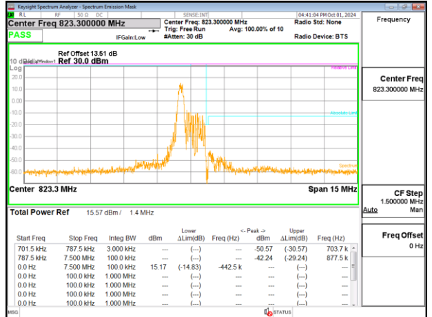
Emission Mask_Band26-Part90s_1.4MHz_PUSCH_823.3MHz_Chain0
