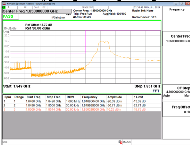
Band Edge_Band25_5MHz_PUSCH_1852.5MHz_Chain0
