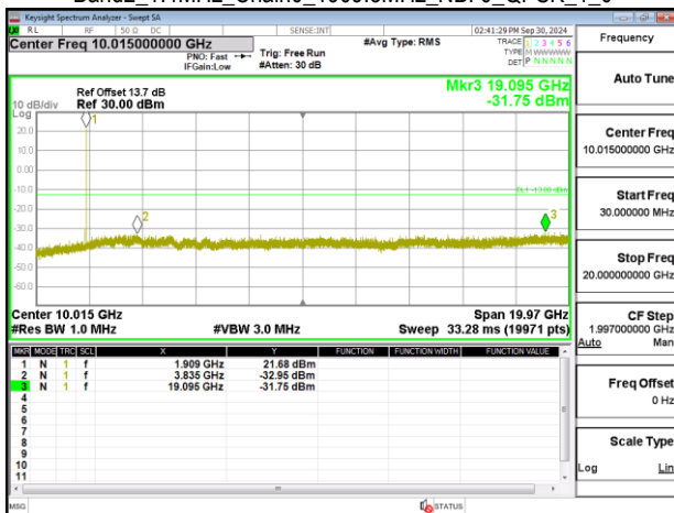
Band2_1.4MHz_Chain0_1909.3MHz_NBI_0_QPSK_1_0
