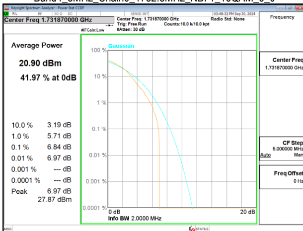
Band4_5MHz_Chain0_1732.5MHz_NBI 1_16QAM_6_0
