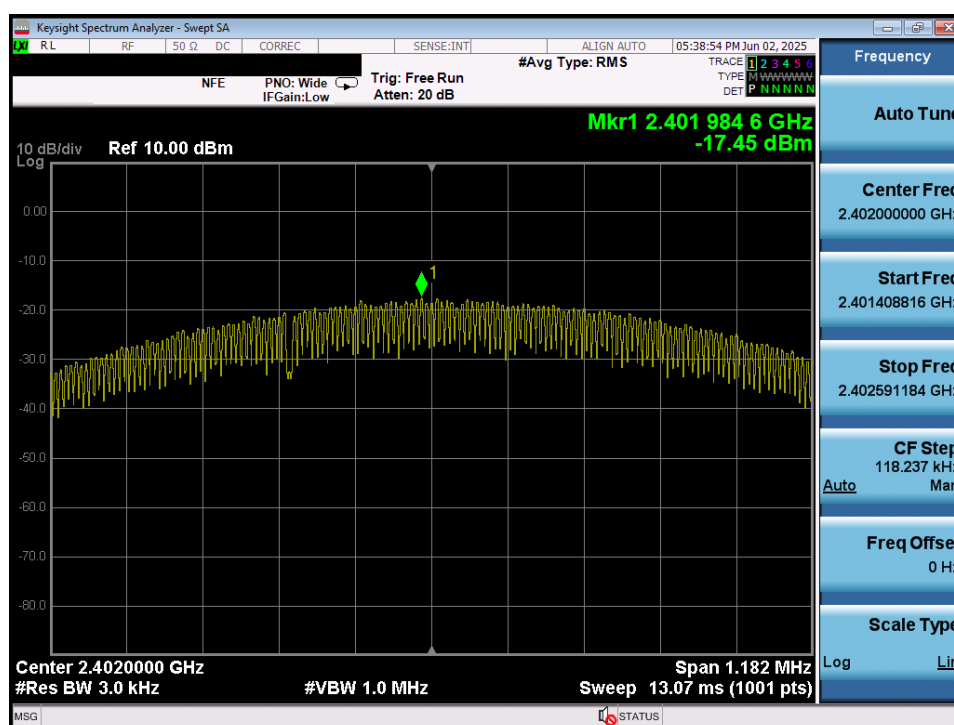
Plot 7-12. Power Spectral Density Plot (ANT+ – Ch. 0)
