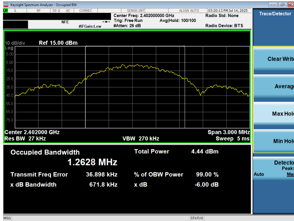
Plot 7-4. Occupied Bandwidth Plot (ANT+ – Ch. 0)
