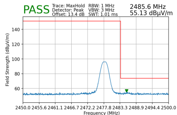
Plot 7-30. Radiated Restricted Upper Band Edge Measurement (Peak)
