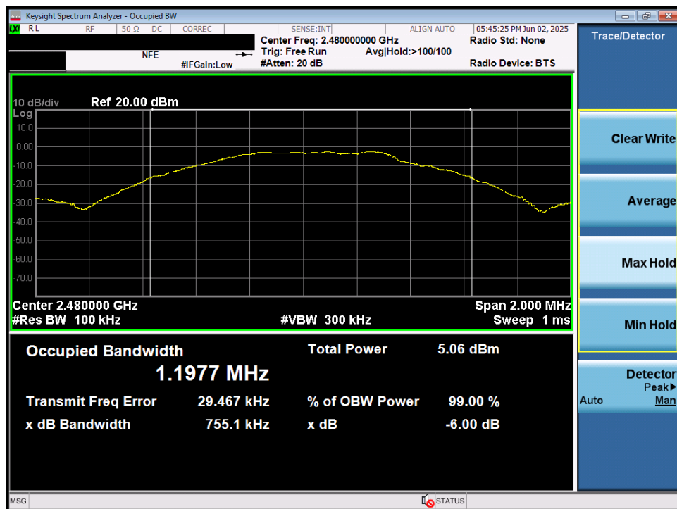
Plot 7-3. 6dB Bandwidth Plot (ANT+ – Ch. 78)
