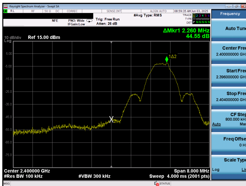
Plot 7-15. Band Edge Plot (ANT+ – Ch. 0)
