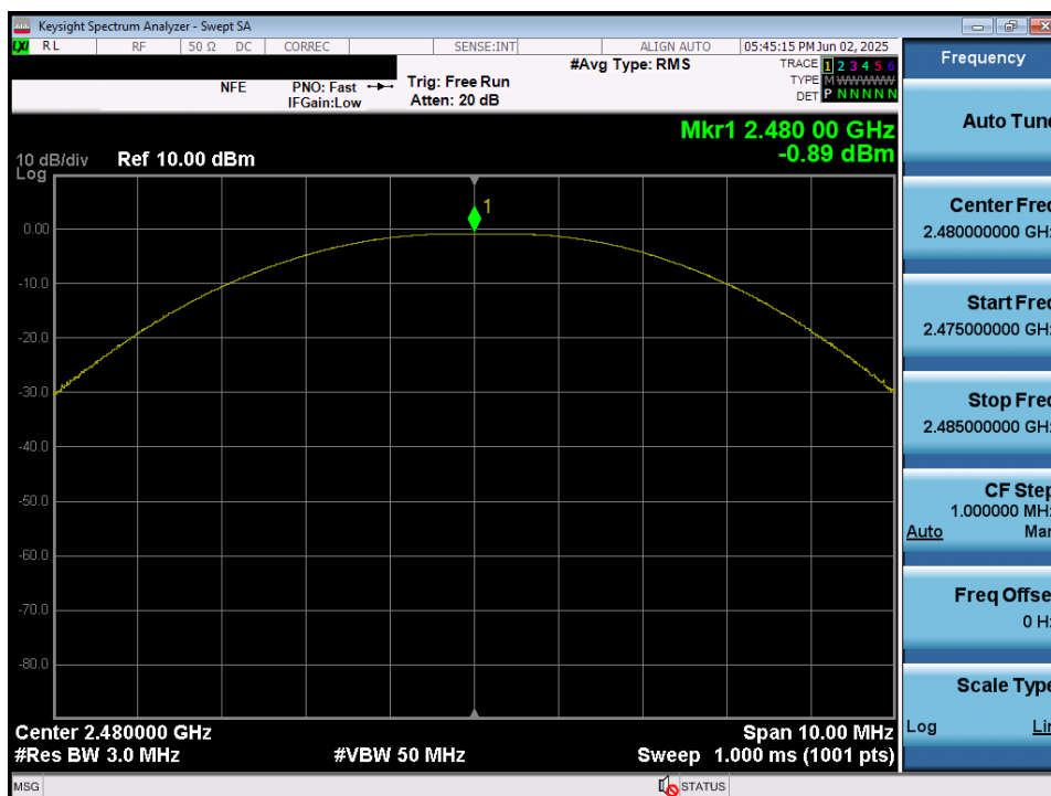
Plot 7-11. Peak Power Plot (ANT+ – Ch. 78)
