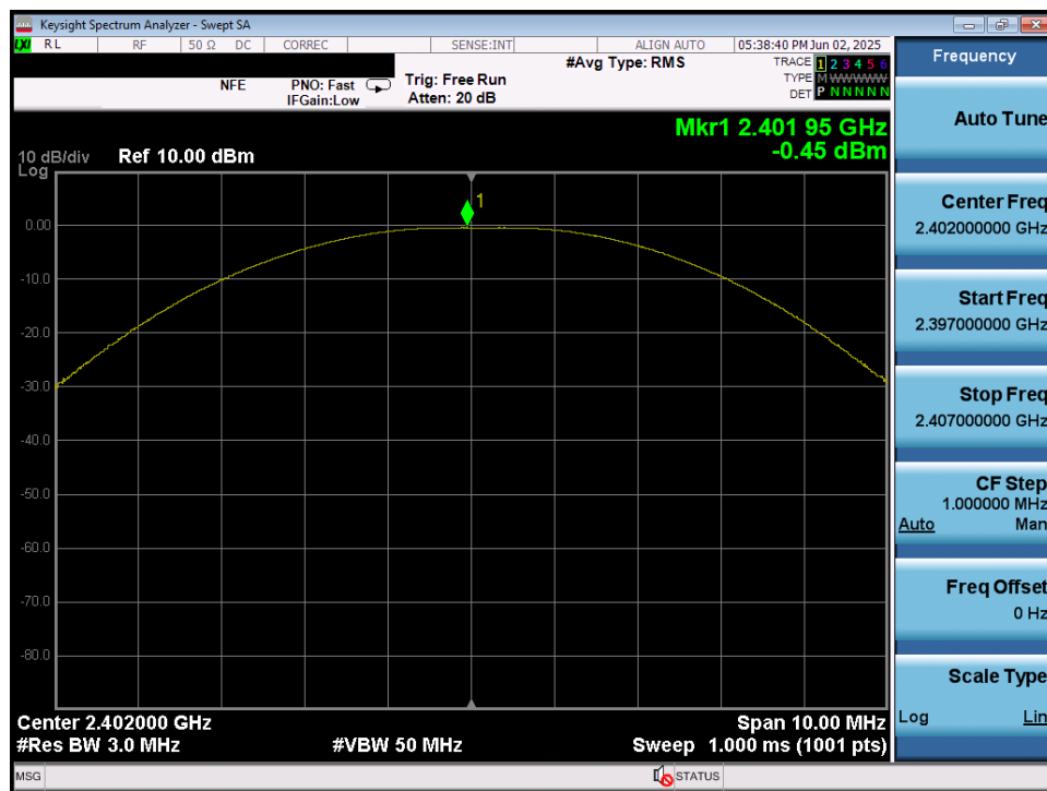
Plot 7-7. Peak Power Plot (ANT+ – Ch. 0)
