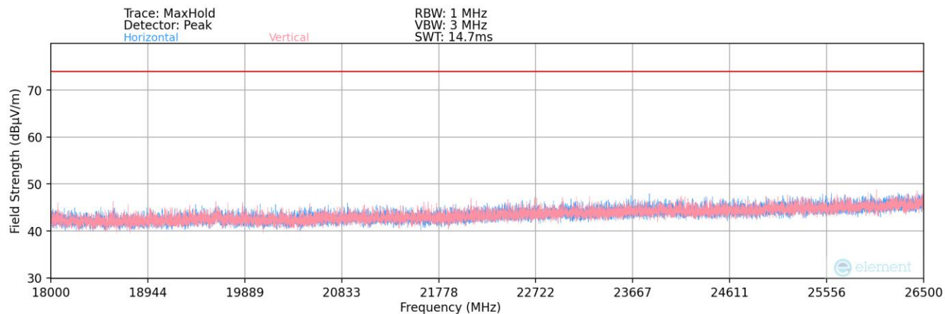
Plot 7-28. Radiated Spurious Plot above 18GHz (ANT+ – Ch. 39)
