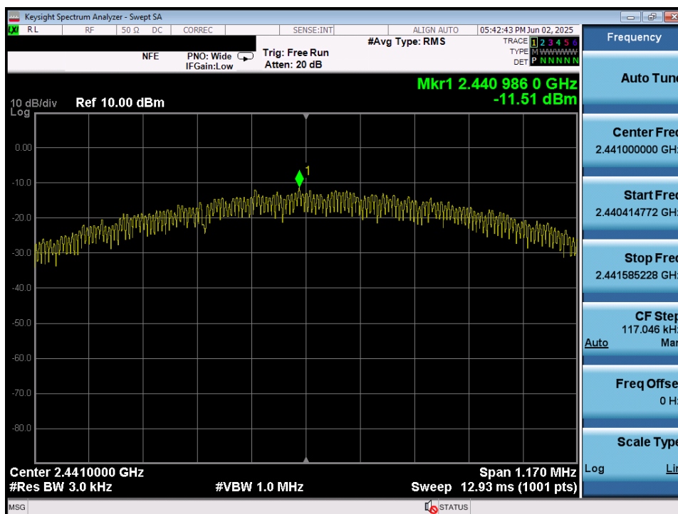
Plot 7-13. Power Spectral Density Plot (ANT+ – Ch. 39)
