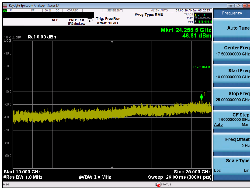
Plot 7-20. Conducted Spurious Plot (ANT+ – Ch. 0)
