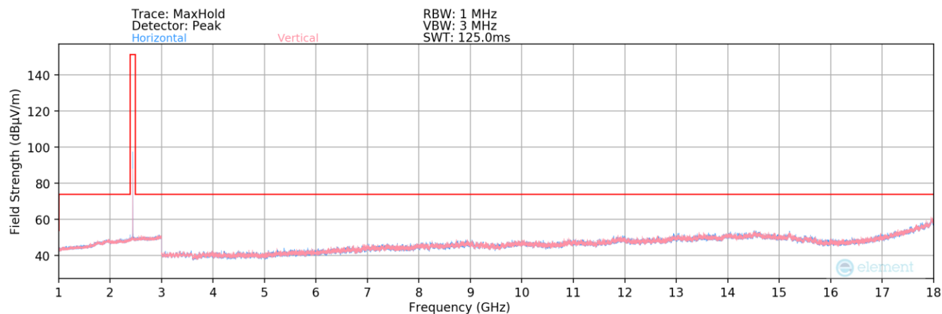
Plot 7-26. Radiated Spurious Plot above 1GHz (ANT+ – Ch. 39)
