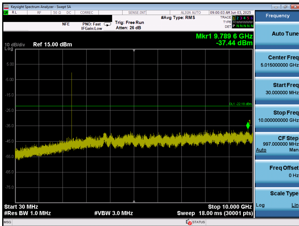
Plot 7-19. Conducted Spurious Plot (ANT+ – Ch. 0)
