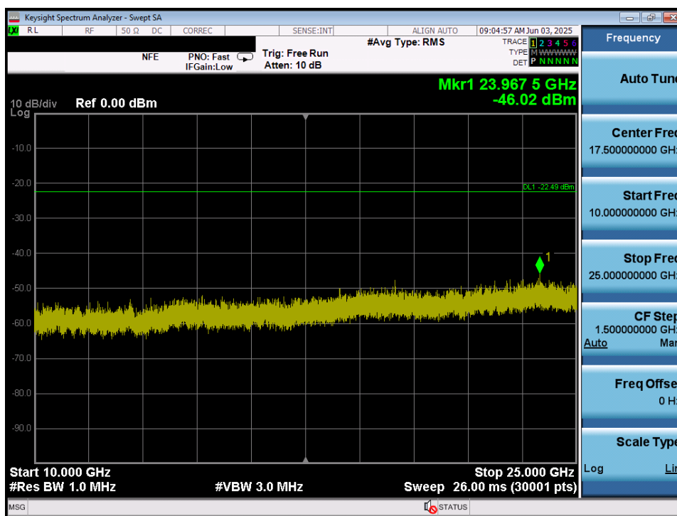
Plot 7-24. Conducted Spurious Plot (ANT+ – Ch. 78)
