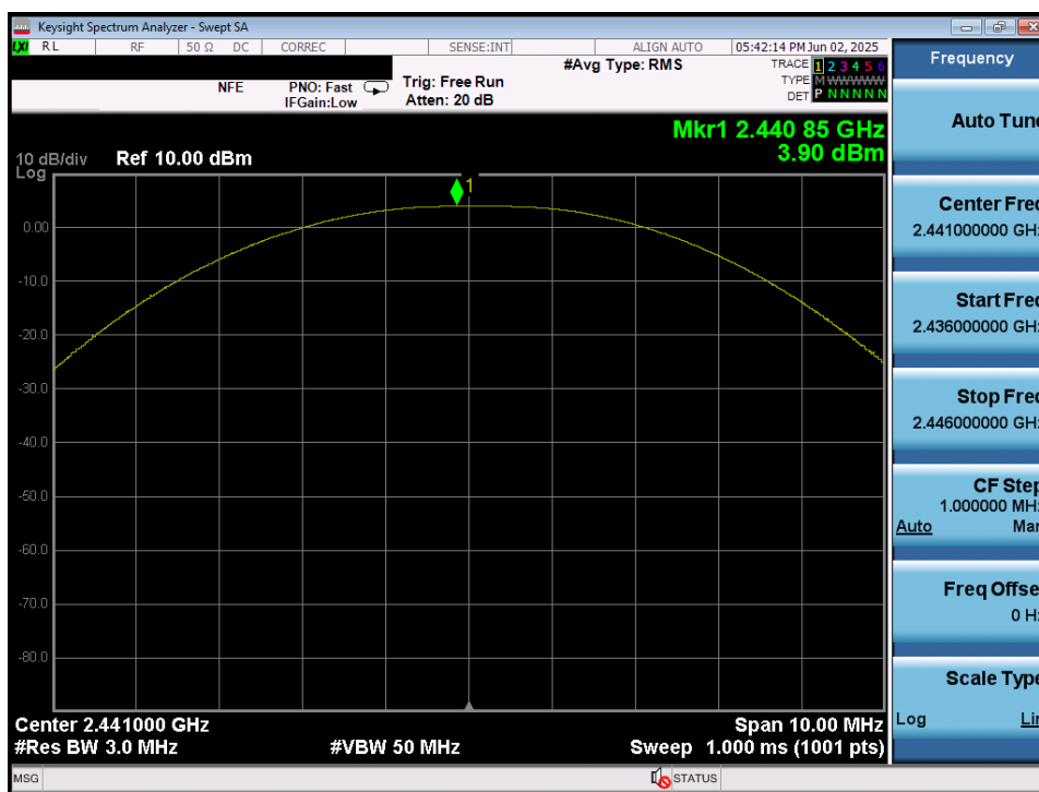
Plot 7-9. Peak Power Plot (ANT+ – Ch. 39)
