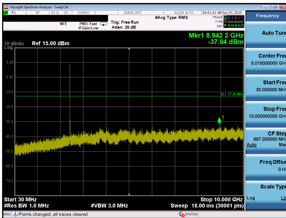
Plot 7-21. Conducted Spurious Plot (ANT+ – Ch. 39)
