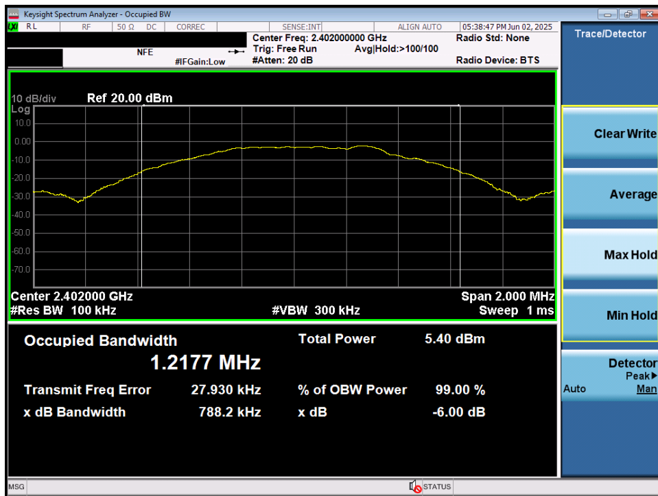
Plot 7-1. 6dB Bandwidth Plot (ANT+ – Ch. 0)
