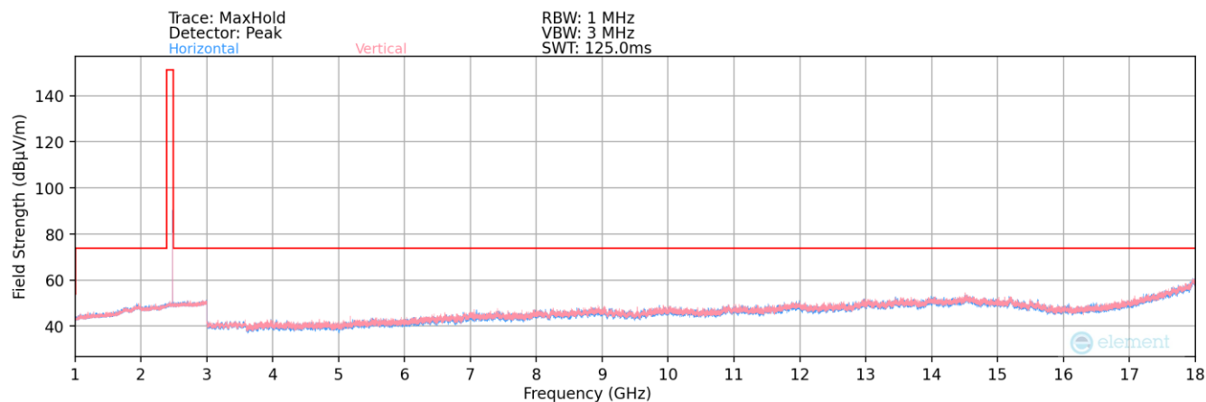
Plot 7-27. Radiated Spurious Plot above 1GHz (ANT+ – Ch. 78)
