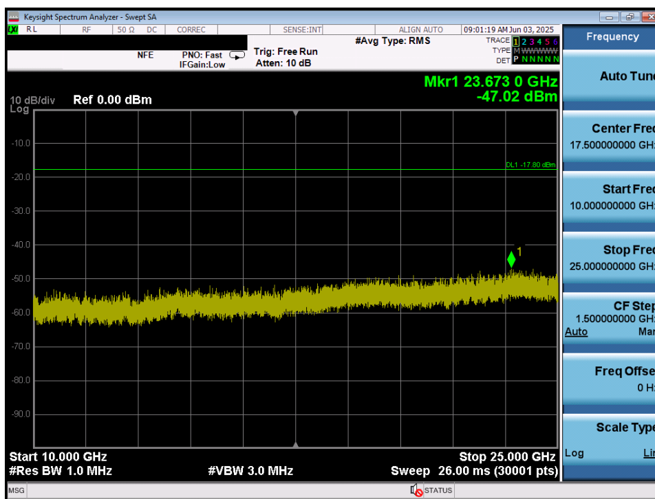
Plot 7-22. Conducted Spurious Plot (ANT+ – Ch. 39)
