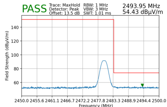
Plot 7-32. Radiated Restricted Upper Band Edge Measurement (Peak)
