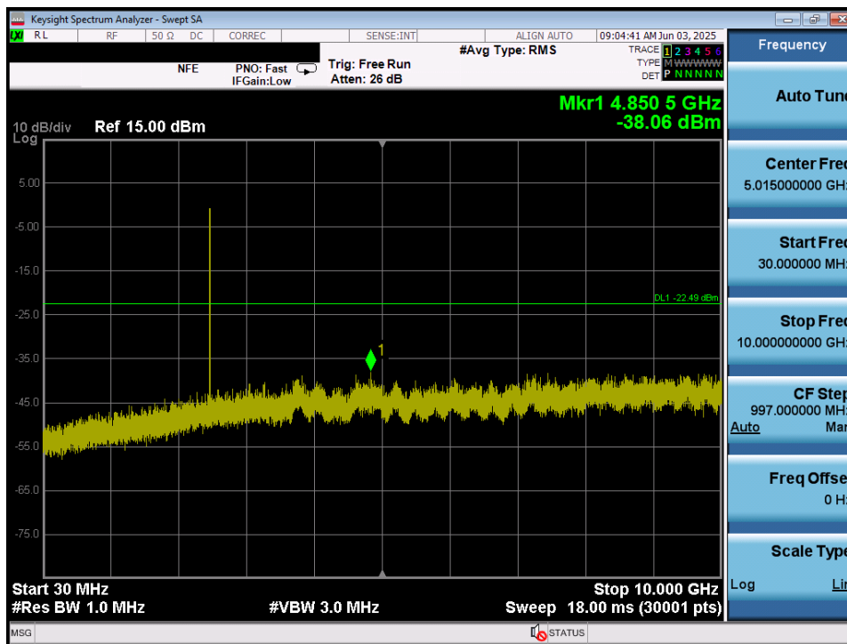
Plot 7-23. Conducted Spurious Plot (ANT+ – Ch. 78)
