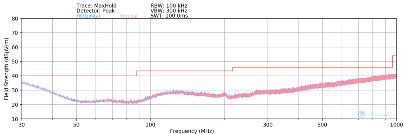
Plot 7-33. Radiated Spurious Plot below 1GHz
