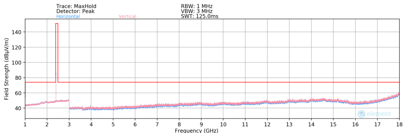
Plot 7-25. Radiated Spurious Plot above 1GHz (ANT+ – Ch. 0)
