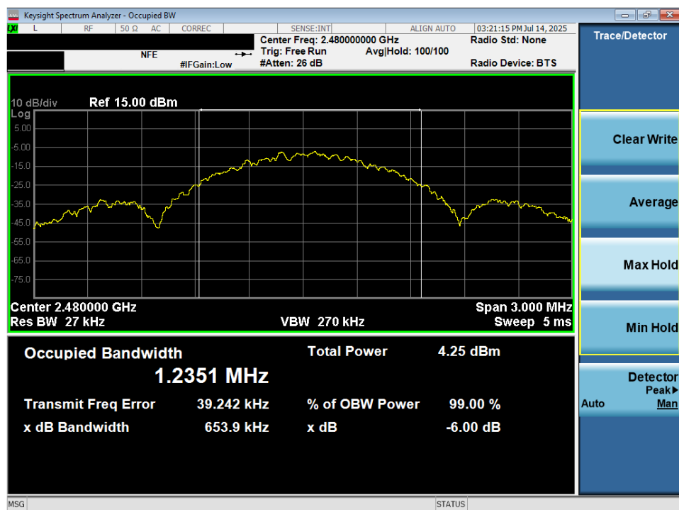
Plot 7-6. Occupied Bandwidth Plot (ANT+ – Ch. 78)
