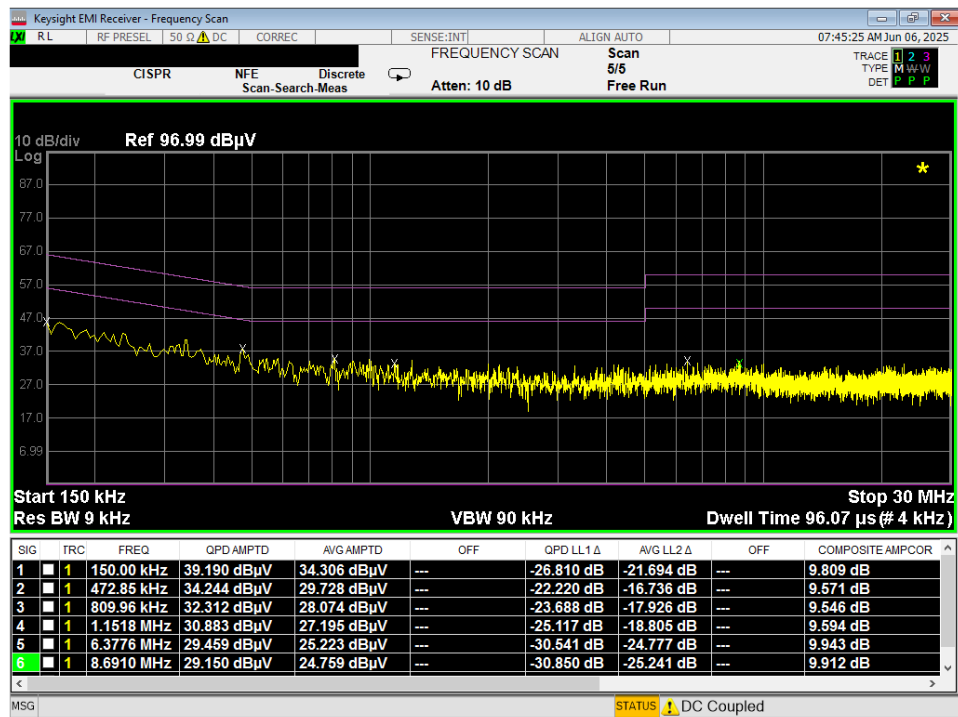
Plot 7-34. Line Conducted Plot with ANT+ (L1)
