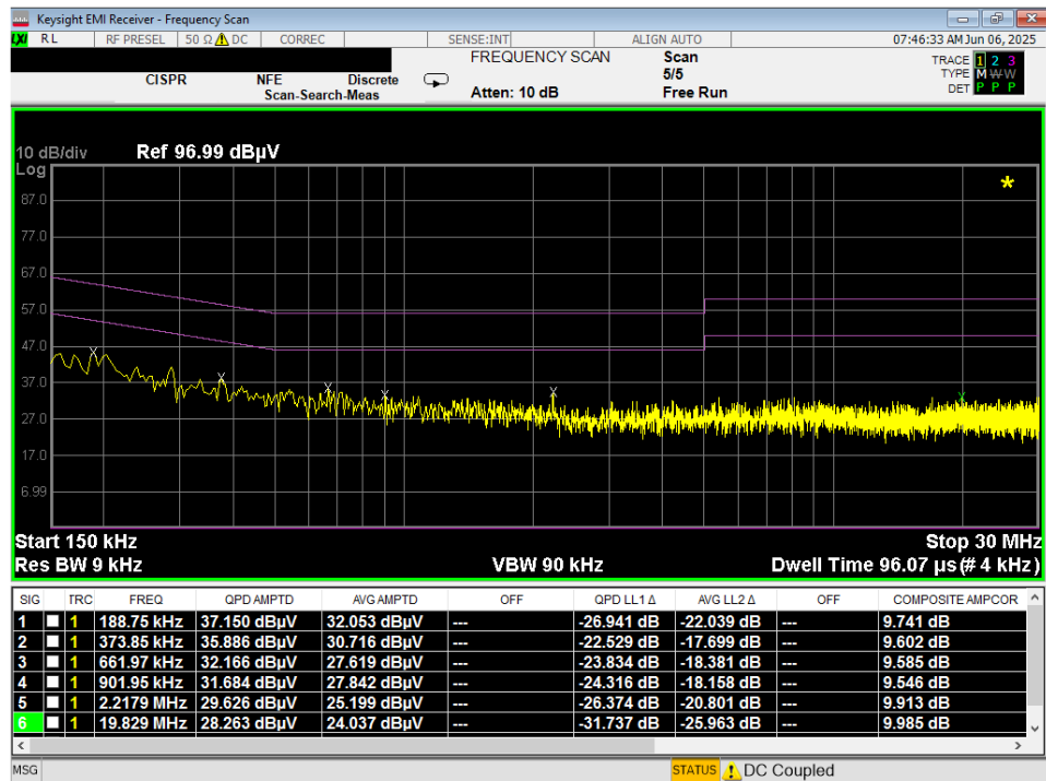
Plot 7-35. Line Conducted Plot with ANT+ (N)
