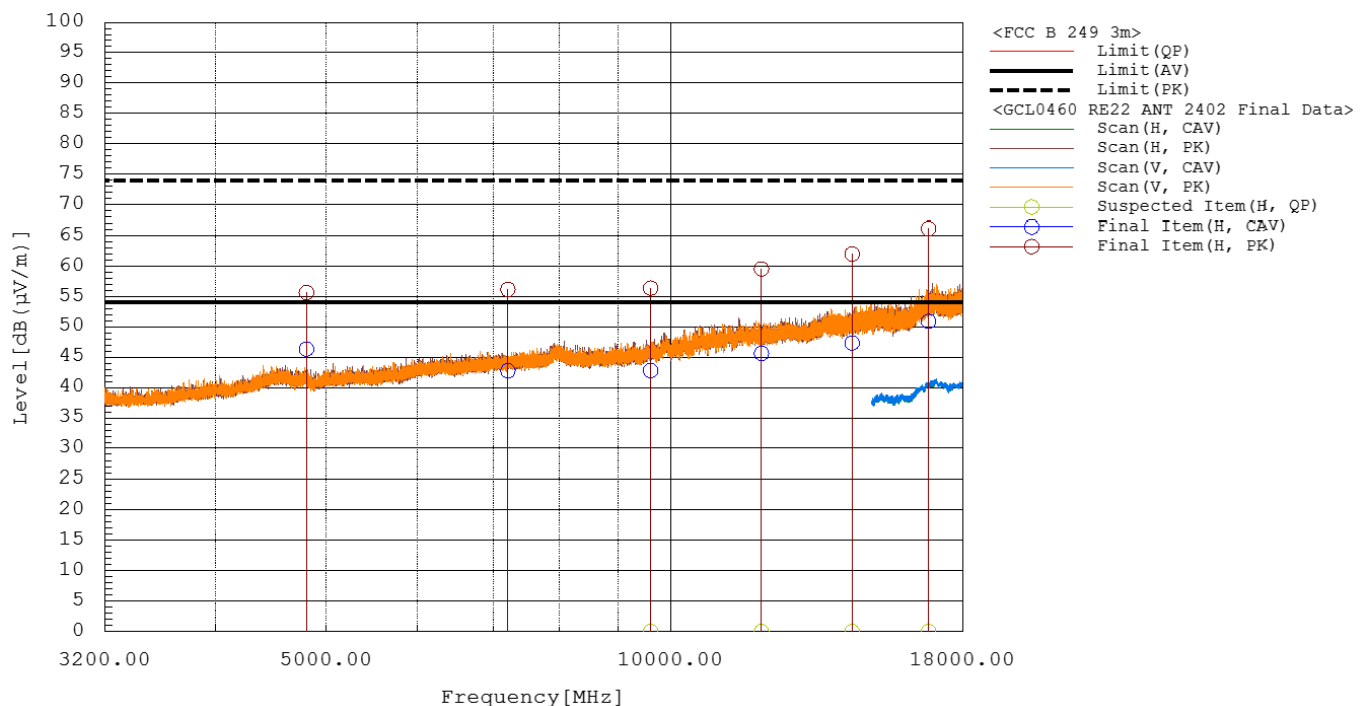
Figure RE22.1: Spectral data (ANT 2402MHz)
