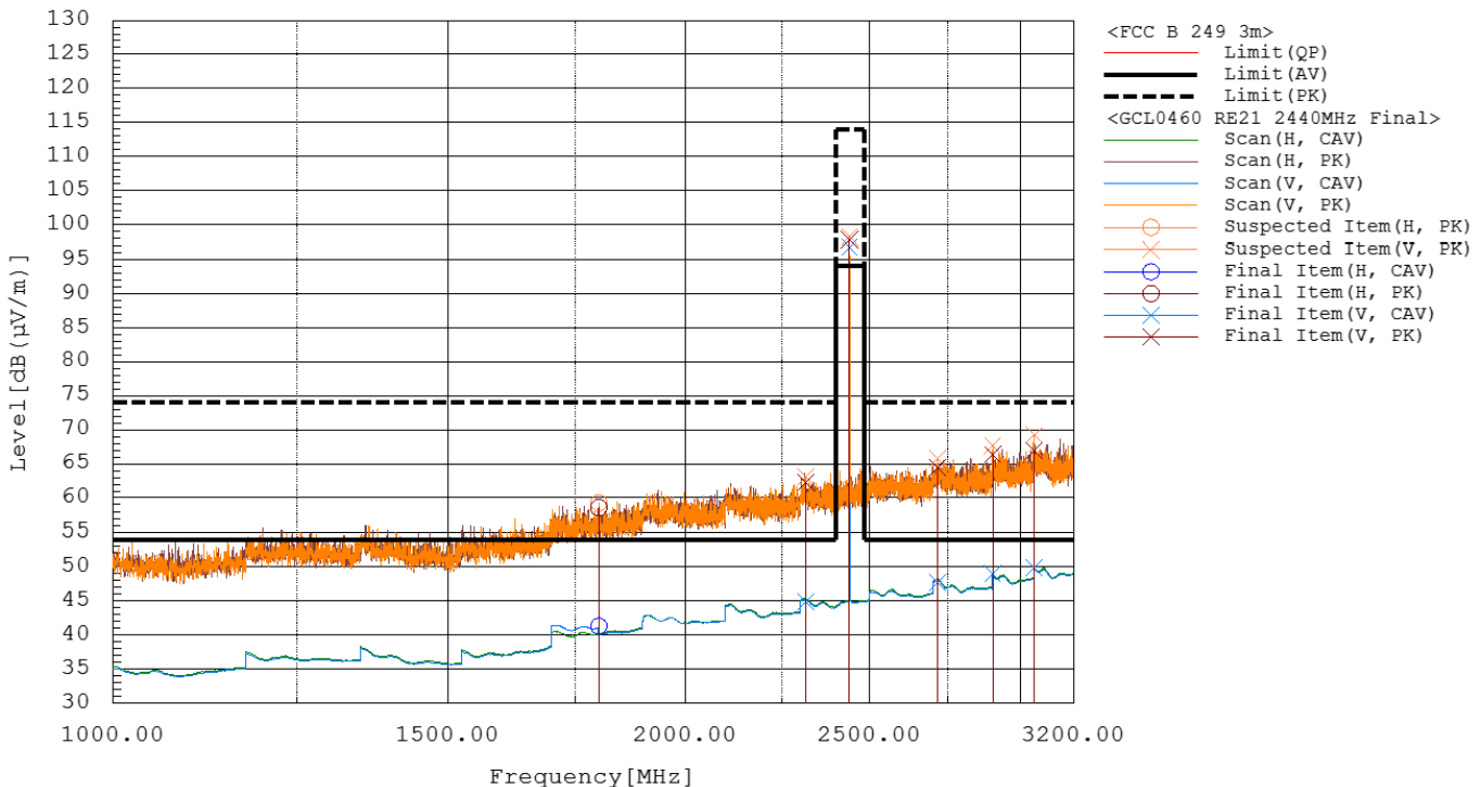
Figure RE21.2: Spectral data (Ant 2440MHz)
