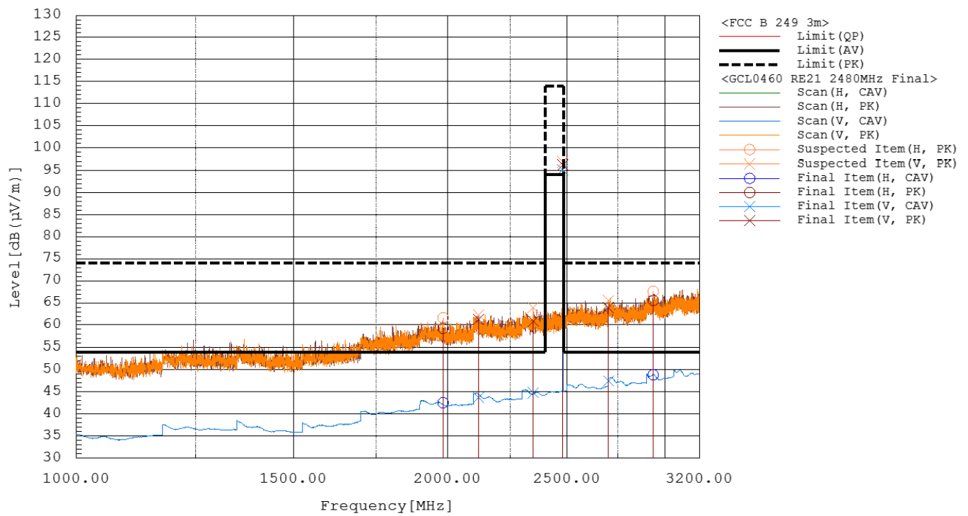
Figure RE21.3: Spectral data (Ant 2480MHz)
