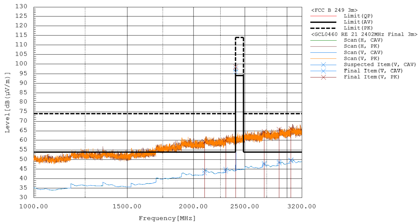
Figure RE21.1: Spectral data (Ant 2402MHz)
