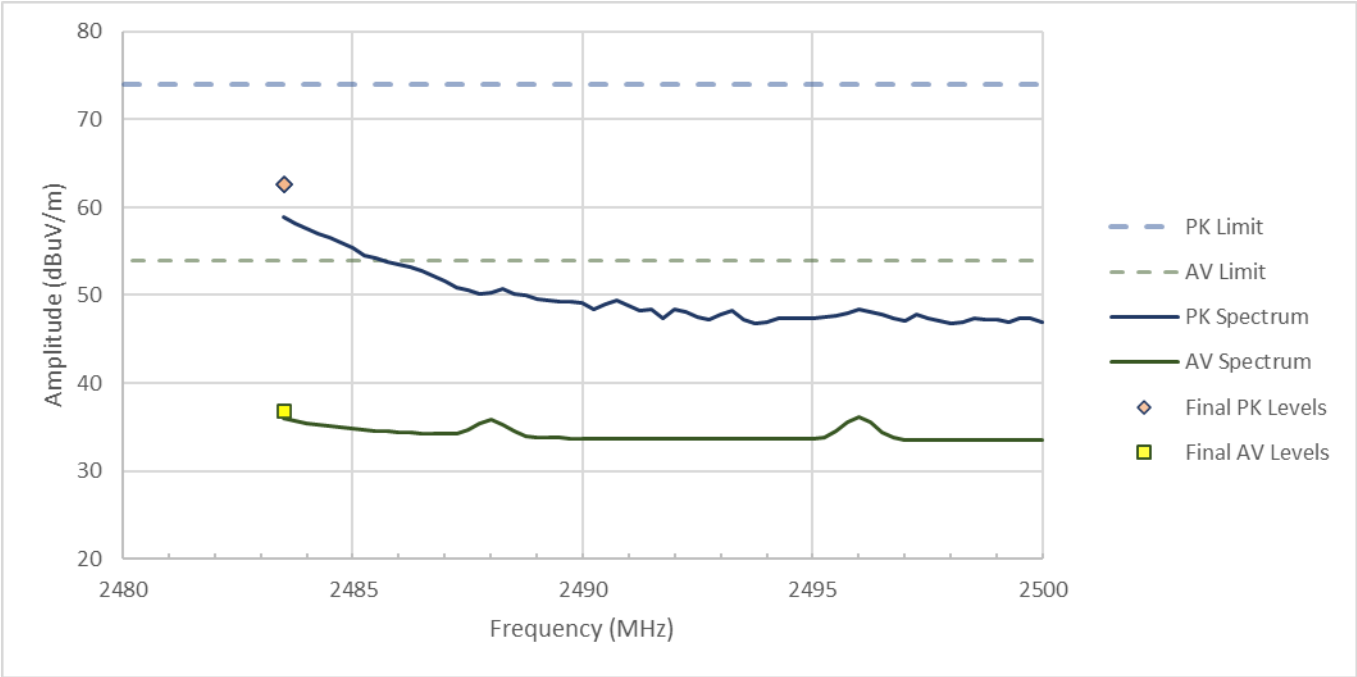
Figure RE04.2: FCC restricted band spectral data from 2483.5 to 2500 MHz (ANT)
