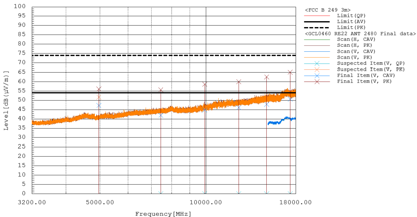
Figure RE22.3: Spectral data (ANT 2480MHz)
