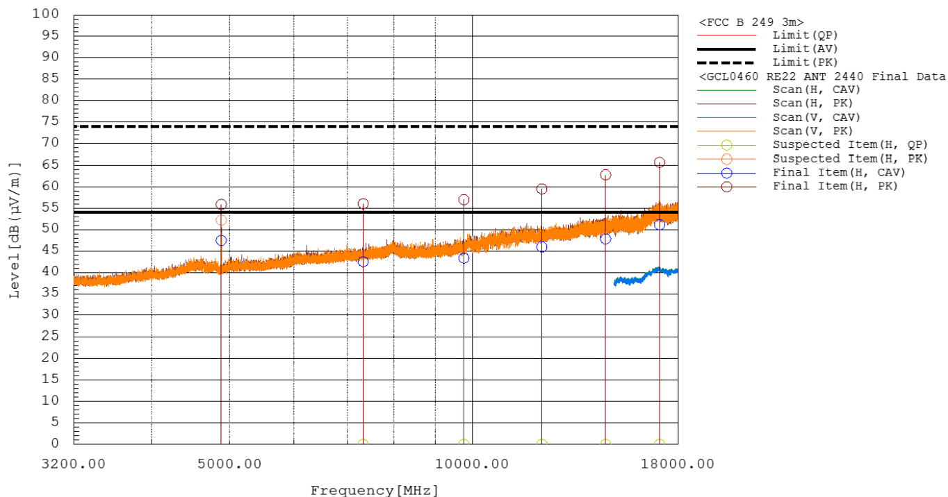
Figure RE22.2: Spectral data (ANT 2440MHz)
