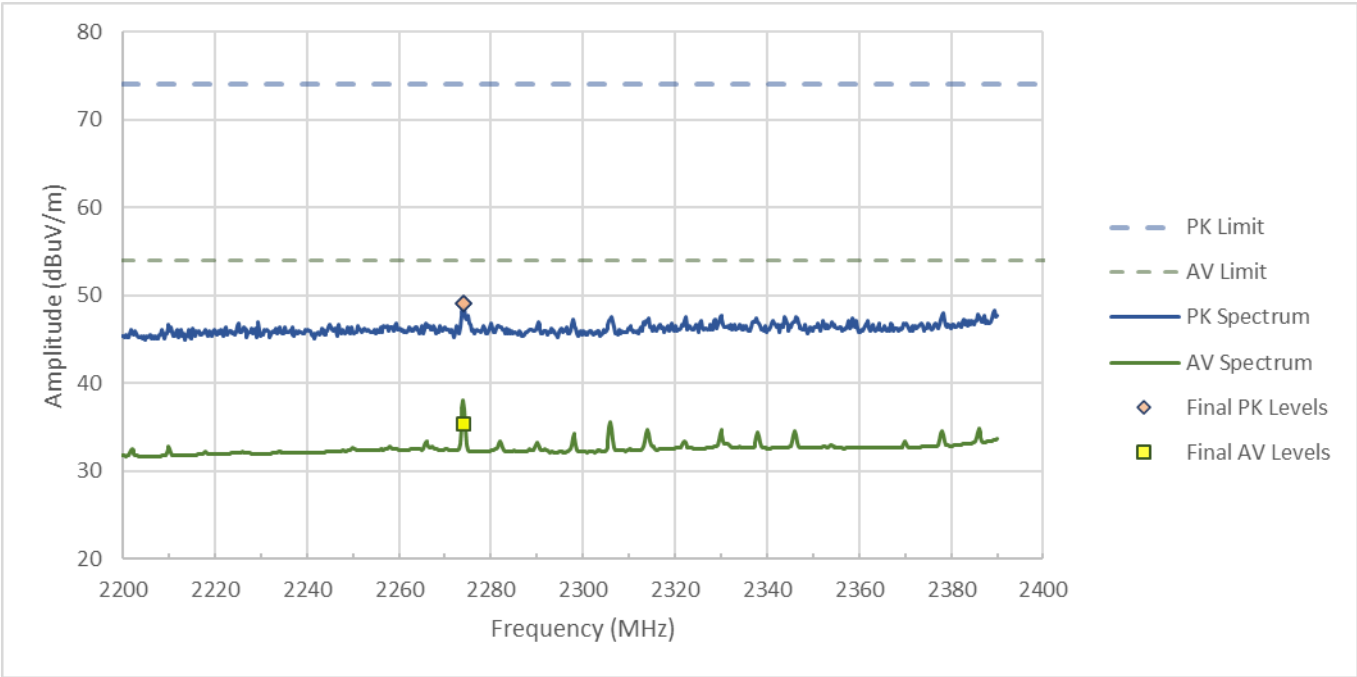
Figure RE04.1: FCC restricted band spectral data from 2200 to 2390 MHz (ANT)
