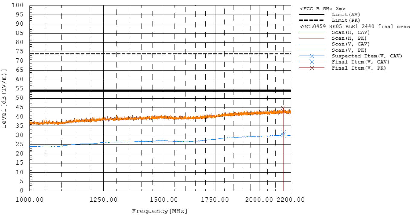
Figure RE05.2: Spectral data (BLE 1 Mbps 2440MHz)
