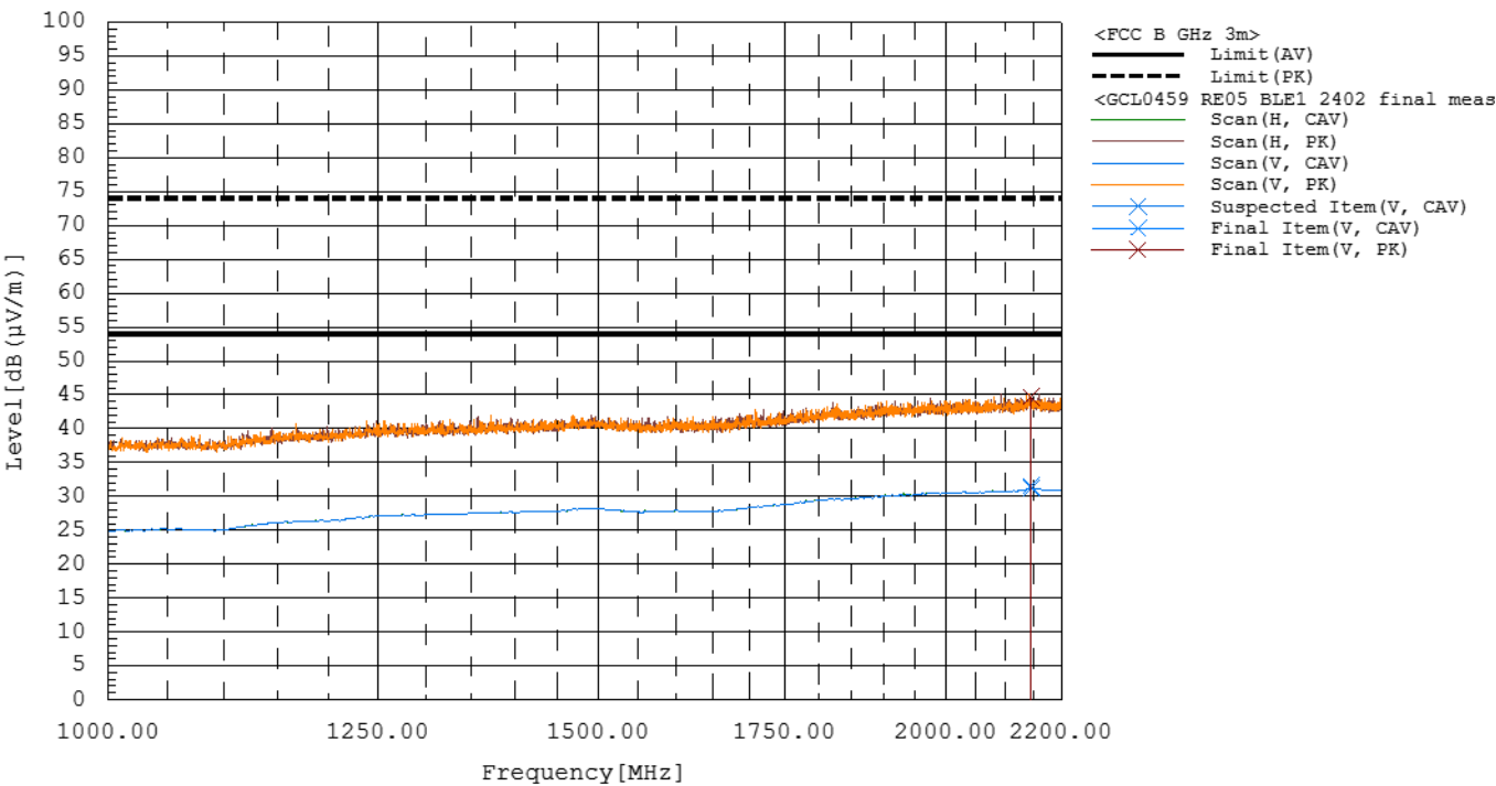
Figure RE05.1: Spectral data (BLE 1 Mbps 2402MHz)
