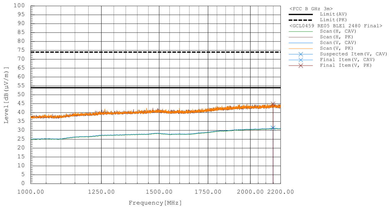
Figure RE05.3: Spectral data (BLE 1 Mbps 2480MHz)
