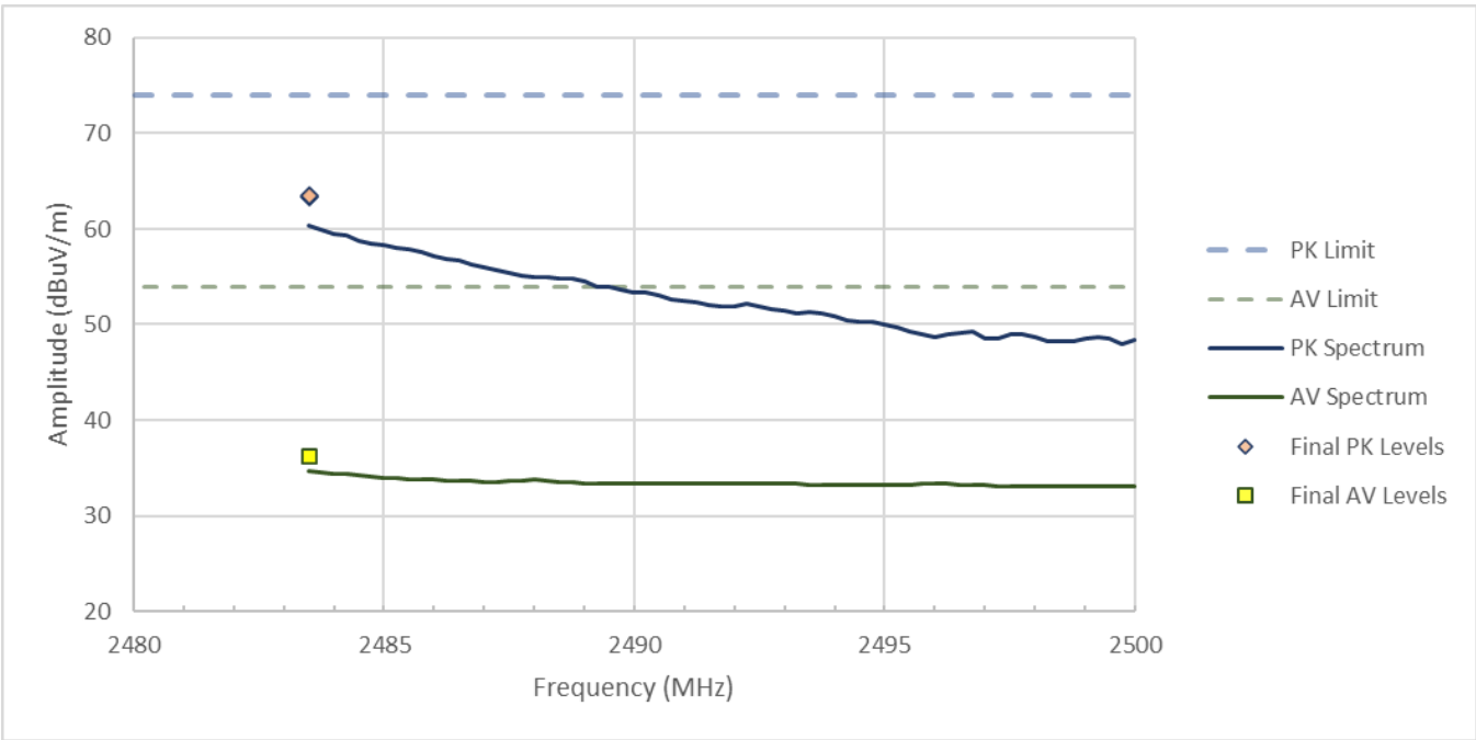
Figure RE03.2: FCC restricted band spectral data from 2483.5 to 2500 MHz (BLE 1Mb/s)
