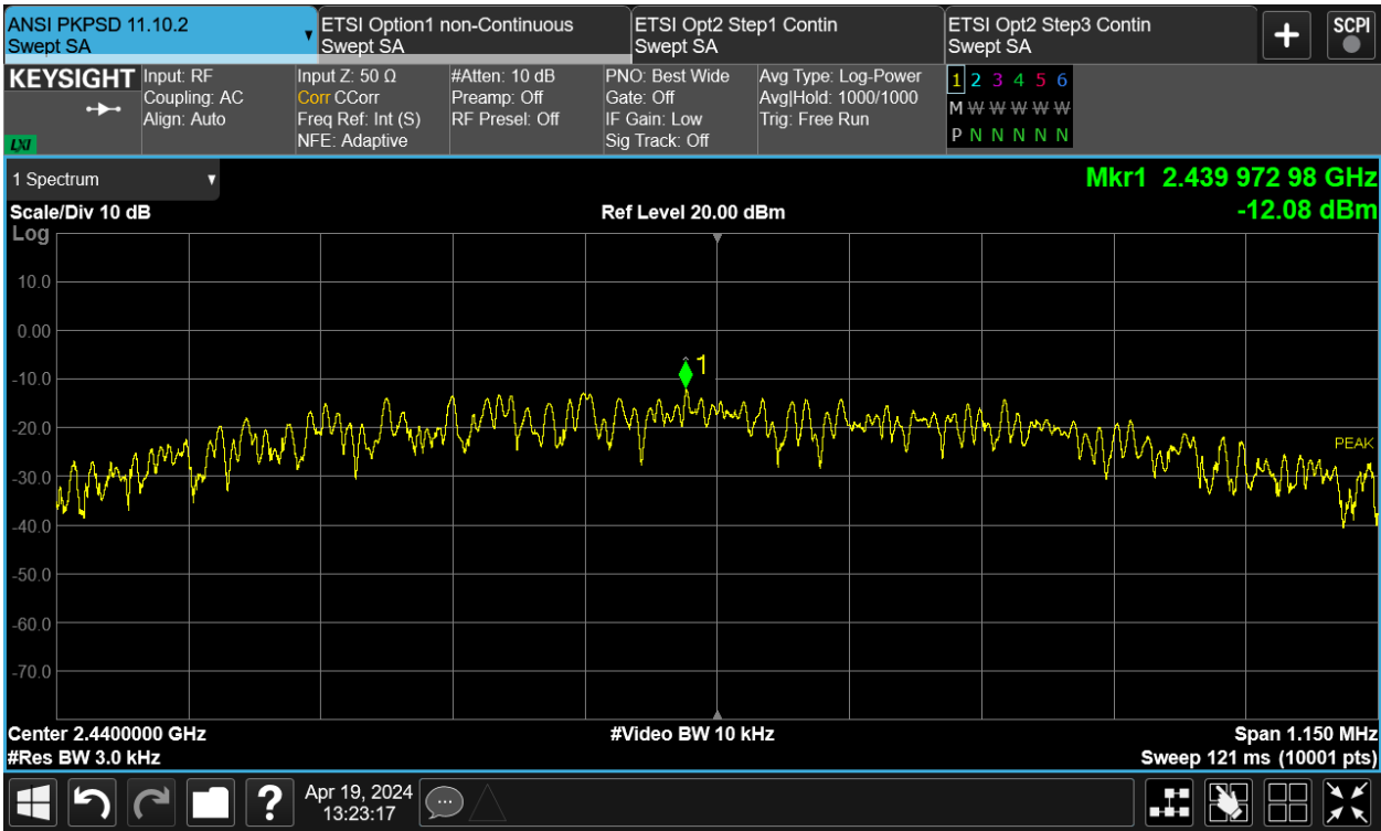
Figure TR19.2: Test data for BLE 1 Mbps, 2440 MHz
