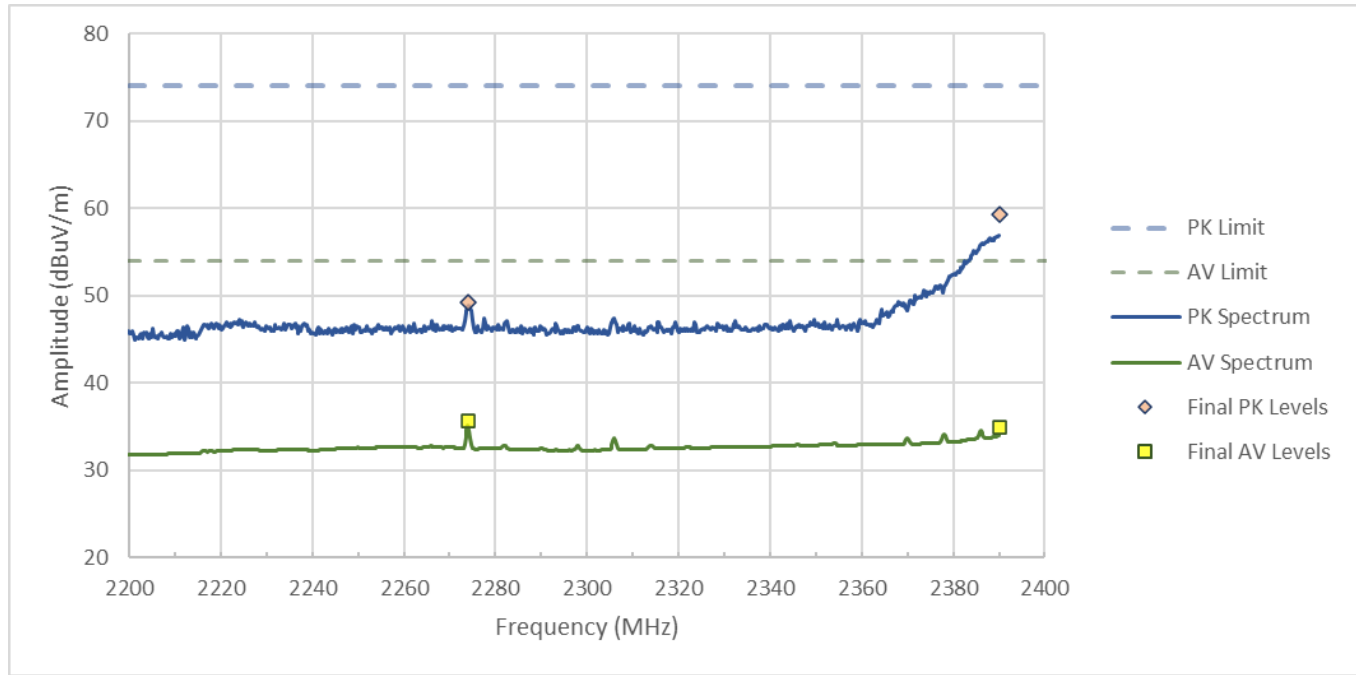
Figure RE03.1: FCC restricted band spectral data from 2200 to 2390 MHz (BLE 1Mb/s)
