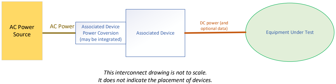
Figure 1: Block diagram of equipment for arrangements A2, A3, A4
