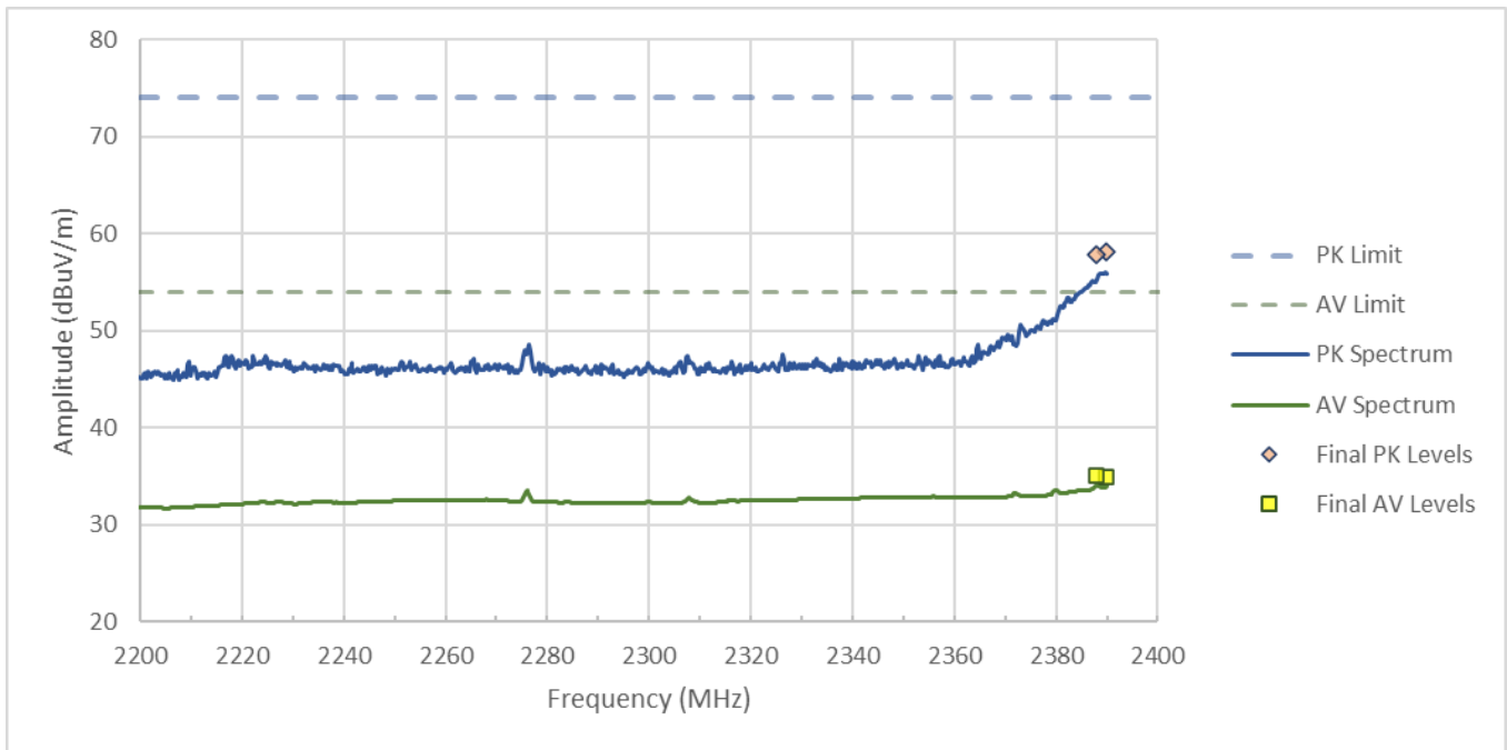
Figure RE03.3: FCC restricted band spectral data from 2200 to 2390 MHz (BLE 2Mb/s)
