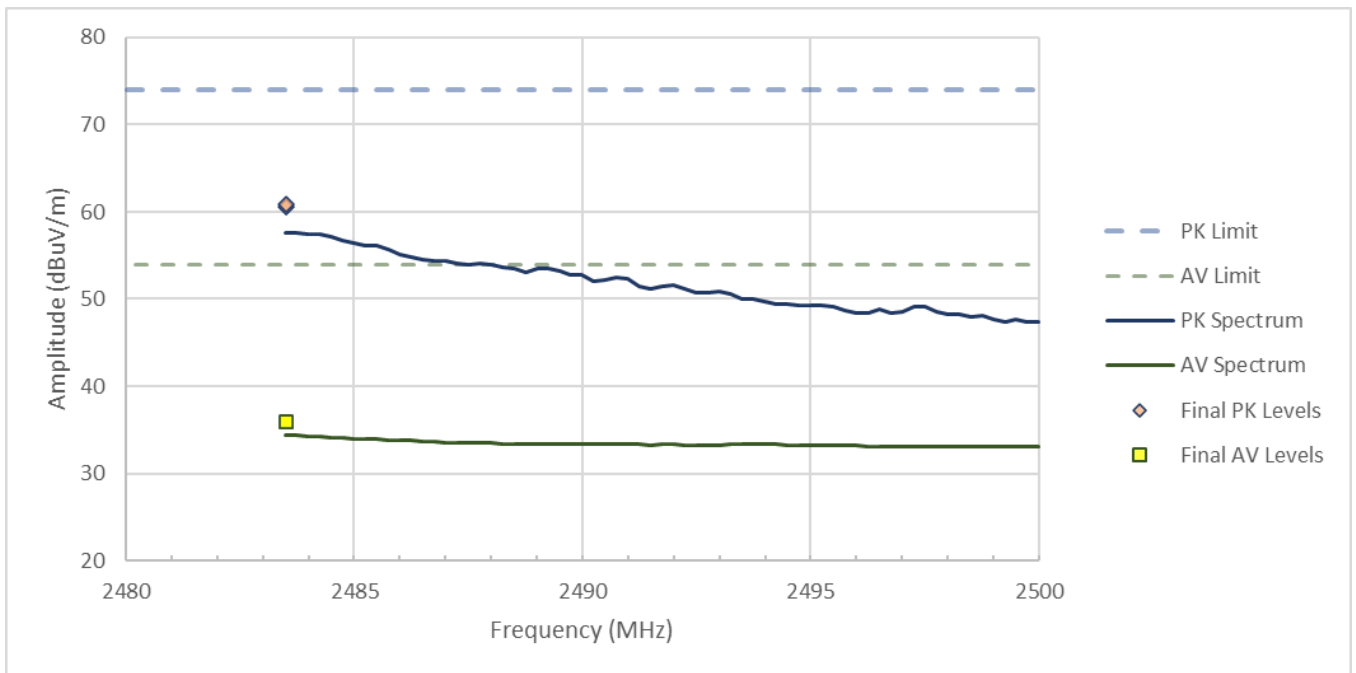
Figure RE03.4: FCC restricted band spectral data from 2483.5 to 2500 MHz (BLE 2Mb/s)
