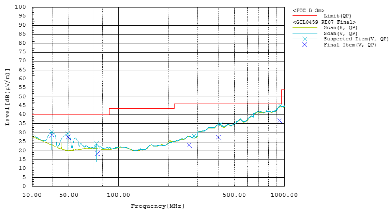
Figure RE07.1: Spectral data
