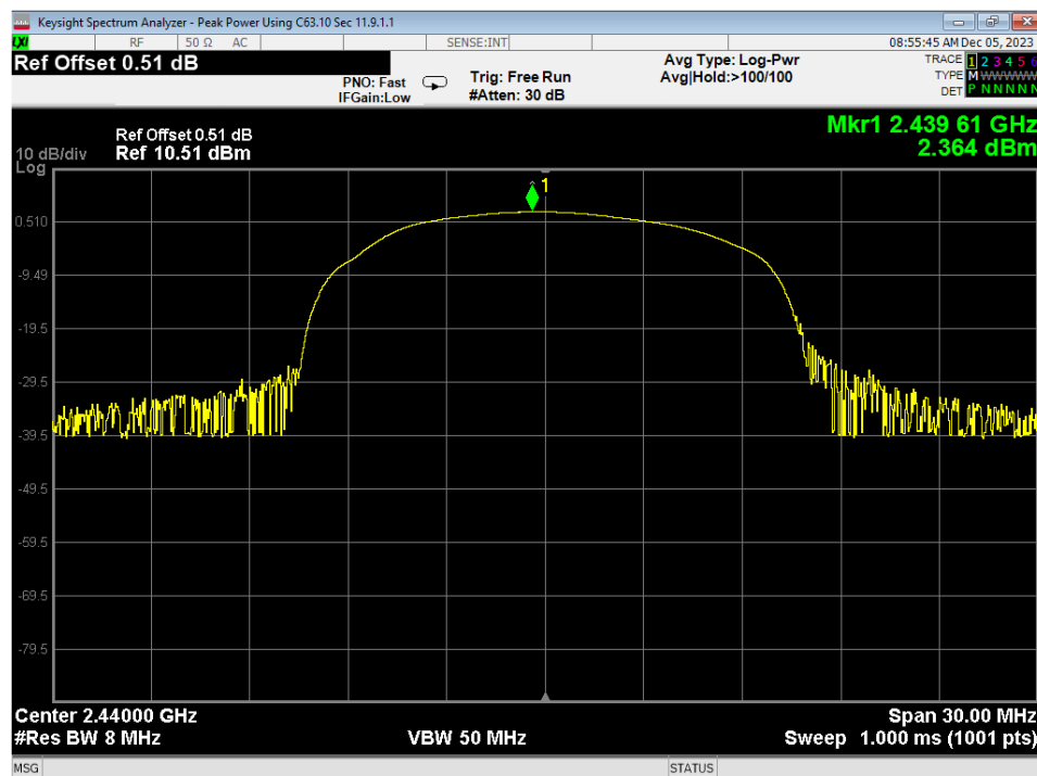
Figure 3 – Conducted Peak Power Measurement, GFSK
