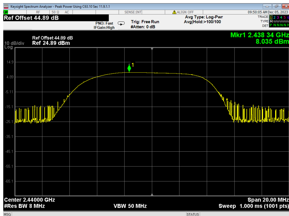
Figure 4 – Radiated Peak Power Measurement, GFSK
