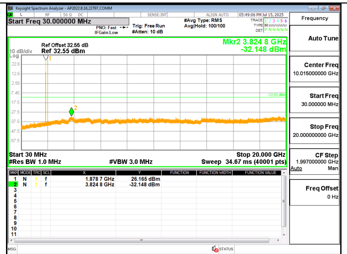
LTE2 5MHz QPSK MID Ch RB1-0
