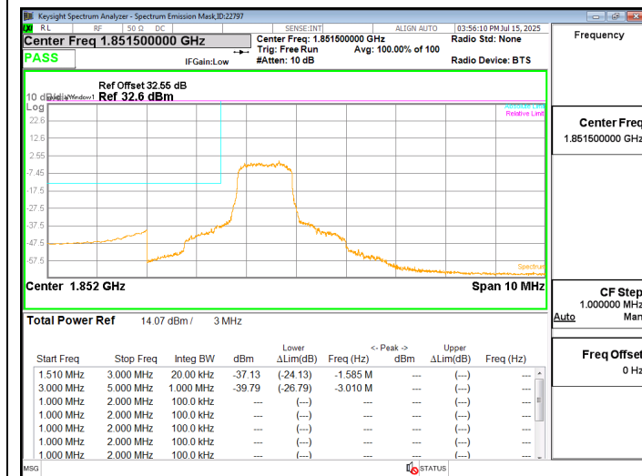
LTE2 3MHz QPSK LOW Ch RB6-0
