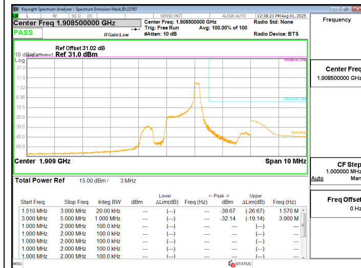
LTE2 3MHz QPSK HIGH Ch RB1-5
