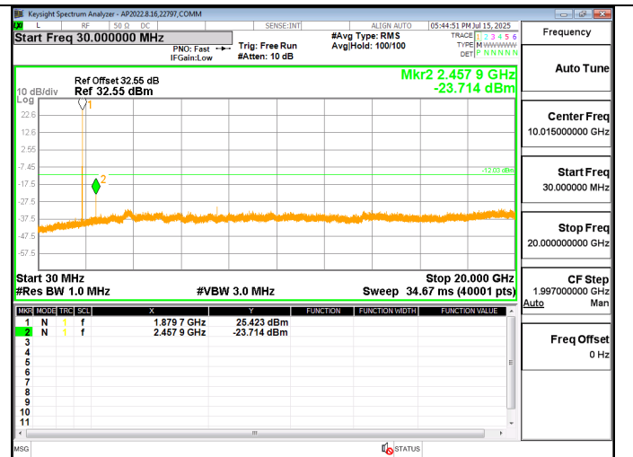
LTE2 1.4MHz QPSK MID Ch RB1-0
