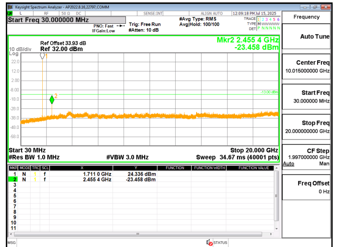
LTE4 3MHz QPSK LOW Ch RB1-0
