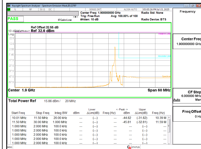
LTE2 20MHz QPSK HIGH Ch RB1-5
