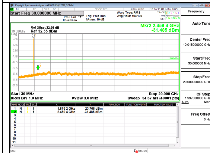
LTE2 10MHz QPSK MID Ch RB1-0
