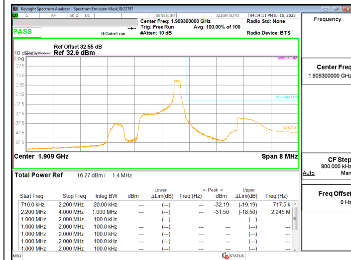
LTE2 1.4MHz QPSK HIGH Ch RB1-5
