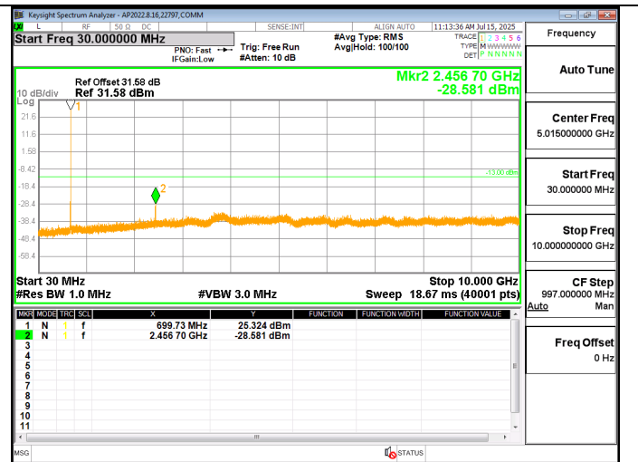
LTE12 3MHz QPSK LOW Ch RB1-0
