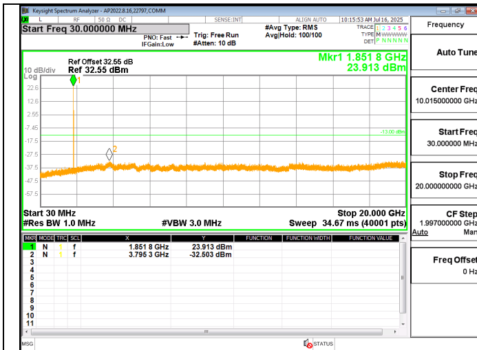
LTE2 1.4MHz QPSK LOW Ch RB1-0
