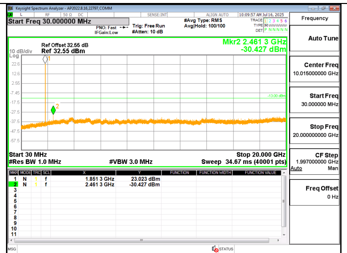
LTE2 10MHz QPSK LOW Ch RB1-0
