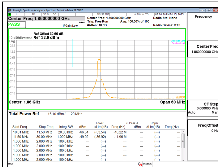
LTE2 20MHz QPSK LOW Ch RB1-0
