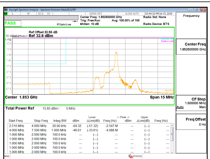
LTE2 5MHz QPSK LOW Ch RB1-5
