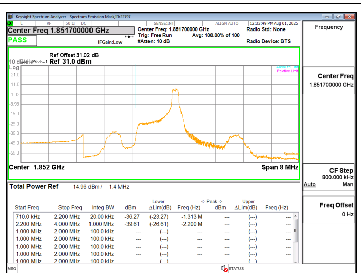
LTE2 1.4MHz QPSK LOW Ch RB1-5
