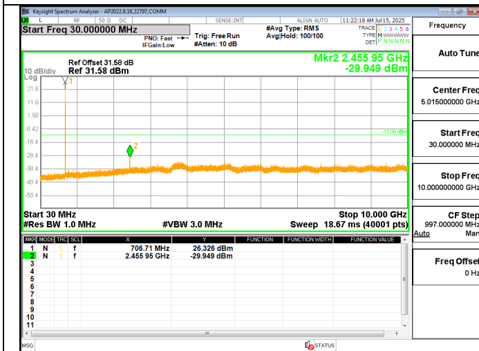
LTE12 3MHz QPSK MID Ch RB1-0
