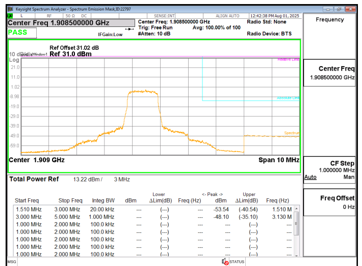
LTE2 3MHz QPSK HIGH Ch RB6-0
