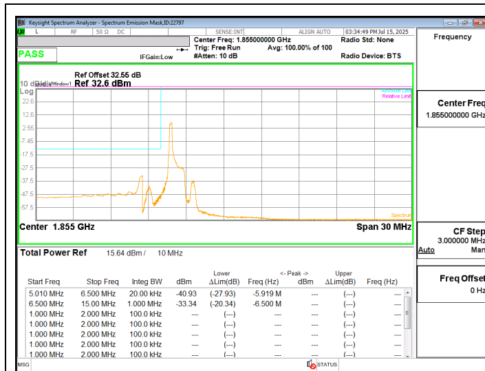
LTE2 10MHz QPSK LOW Ch RB1-0
