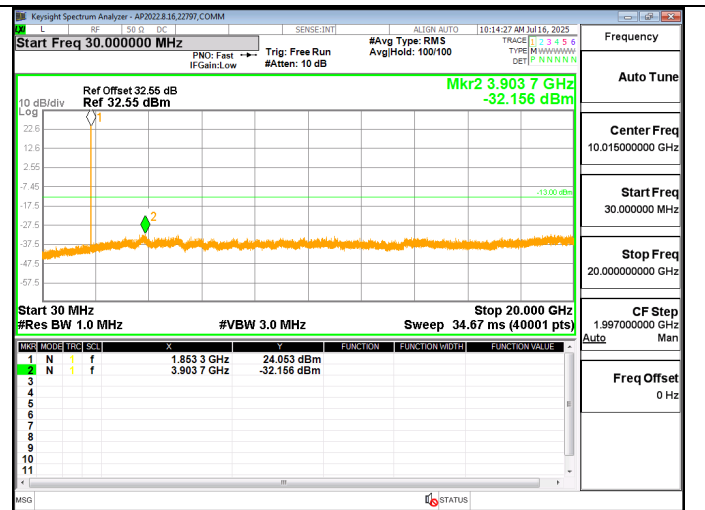
LTE2 3MHz QPSK LOW Ch RB1-0
