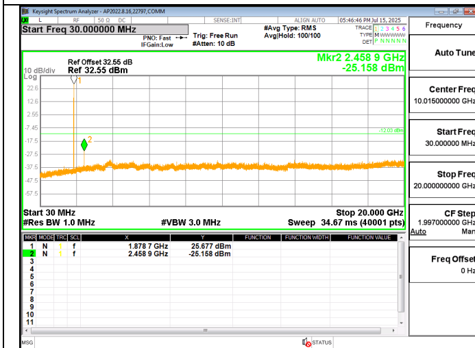
LTE2 3MHz QPSK MID Ch RB1-0
