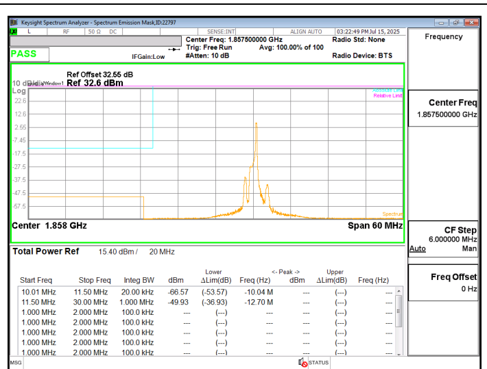
LTE2 15MHz QPSK LOW Ch RB1-5
