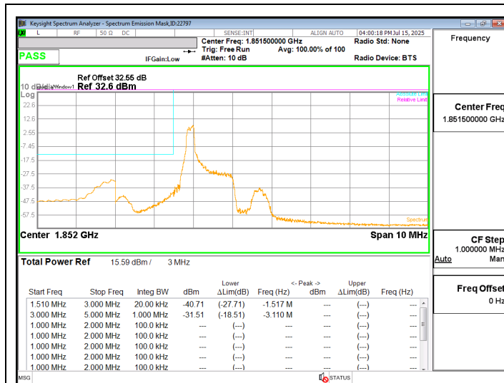
LTE2 3MHz QPSK LOW Ch RB1-0
