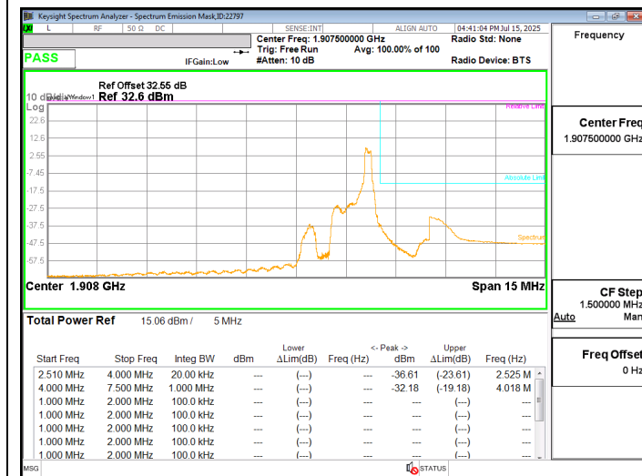
LTE2 5MHz QPSK HIGH Ch RB1-5
