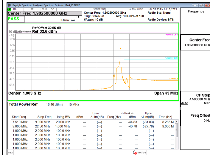
LTE2 15MHz QPSK HIGH Ch RB1-5
