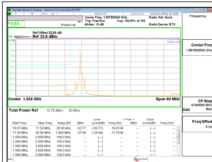
LTE2 15MHz QPSK LOW Ch RB1-0
