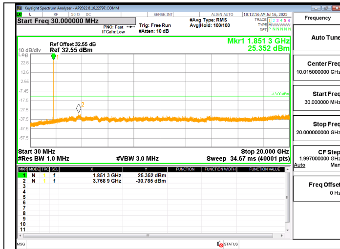
LTE2 5MHz QPSK LOW Ch RB1-0
