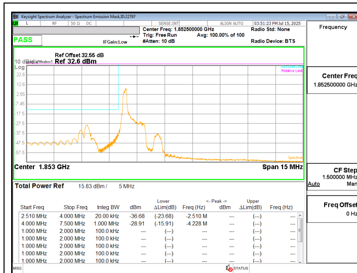
LTE2 5MHz QPSK LOW Ch RB1-0
