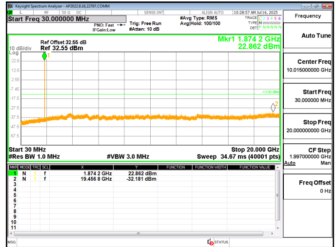
LTE2 15MHz QPSK MID Ch RB1-0
