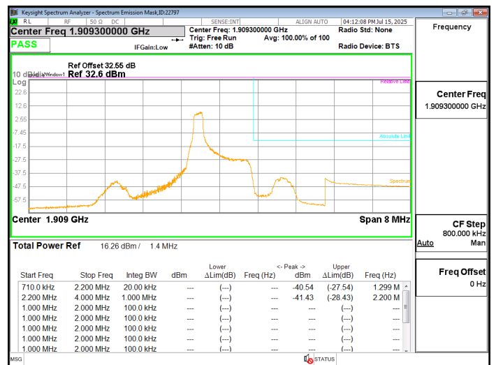
LTE2 1.4MHz QPSK HIGH Ch RB1-0
