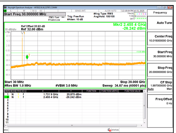
LTE4 1.4MHz QPSK MID Ch RB1-0
