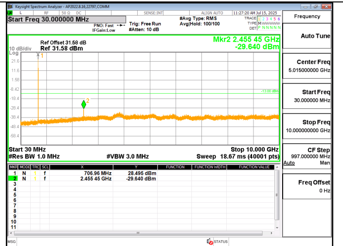
LTE12 1.4MHz QPSK MID Ch RB1-0
