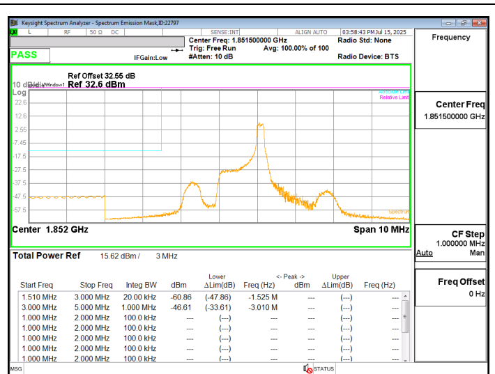
LTE2 3MHz QPSK LOW Ch RB1-5
