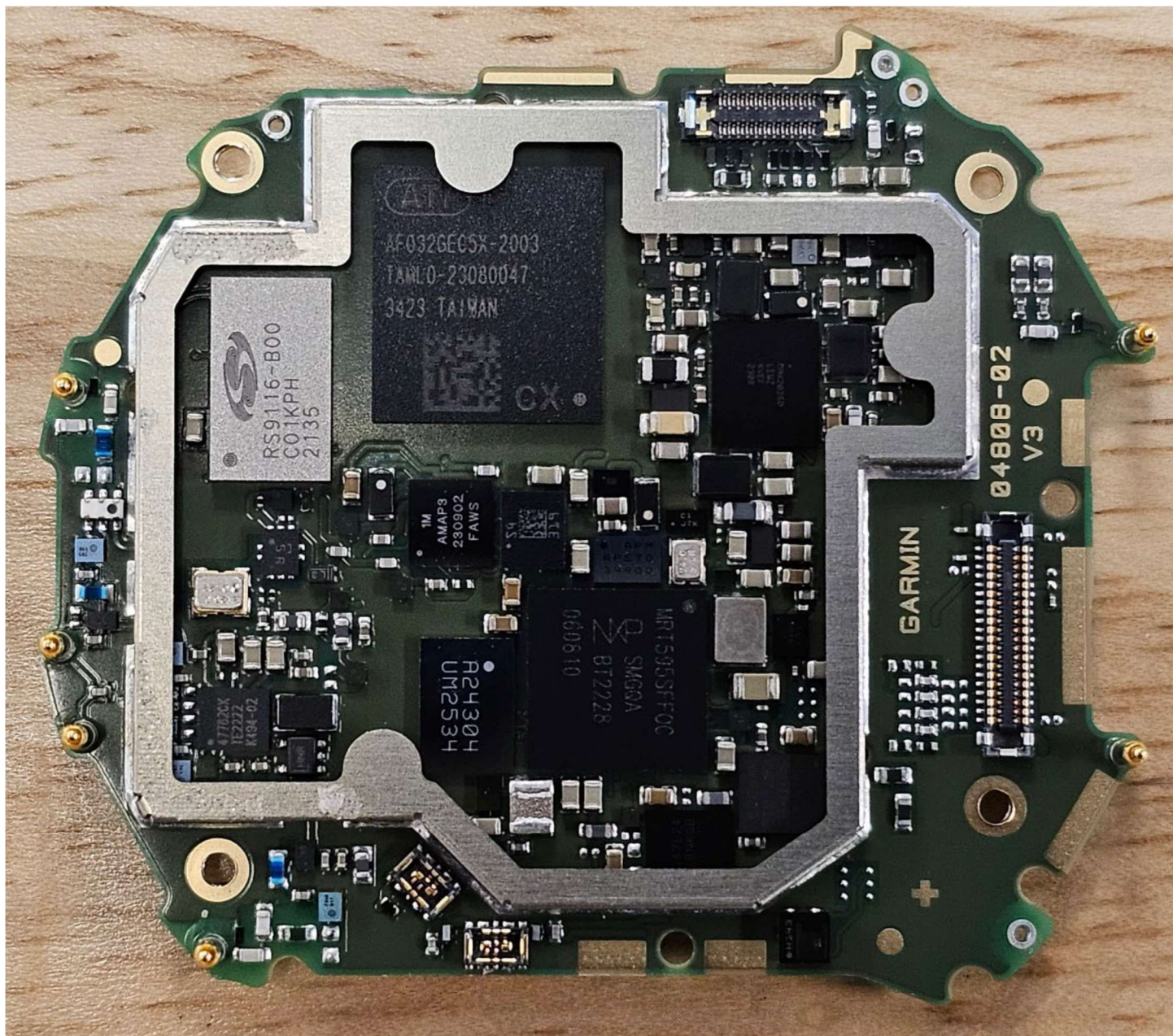
Figure E14.4 – Internal – DUT Split, Main PCB, Shield Removed
