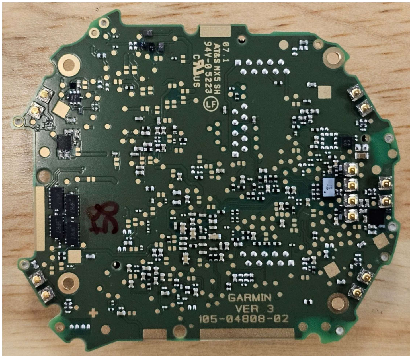
Figure E14.5 – Internal – DUT Split, Main PCB, Back Side
