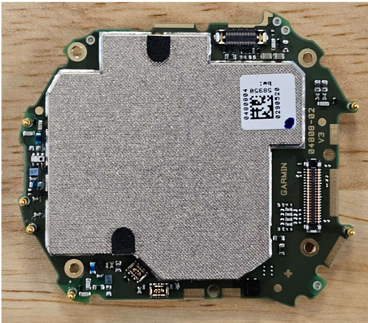
Figure E14.3 – Internal – DUT Split, Main PCB
