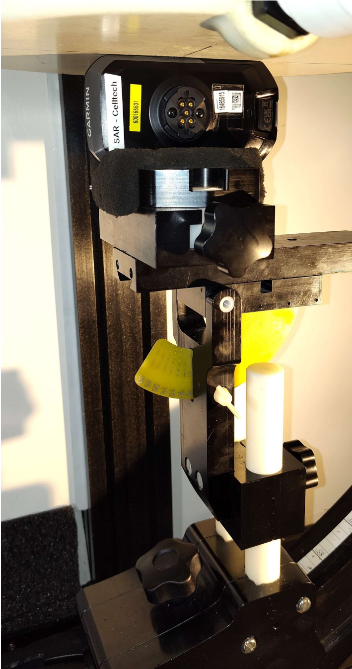
Figure C.4 – Setup Photo, Right Touch
