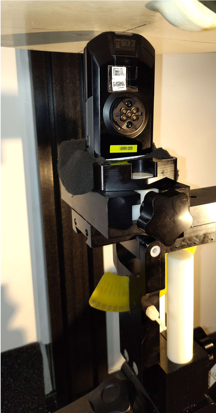
Figure C.6 – Setup Photo, Bottom Touch
