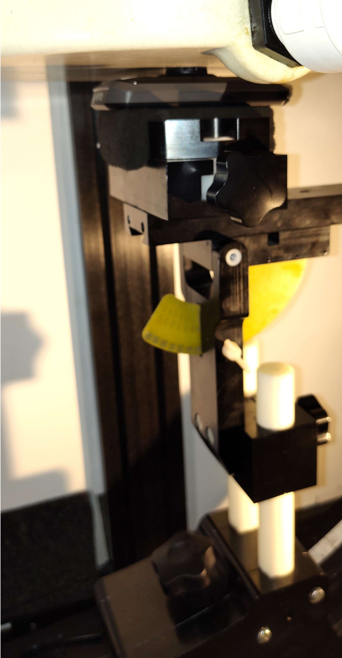
Figure C.1 – Setup Photo, Back Touch
