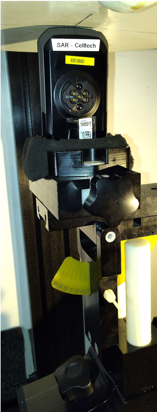
Figure C.5 – Setup Photo, Top Touch
