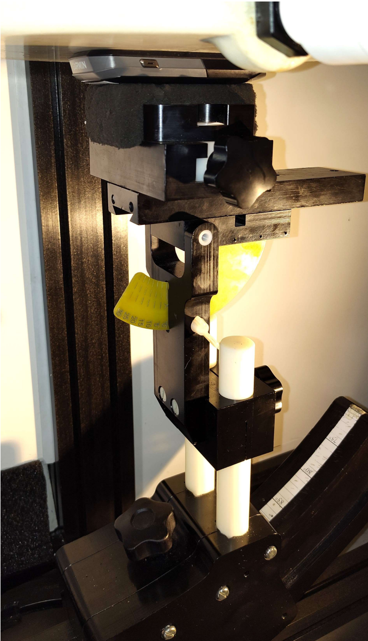
Figure C.2 – Setup Photo, Front Touch
