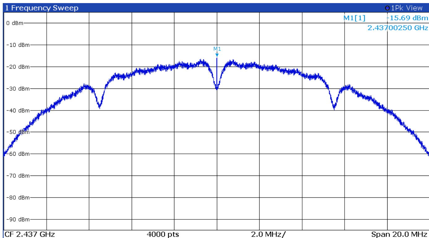
Figure 43 Plot of Transmitter Power Spectral Density Mode 5 802.11b
