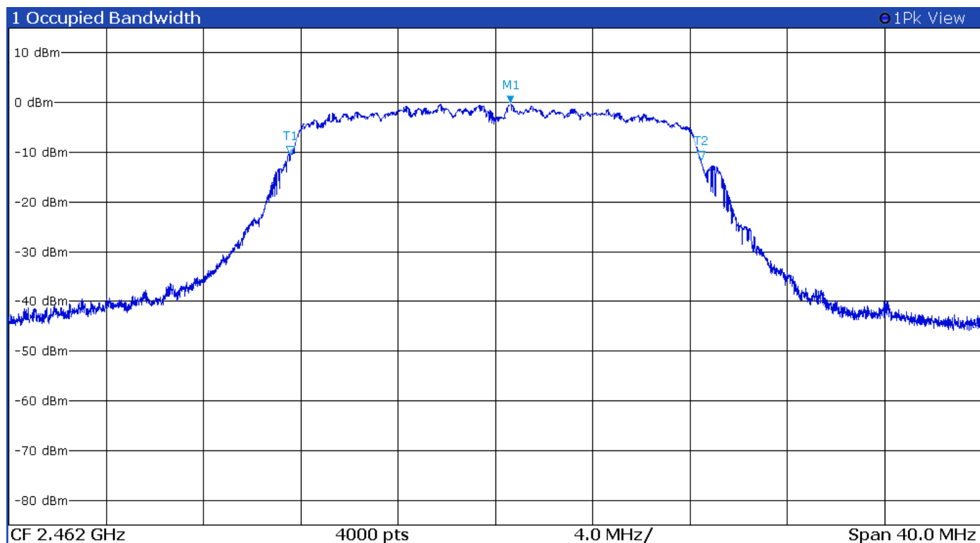
Figure 35 Plot of 99% Occupied Bandwidth Mode 6 802.11g
