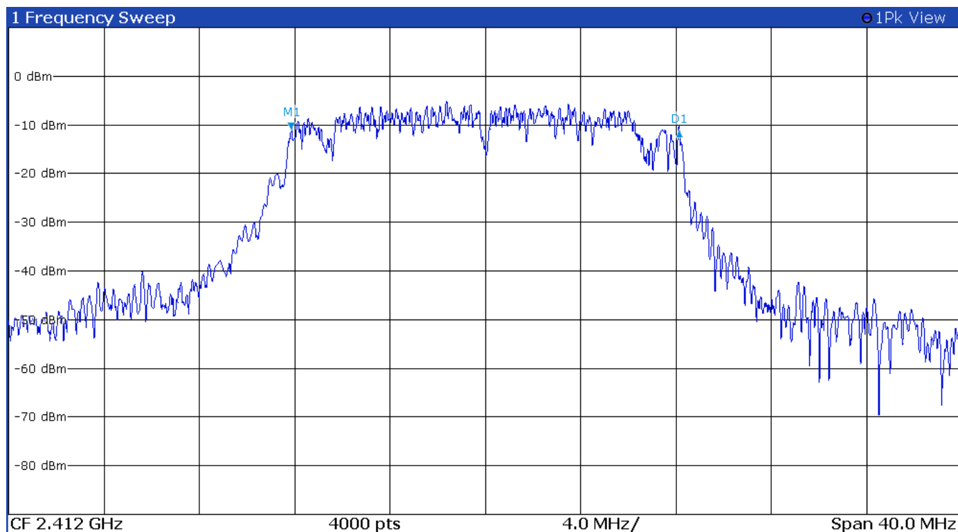
Figure 34 Plot of 6-dB Occupied Bandwidth Mode 6 802.11g
