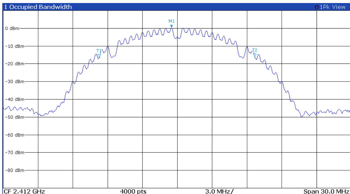
Figure 33 Plot of 99% Occupied Bandwidth Mode 5 802.11b
