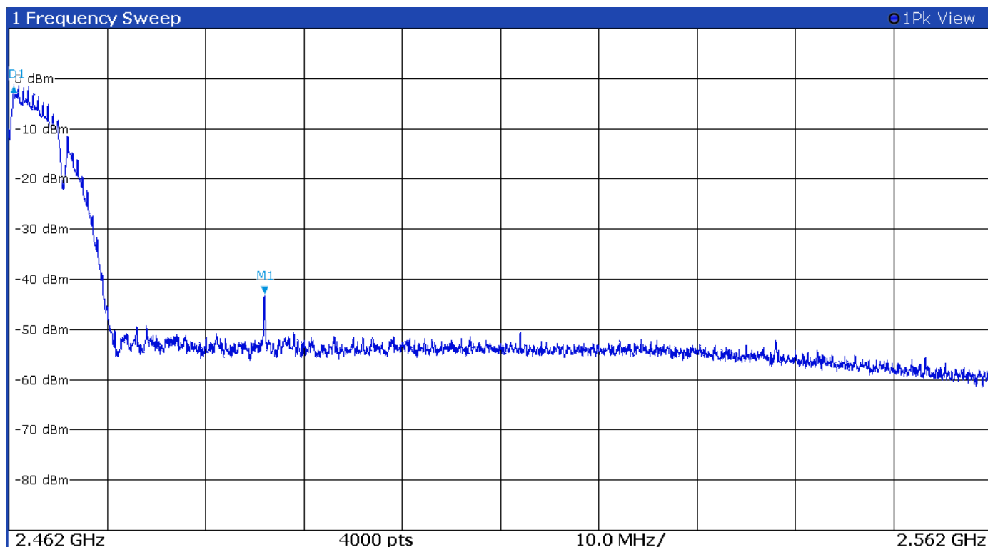
Figure 22 Plot of Transmitter Emissions High Band Edge Mode 5 802.11b
