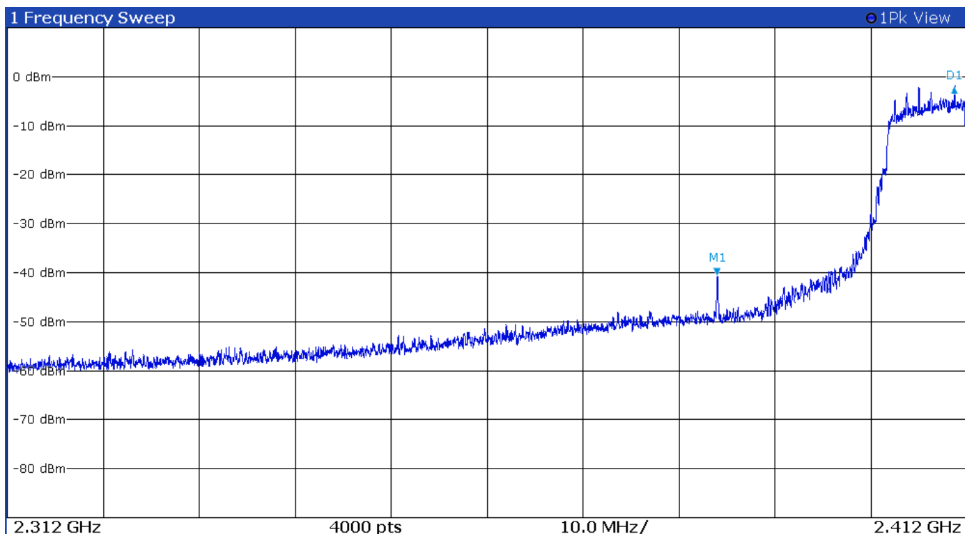
Figure 16 Plot of Transmitter Emissions Low Band Edge Mode 6 802.11g
