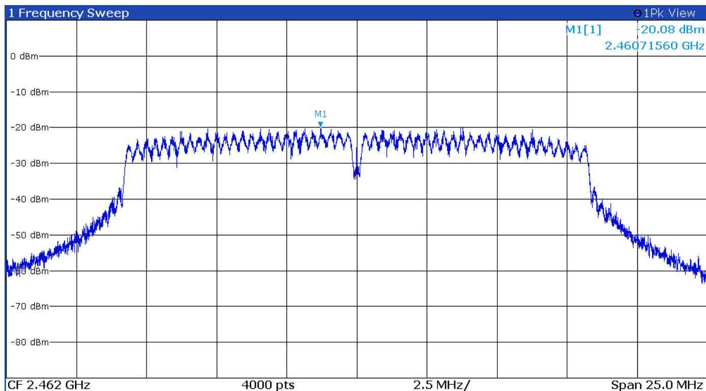
Figure 44 Plot of Transmitter Power Spectral Density Mode 6 802.11g
