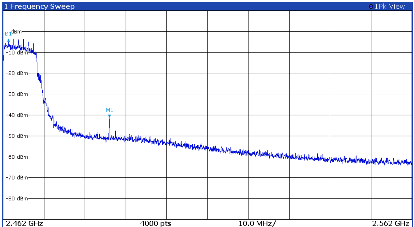
Figure 23 Plot of Transmitter Emissions High Band Edge Mode 6 802.11g
