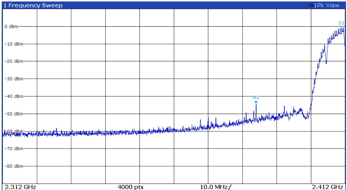
Figure 15 Plot of Transmitter Emissions Low Band Edge Mode 5 802.11b
