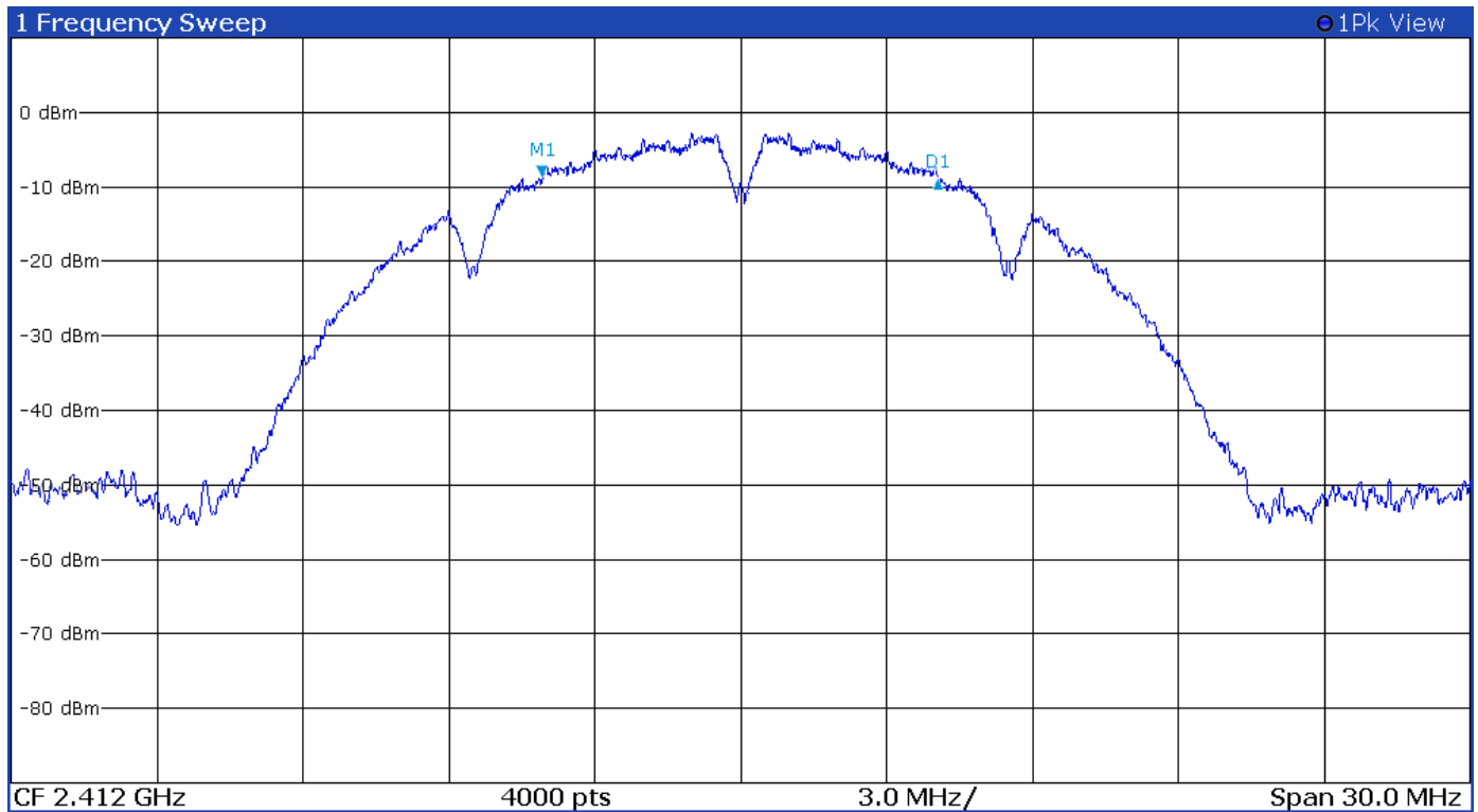
Figure 32 Plot of 6-dB Occupied Bandwidth Mode 5 802.11b
