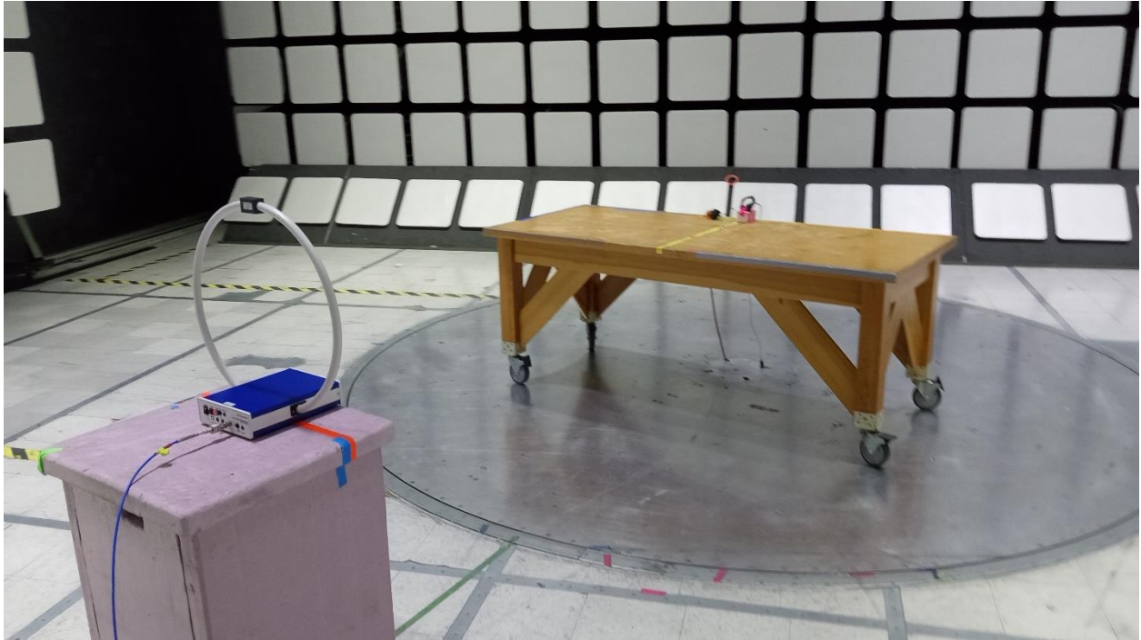
150kHz – 30 MHz Test Setup
