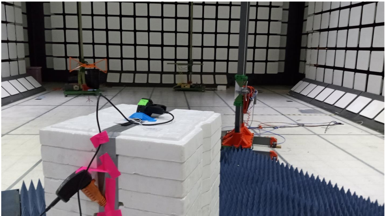
1 – 26 GHz Test Setup
