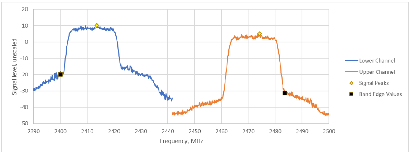
Figure TR36.12: Spectral data for IEEE 802.11 n MCS1 Mbps at 20 °C and 5.75 Vdc which represent Ch1 and Ch13
