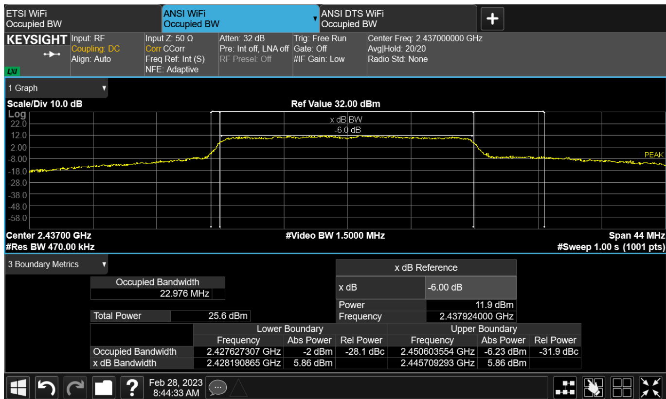
Figure TR15.6: Occupied bandwidth data for 802.11n MCS1 at channel 6
