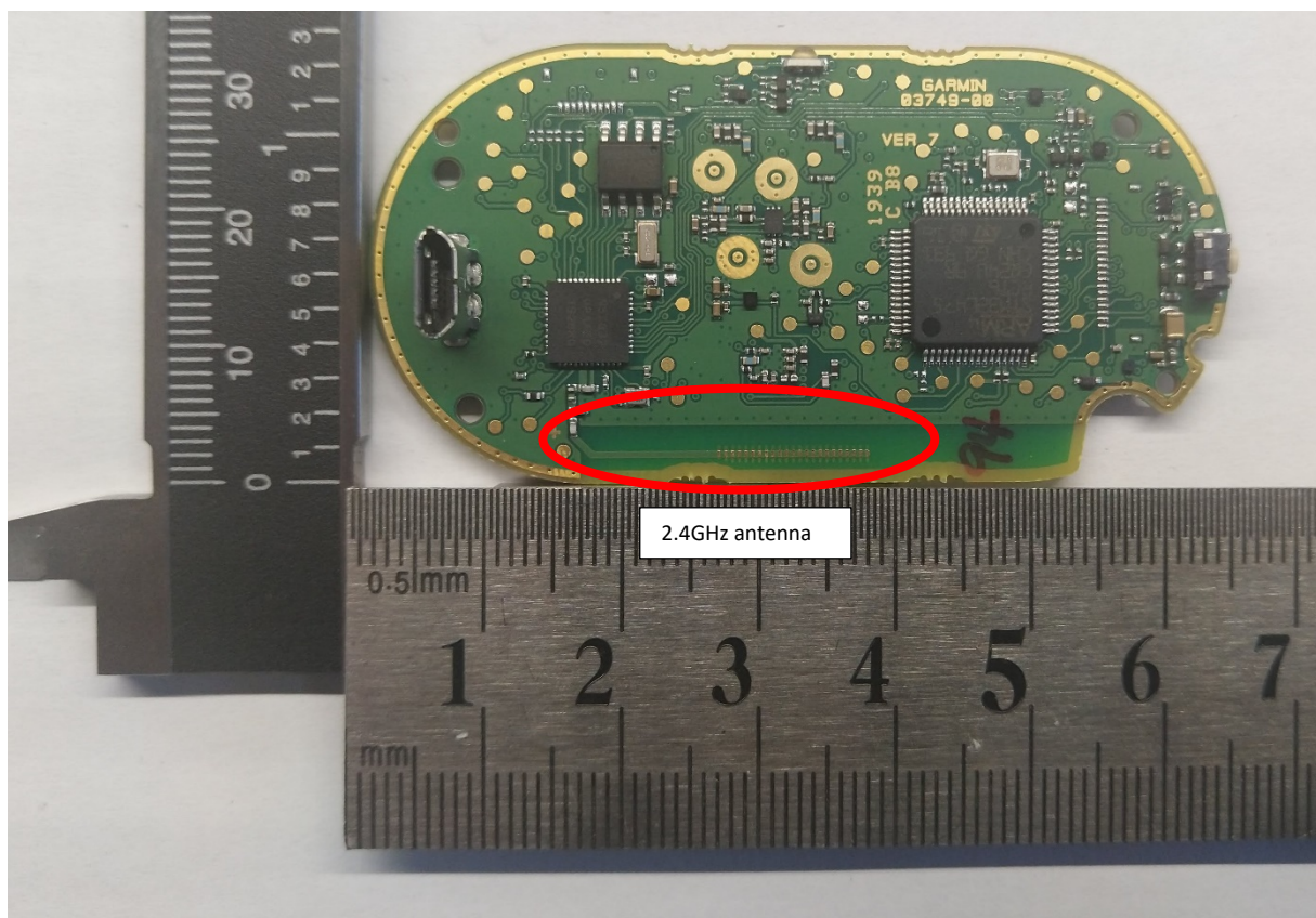
Figure 5 - PCB Rear
