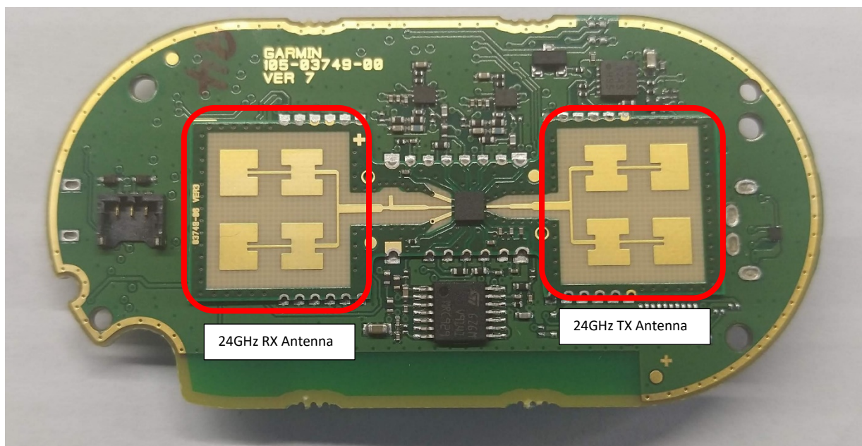
Figure 6 - PCB Front
