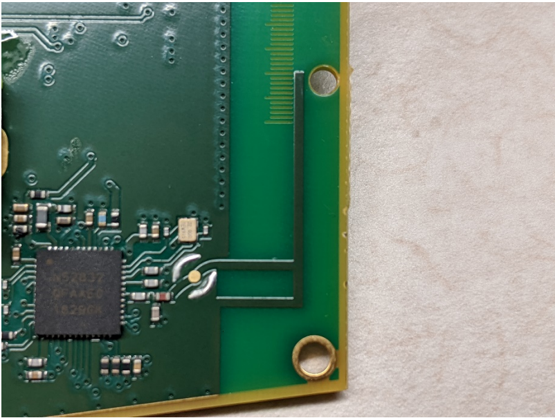
Figure 4 - Antenna
